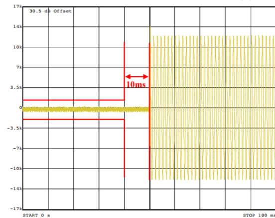
Transmitter Frequency Behavior @ 12.5 KHz Channel Separation-----On – Off
