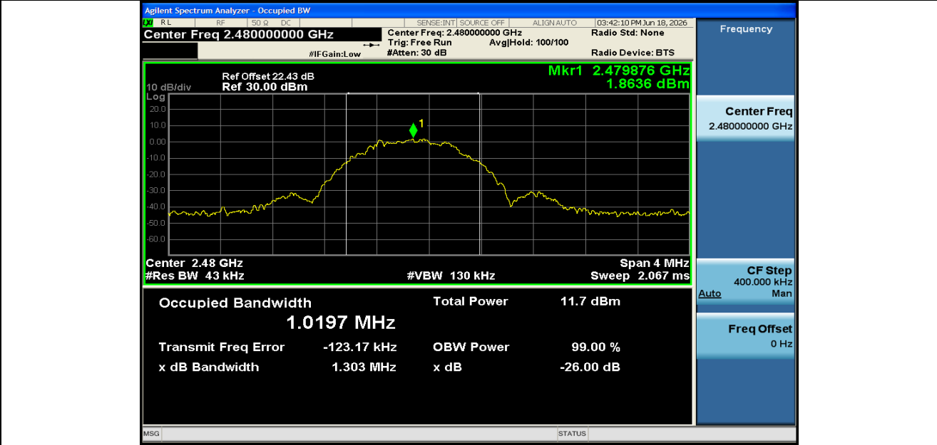
BLE_1M-Ant1-2480
