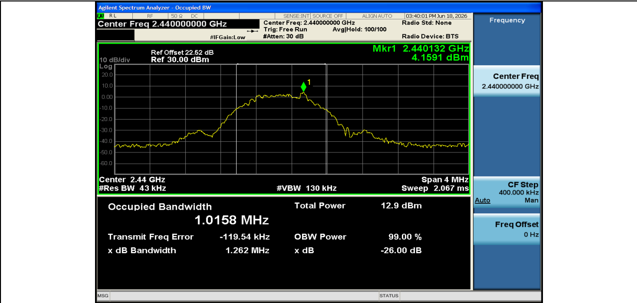
BLE_1M-Ant1-2440
