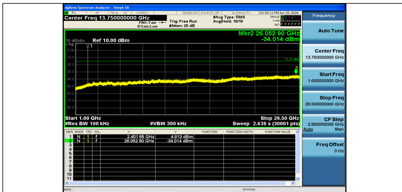
BLE_1M-Ant1-2402-1000~26500-PASS
