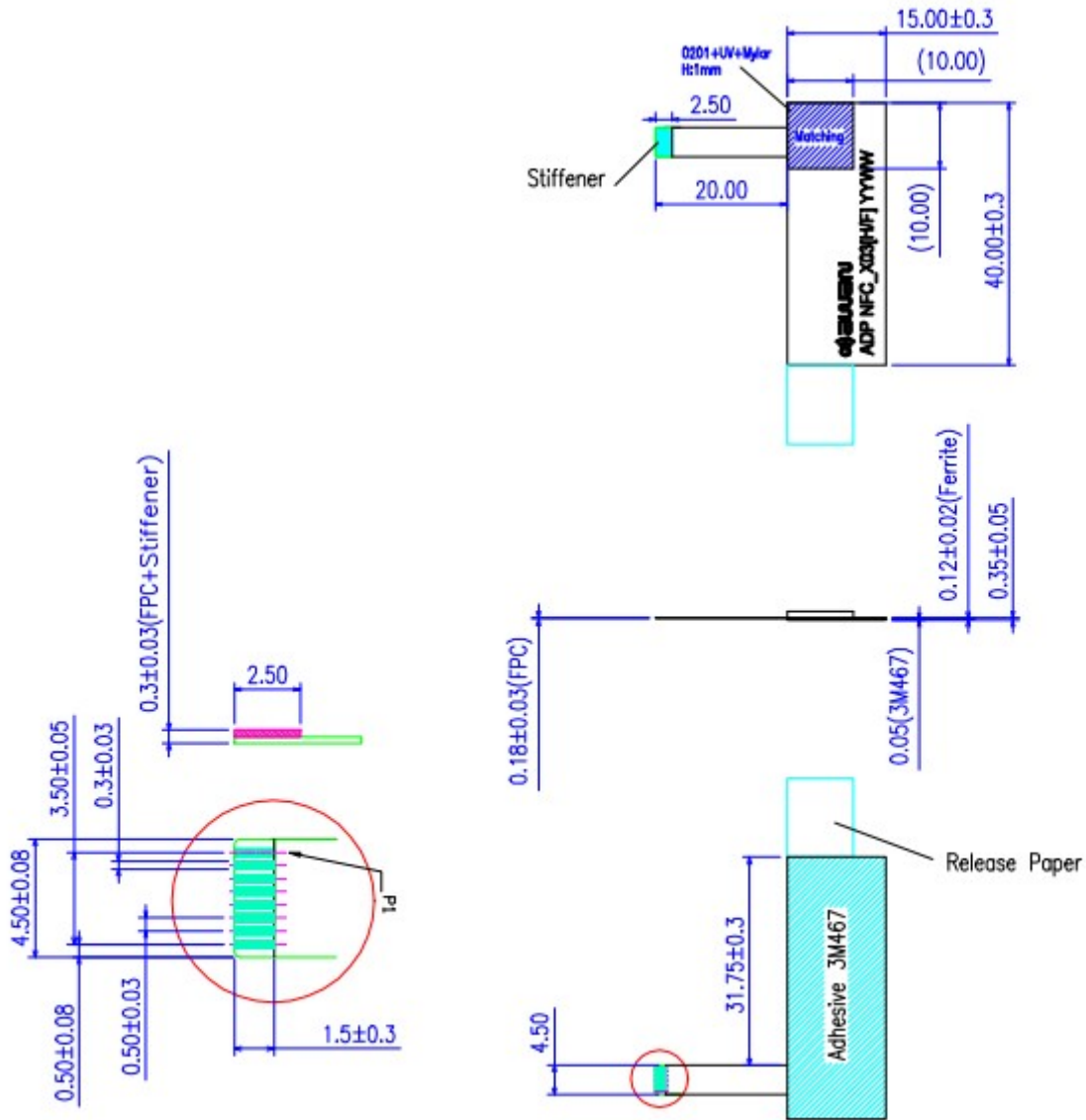
8 Pin Connector
