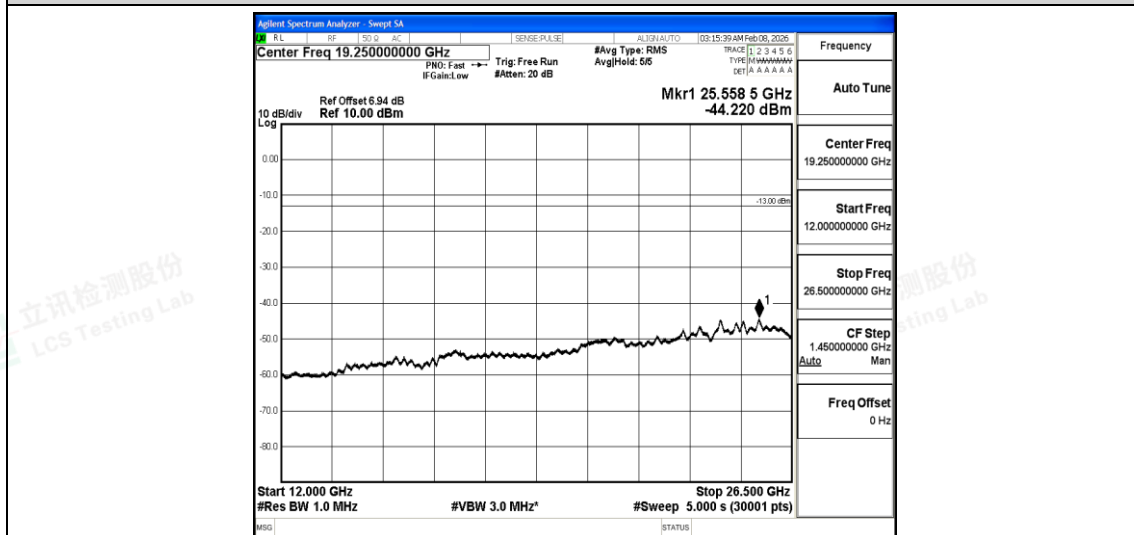
Band5-Stand-Alone-NaN-BPSK-20401-1@11-15kHz-12000-26500-12000~26500MHz@-44.22dBm--13-PASS
