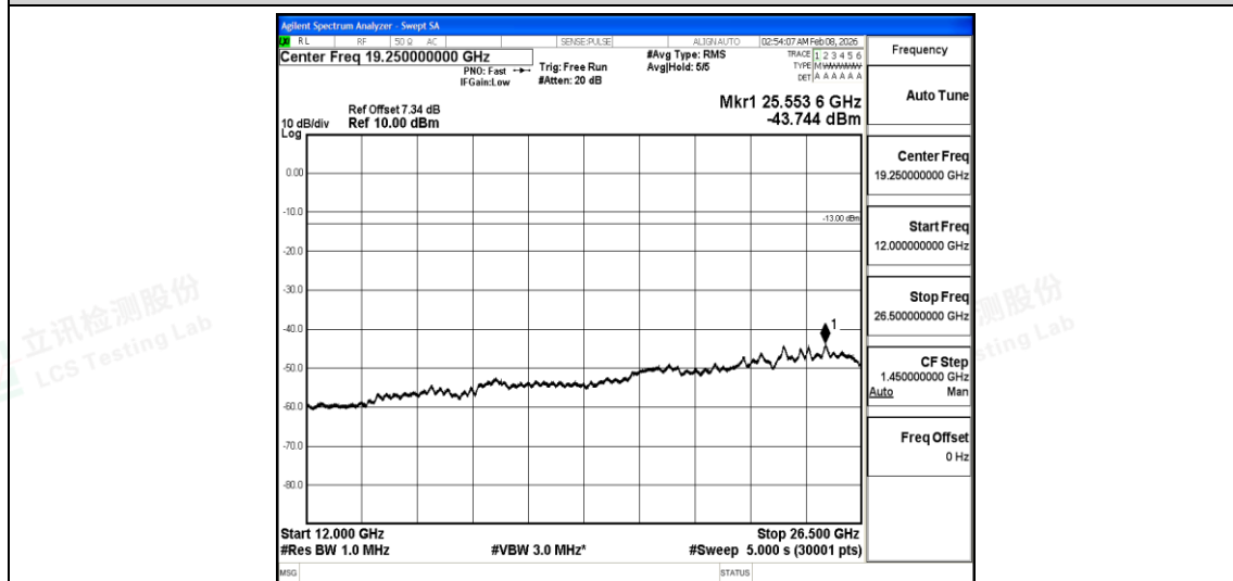
Band5-Stand-Alone-NaN-QPSK-20649-1@0-3.75kHz-12000-26500-12000~26500MHz@-43. 74dBm--13-PASS
