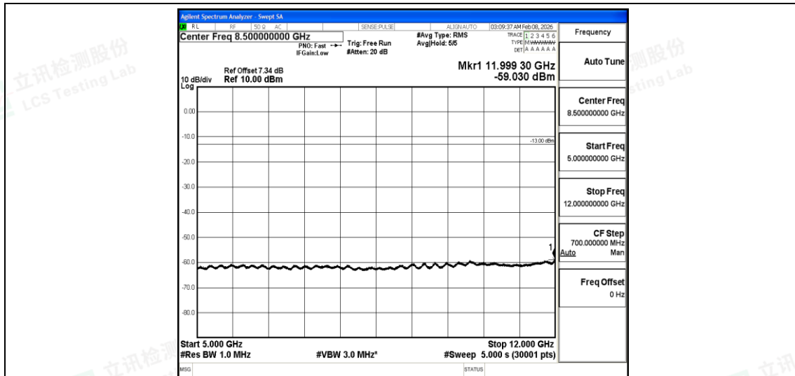
Band5-Stand-Alone-NaN-QPSK-20649-12@0-15kHz-5000-12000-5000~12000MHz@-59.03dBm--13-PASS
