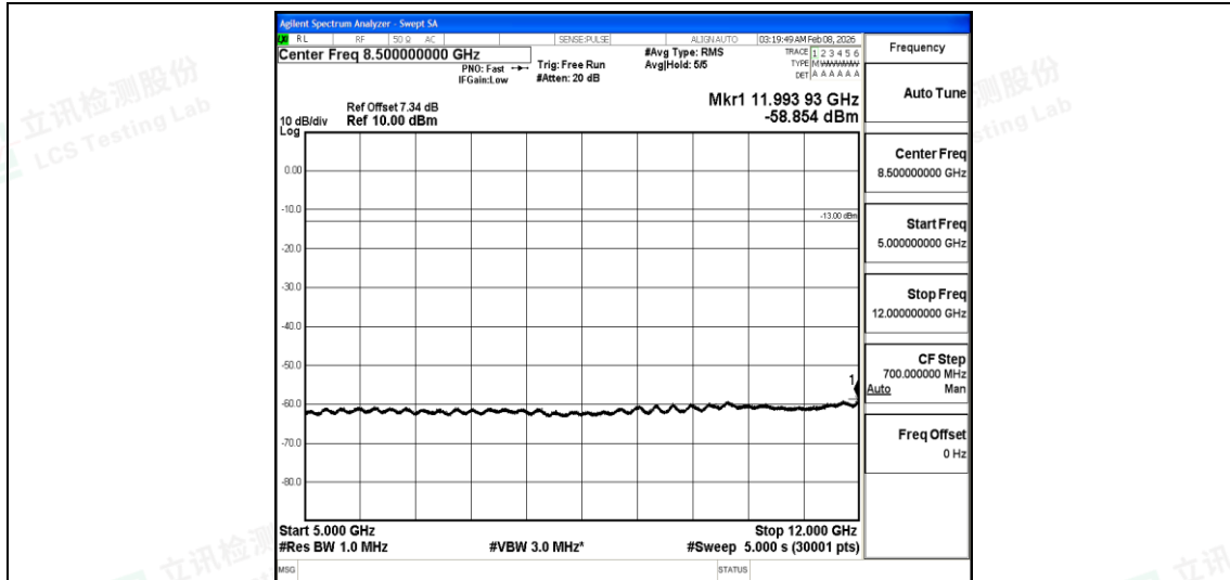
Band5-Stand-Alone-NaN-BPSK-20525-1@11-15kHz-5000-12000-5000~12000MHz@-58.85dBm--13-PASS
