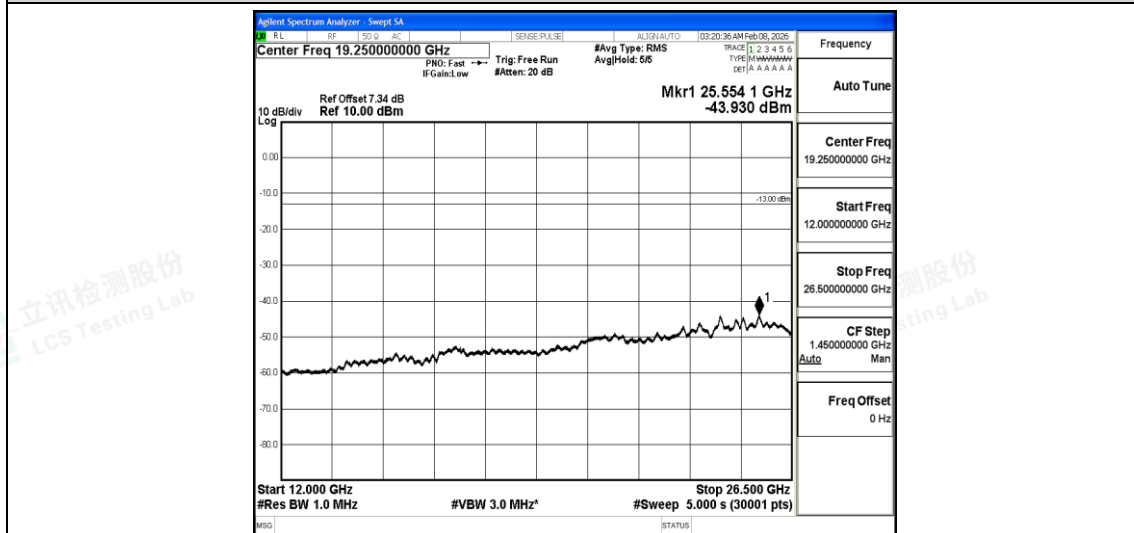
Band5-Stand-Alone-NaN-BPSK-20525-1@11-15kHz-12000-26500-12000~26500MHz@-43.93dBm--13-PASS
