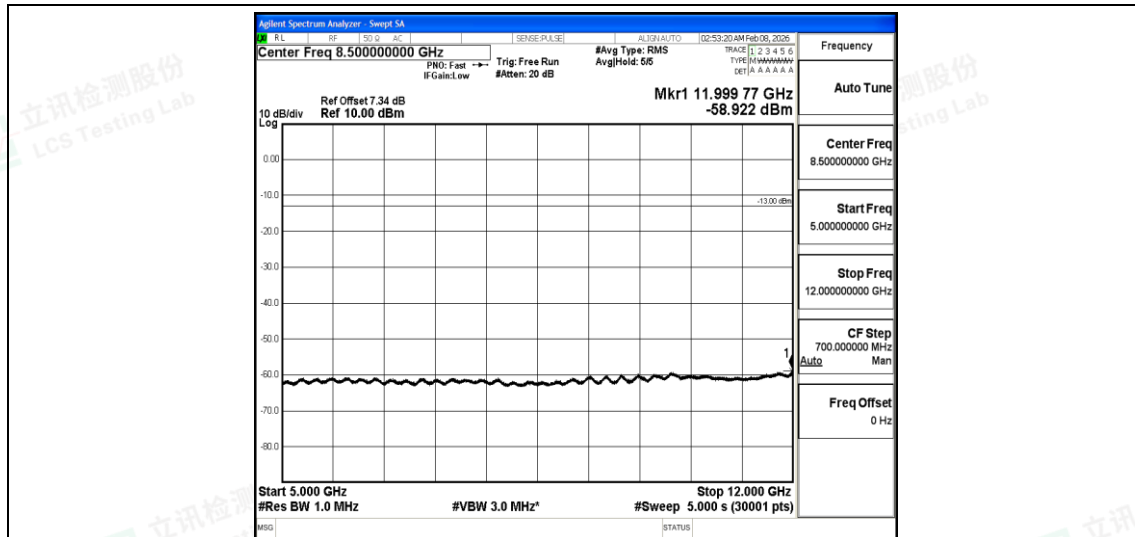
Band5-Stand-Alone-NaN-QPSK-20649-1@0-3.75kHz-5000-12000-5000~12000MHz@-58.92 dBm--13-PASS
