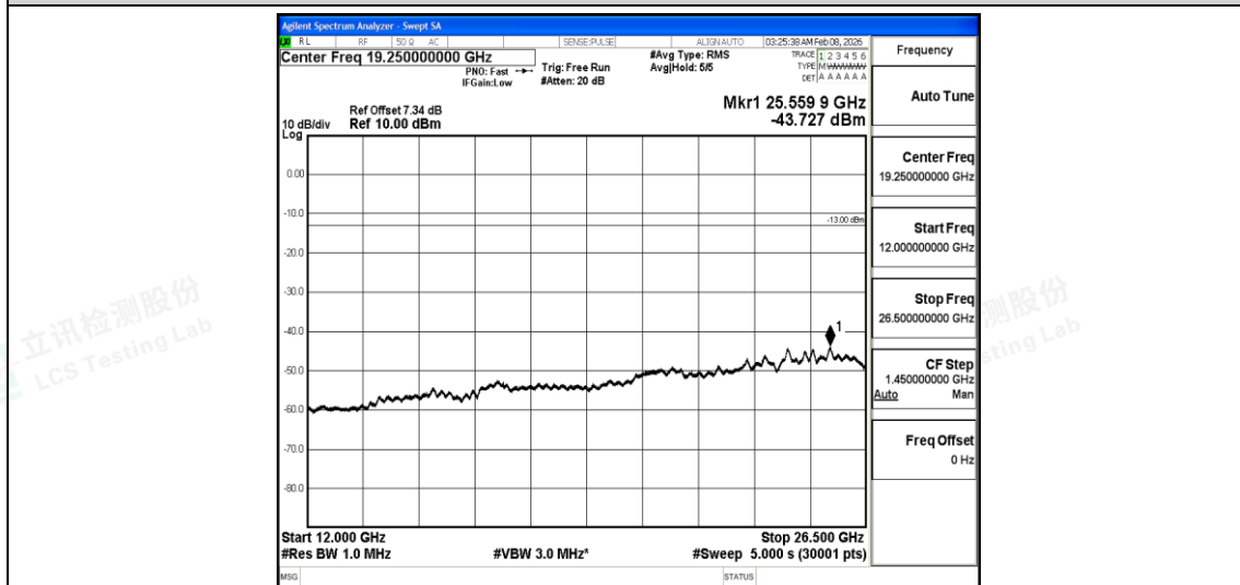
Band5-Stand-Alone-NaN-BPSK-20649-1@11-15kHz-12000-26500-12000~26500MHz@-43.73dBm--13-PASS
