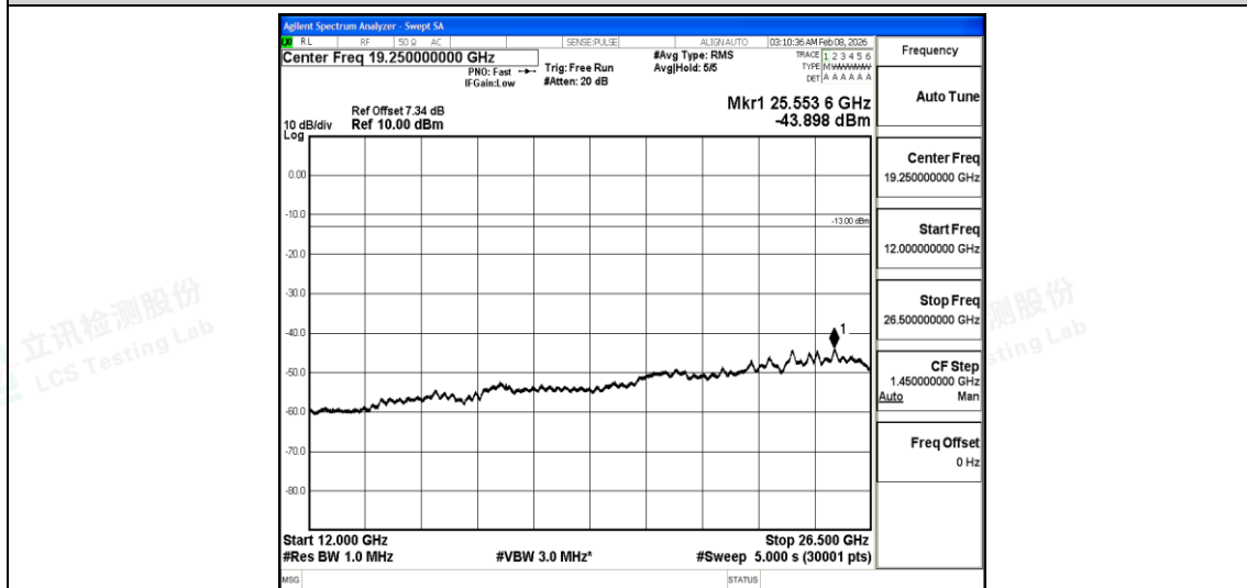
Band5-Stand-Alone-NaN-QPSK-20649-12@0-15kHz-12000-26500-12000~26500MHz@-43.9dBm--13-PASS
