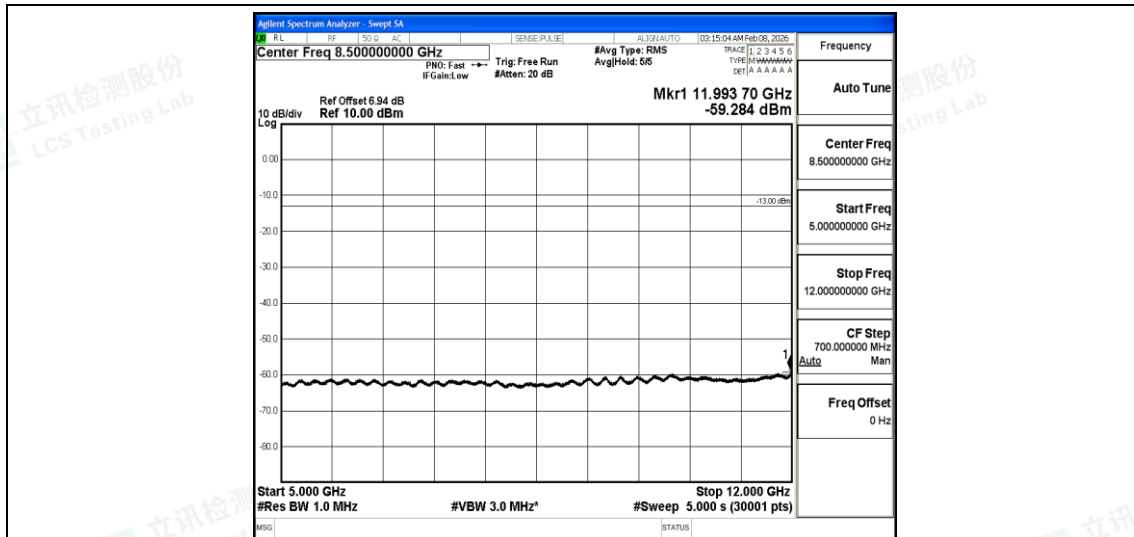
Band5-Stand-Alone-NaN-BPSK-20401-1@11-15kHz-5000-12000-5000~12000MHz@-59.28dBm--13-PASS
