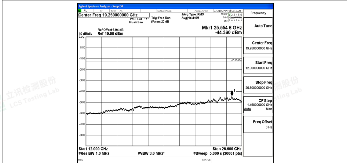
Band13-Stand-Alone-NaN-BPSK-23181-1@0-15kHz-12000-26500-12000~26500MHz@-44.3 6dBm--13-PASS
