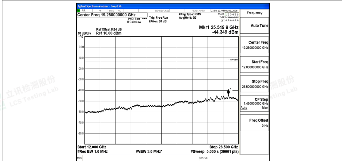
Band13-Stand-Alone-NaN-BPSK-23279-1@11-15kHz-12000-26500-12000~26500MHz@-44.35dBm--13-PASS
