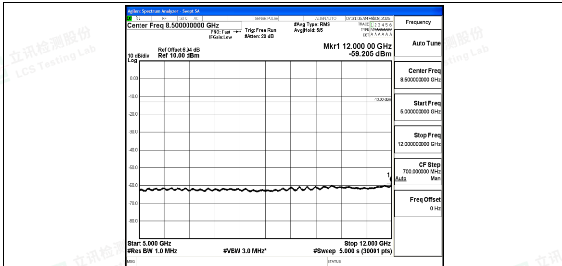
Band13-Stand-Alone-NaN-BPSK-23181-1@0-15kHz-5000-12000-5000~12000MHz@-59.21d Bm--13-PASS
