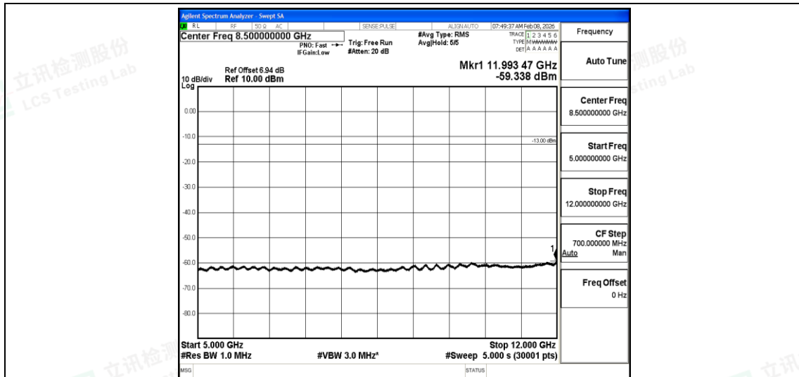
Band13-Stand-Alone-NaN-BPSK-23279-1@11-15kHz-5000-12000-5000~12000MHz@-59.34 dBm--13-PASS
