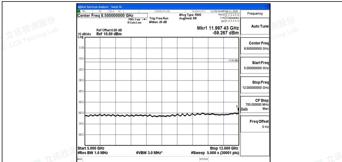
Band17-Stand-Alone-Na-N-BPSK-23790-1@0-15kHz-5000-12000-5000~12000MHz@-59.27d Bm--13-PASS
