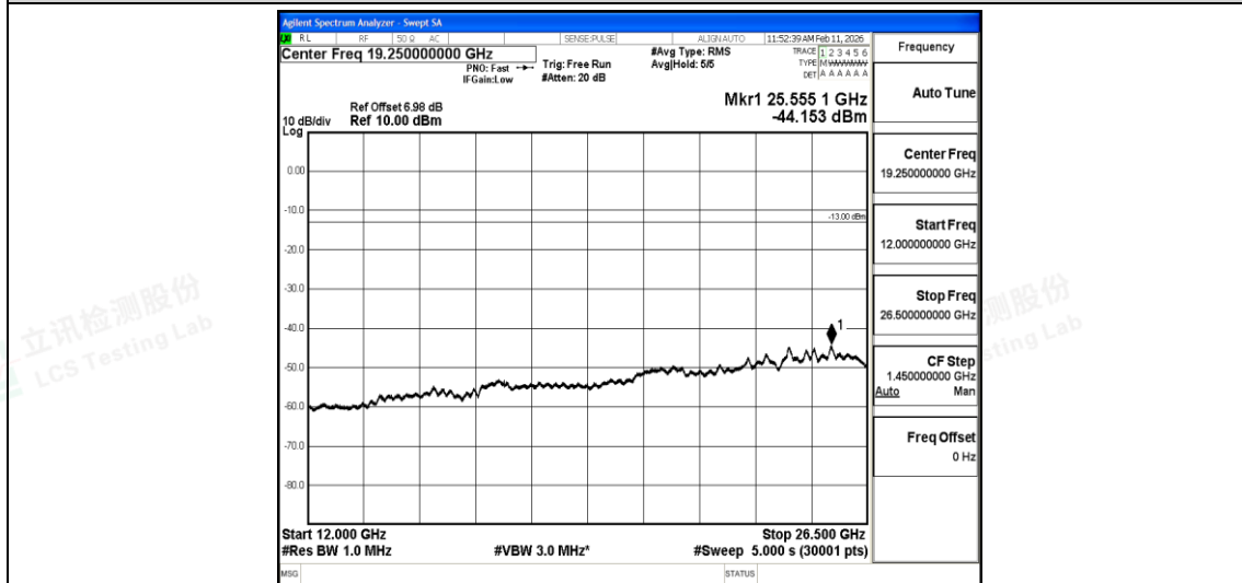
Band17-Stand-Alone-Na-N-BPSK-23790-1@0-15kHz-12000-26500-12000~26500MHz@-44.1 5dBm--13-PASS
