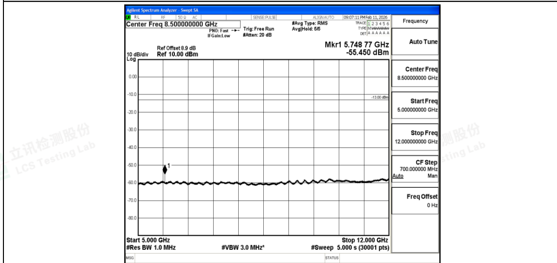
Band25-Stand-Alone-NaN-BPSK-26689-1@11-15kHz-5000-12000-5000~12000MHz@-55.45 dBm--13-PASS
