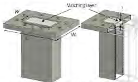
Figure 1: Validation Waveguide Dimensions
