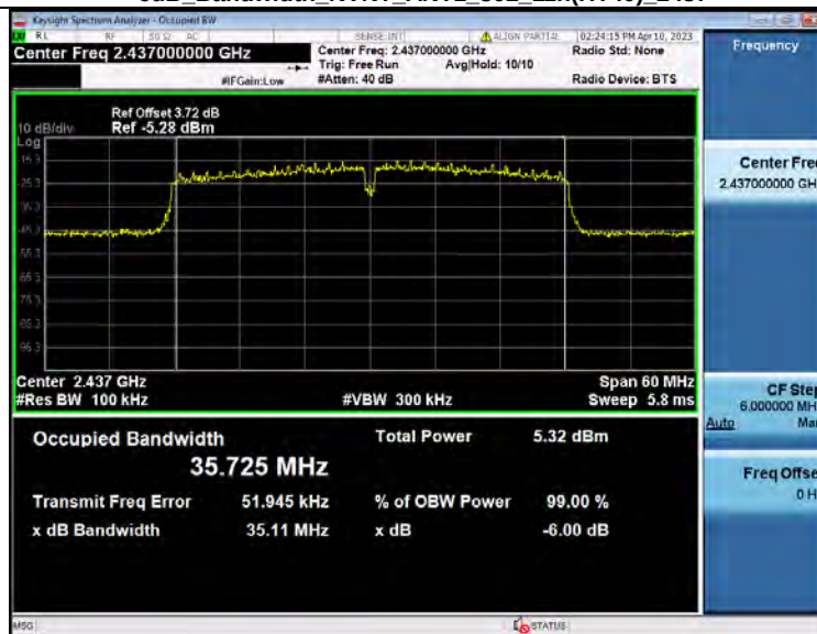
-6dB_Bandwidth_NVNT_ANT1_802_11n(HT40)_2437
