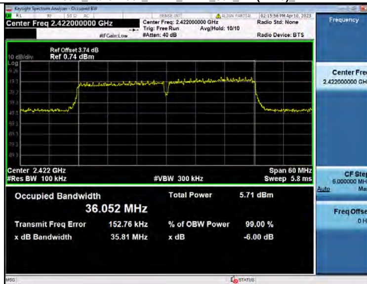
-6dB_Bandwidth_NVNT_ANT1_802_11n(HT40)_2422
