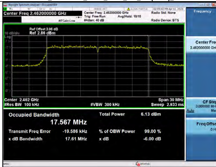
-6dB_Bandwidth_NVNT_ANT1_802_11n(HT20)_2462
