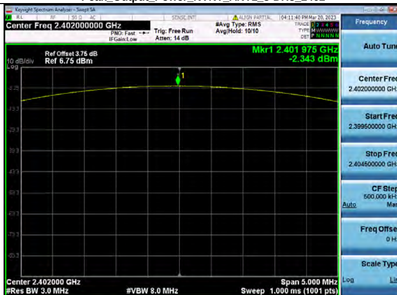
Peak_Output_Power_NVNT_ANT1_3-DH5_2402
