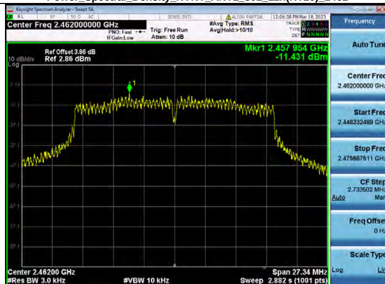
Power Spectral Density NVNT_ANT1_802_11n(HT20)_2462
