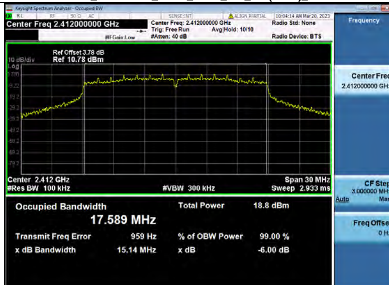
-6dB_Bandwidth_NVNT ANT2_802_11n(HT20)_2412
