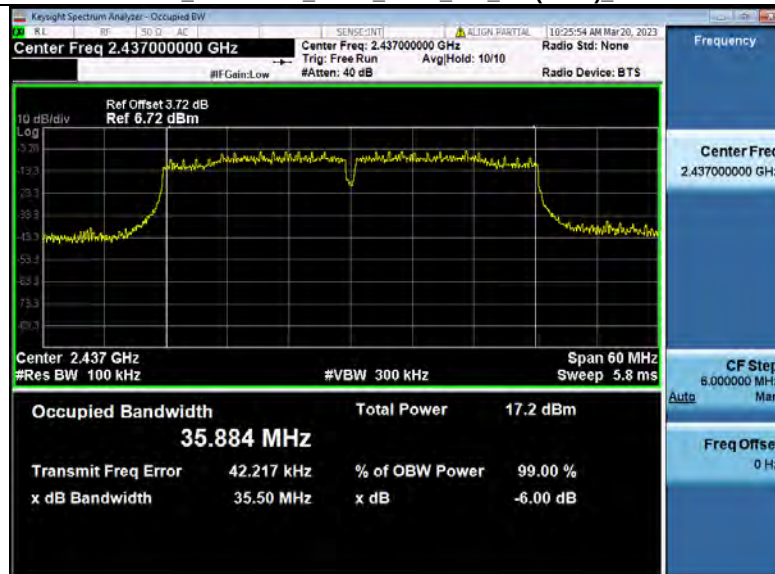
-6dB_Bandwidth_NVNT_ANT2_802_11n(HT40)_2437
