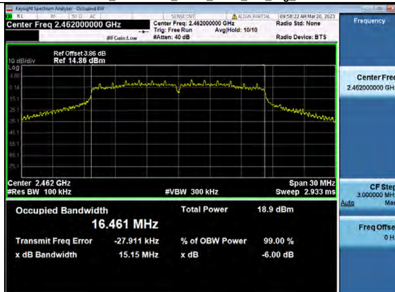
-6dB_Bandwidth_NVNT ANT2_802_11g_2462
