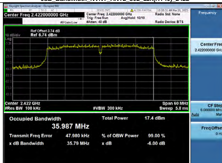
-6dB_Bandwidth_NVNT_ANT2_802_11n(HT40)_2422
