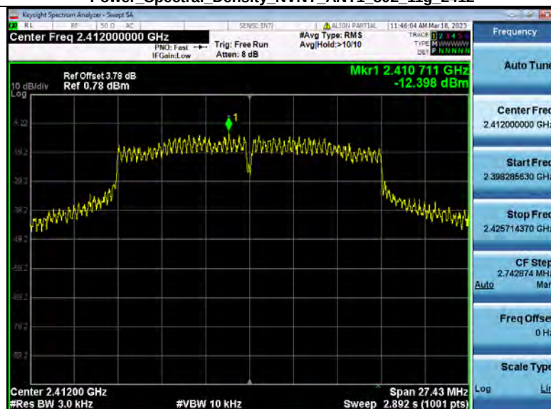
Power Spectral Density NVNT_ANT1_802_11g_2412
