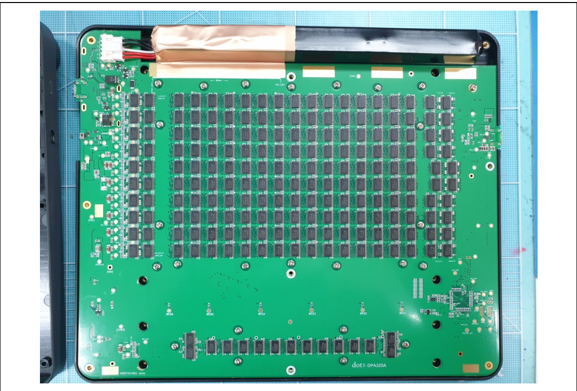
Main Board Rear
