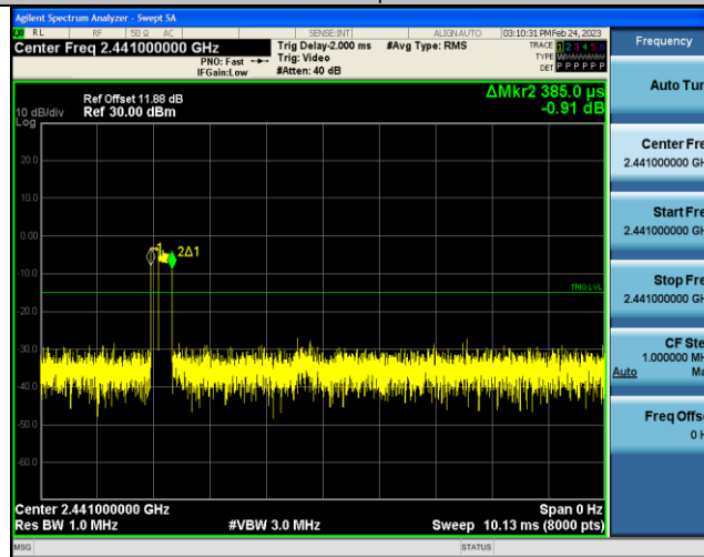
3DH3-Ant1-Hop-1.635-160
