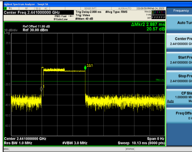
3DH1-Ant1-Hop-0.385-320
