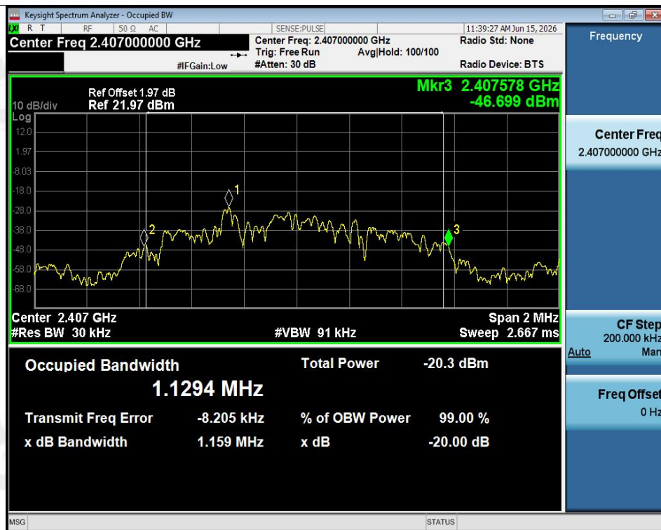
-20dB Bandwidth-GFSK 2407MHz
