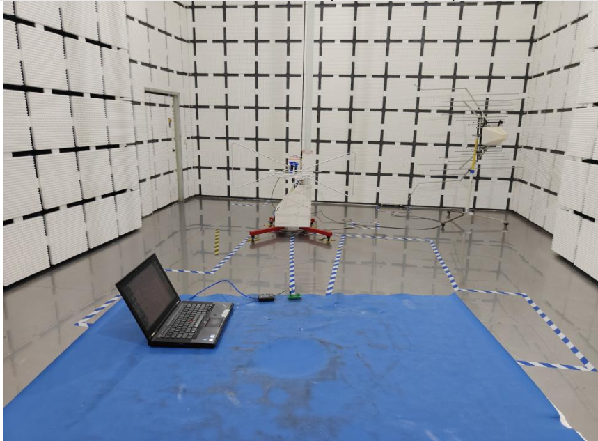
Radiated Emissions (30MHz-1GHz)
