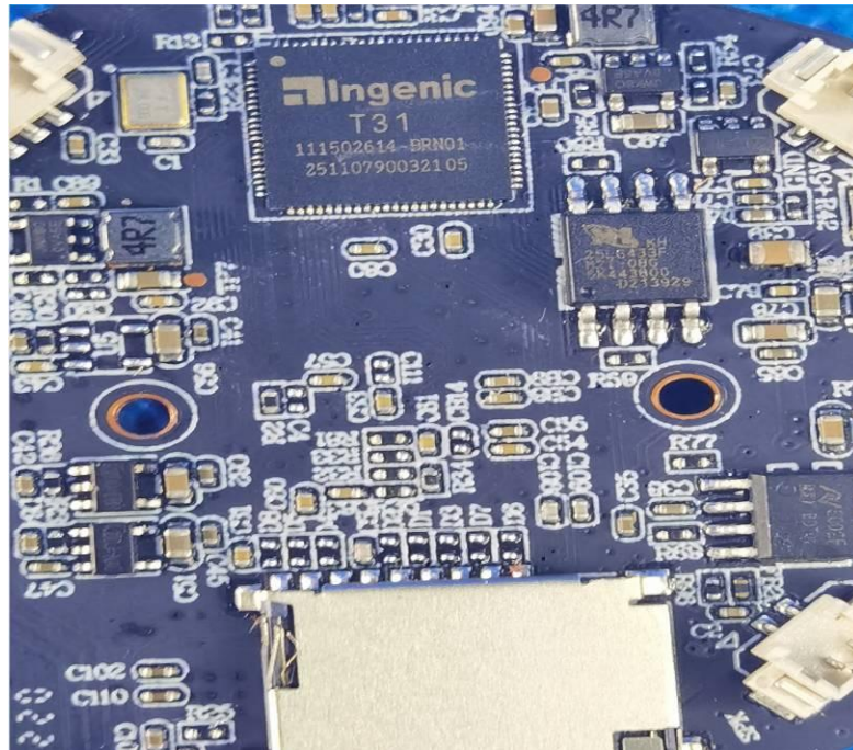
INTERNAL VIEW OF Adapter
