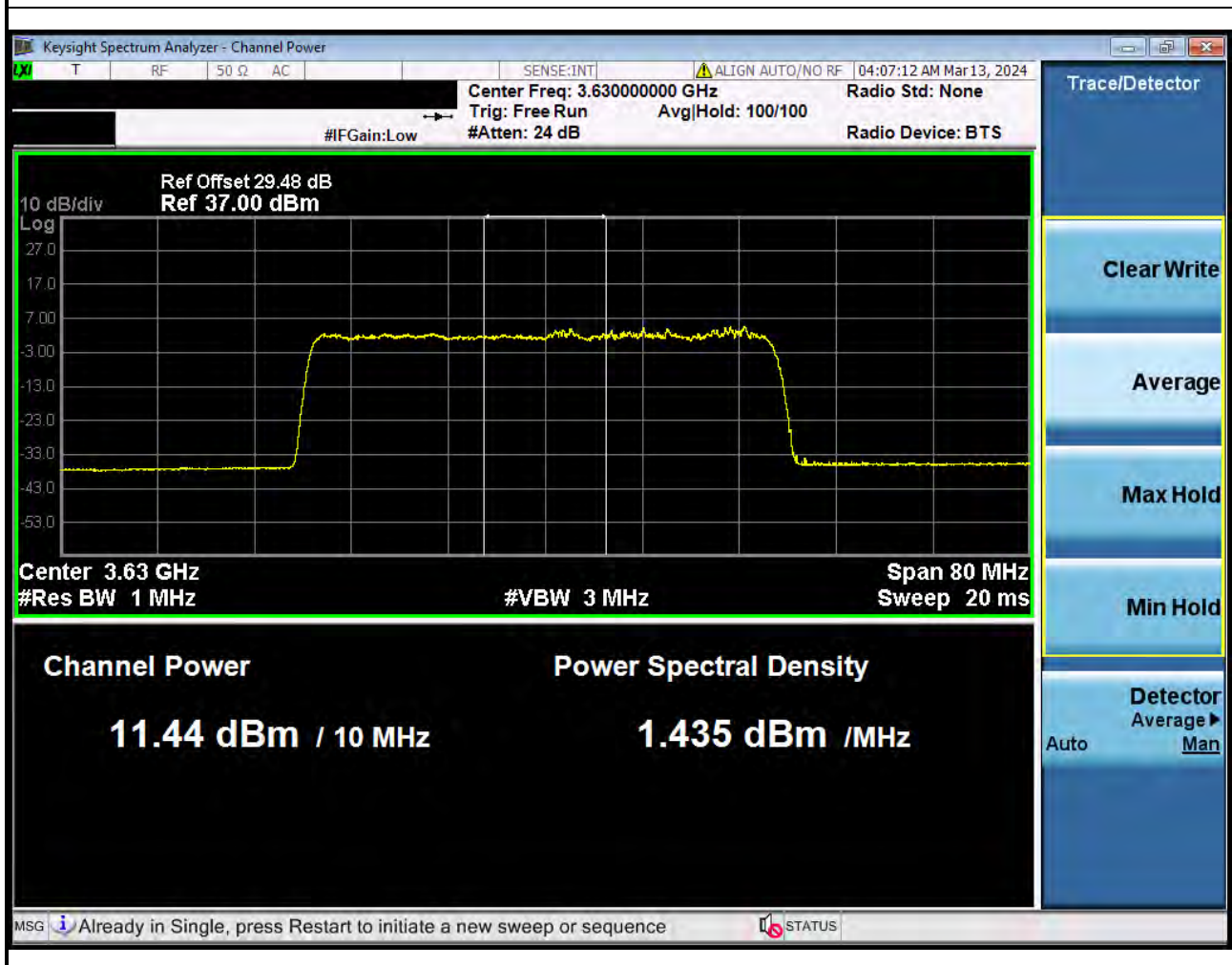
RF measurement plot for WINNF.PT.C.HBT.1 Test Case ID_BW40M_Grant maxEirp 26_Port 1
