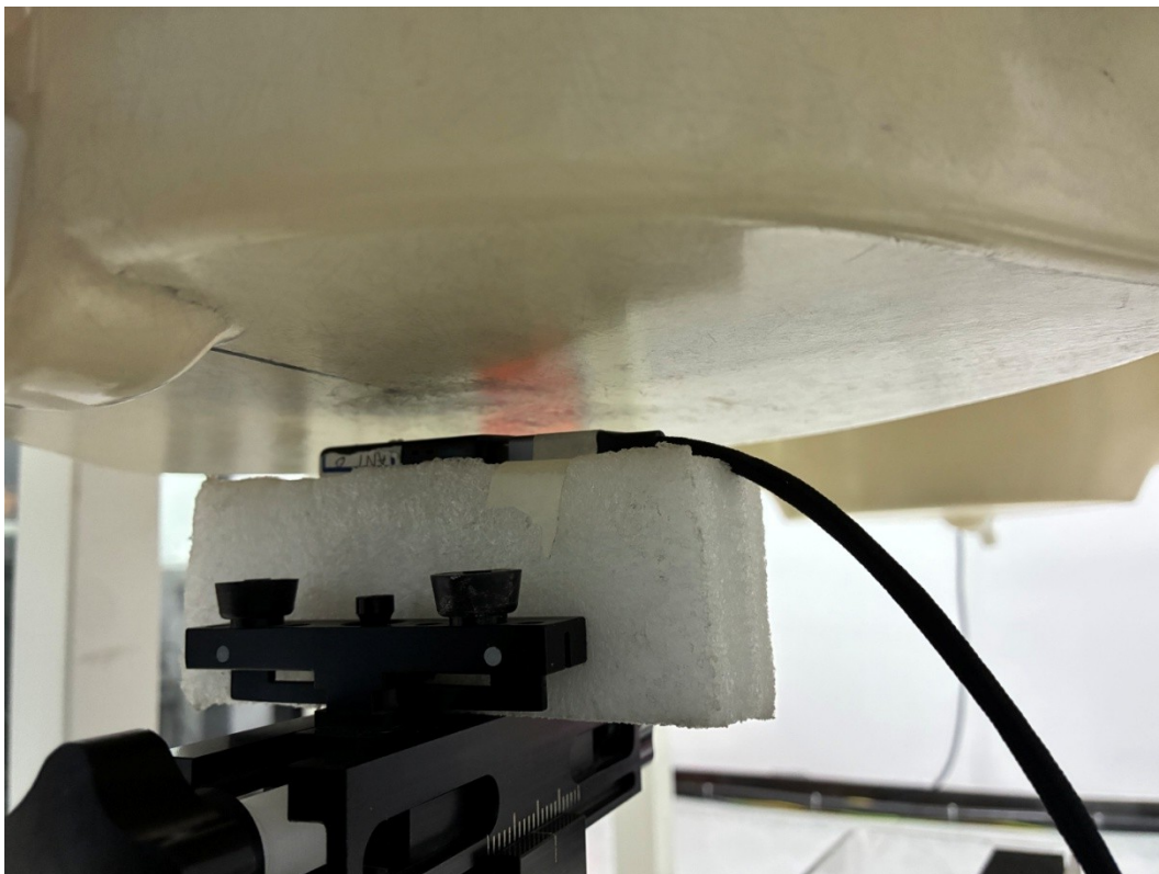
Horizontal-Down Setup Photo (5mm)
