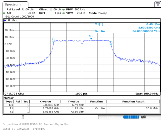
802.11ac40_5795MHz_Chain 1
