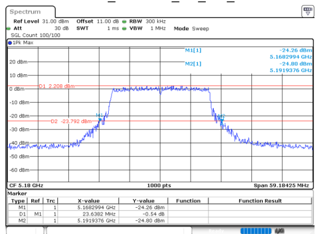
802.11ax20_5180MHz_RU_Full_Chain 0
