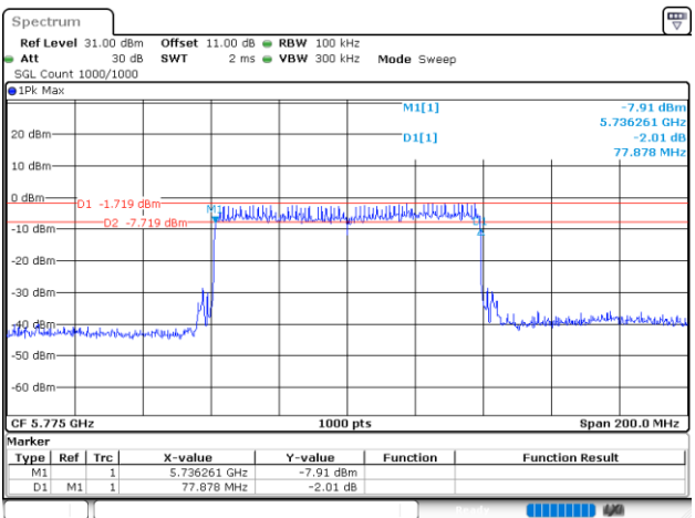
802.11ax80_5775MHz_RU_Full_Chain 1
