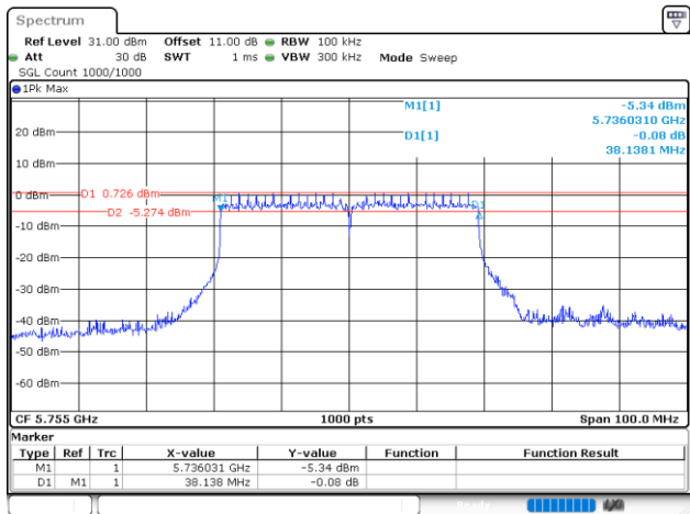
802.11ax40_5755MHz_RU_FULL_Chain 1
