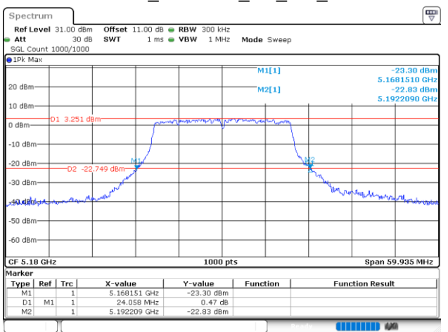
802.11ax20_5180MHz_RU_Full_Chain 1
