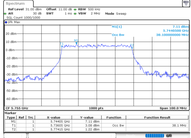
802.11ax40_5755MHz_RU_FULL_Chain 1
