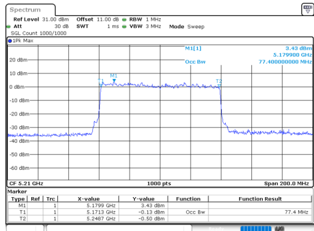
802.11ax80_5210MHz_RU_Full_Chain 0
