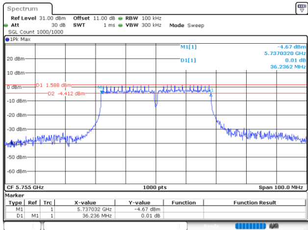
802.11ax40_5755MHz_RU_FULL_Chain 0
