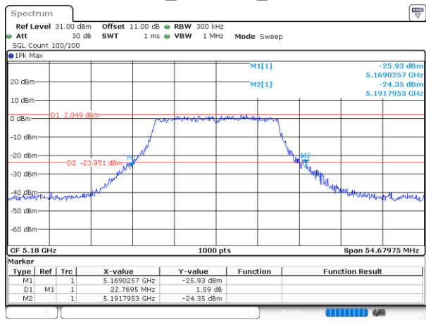
802.11a_5180MHz_Chain 0
