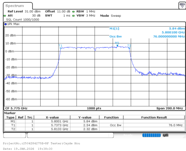
802.11ac80_5775MHz_Chain 1
