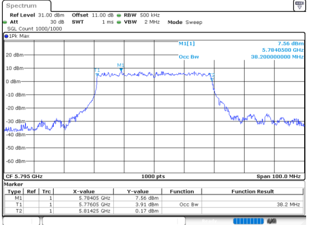
802.11ax40_5795MHz_RU_FULL_Chain 1
