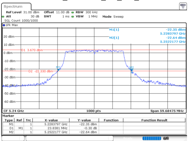
802.11ax20_5240MHz_RU_Full_Chain 1
