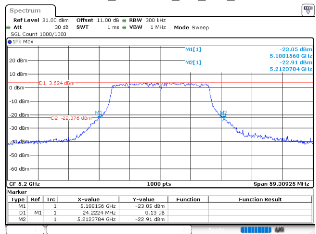
802.11ax20_5200MHz_RU_Full_Chain 1
