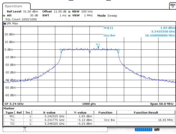
802.11a_5240MHz_Chain 1
