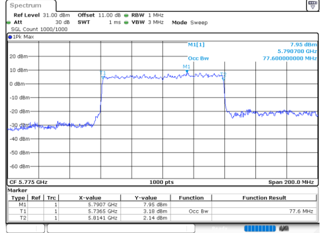
802.11ax80_5775MHz_RU_Full_Chain 0
