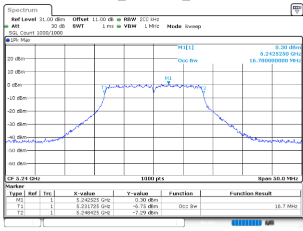
802.11a_5240MHz_Chain 0
