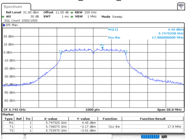
802.11ac20_5745MHz_Chain 1
