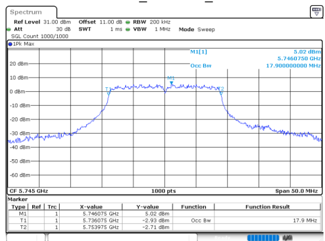
802.11ac20_5745MHz_Chain 0
