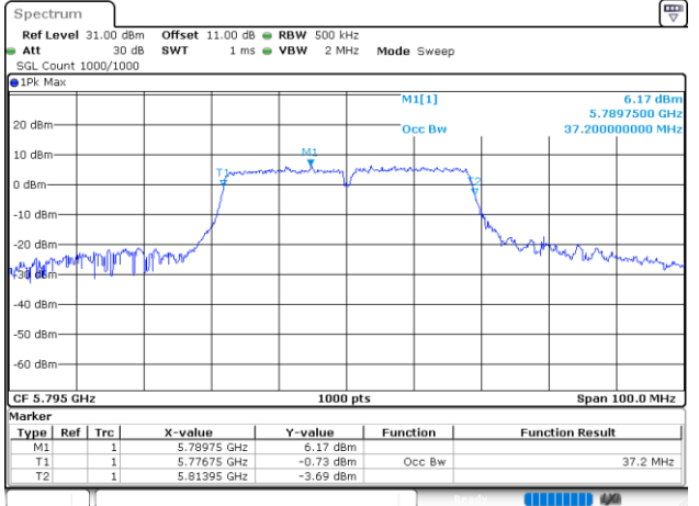
802.11ax40_5795MHz_RU_FULL_Chain 0
