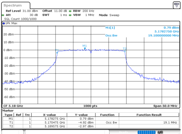
802.11ax20_5180MHz_RU_Full_Chain 1
