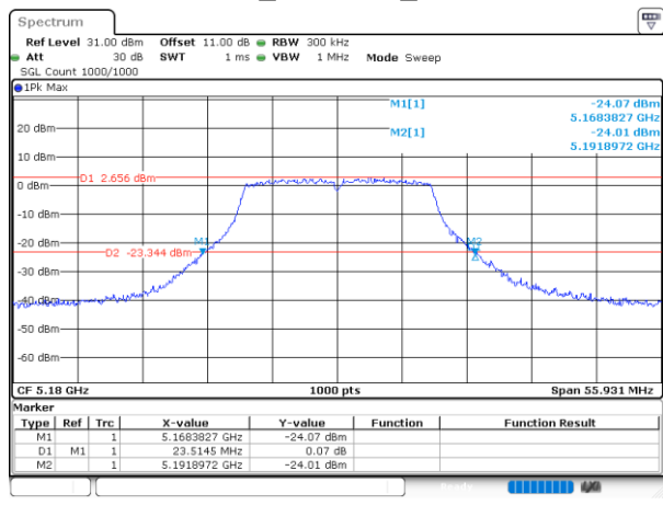
802.11a_5180MHz_Chain 1
