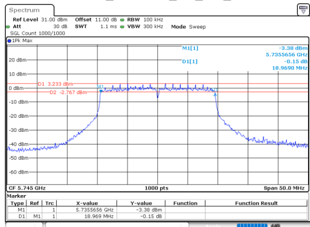
802.11ax20_5745MHz_RU_Full_Chain 1
