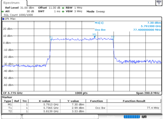
802.11ax80_5775MHz_RU_Full_Chain 1
