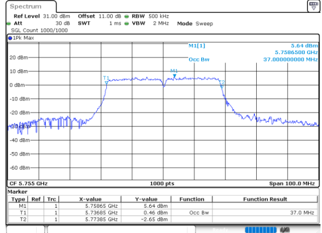
802.11ax40_5755MHz_RU_FULL_Chain 0
