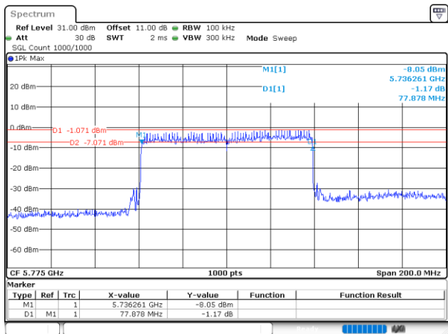
802.11ax80_5775MHz_RU_Full_Chain 0
