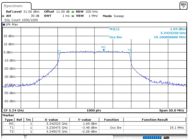
802.11ax20_5240MHz_RU_Full_Chain 1
