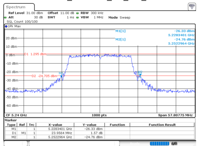
802.11ax20_5240MHz_RU_Full_Chain 0
