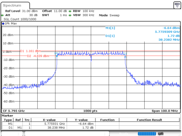
802.11ax40_5795MHz_RU_FULL_Chain 1
