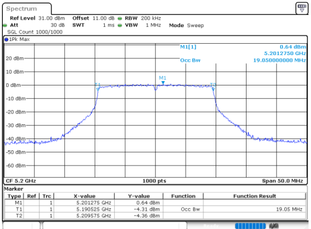
802.11ax20_5200MHz_RU_Full_Chain 0
