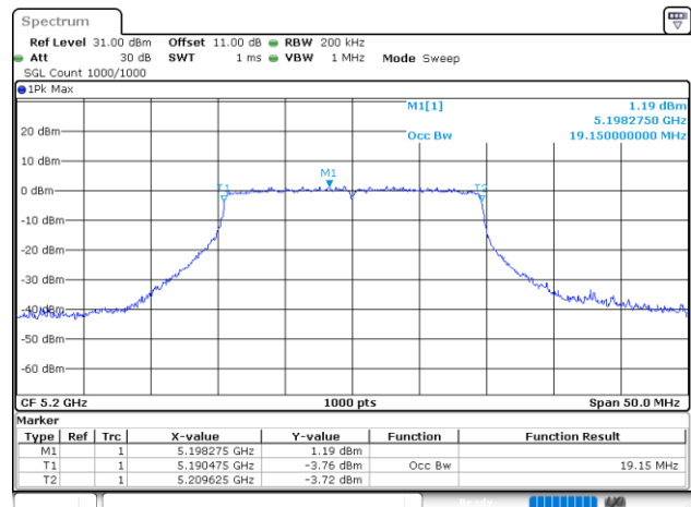
802.11ax20_5200MHz_RU_Full_Chain 1
