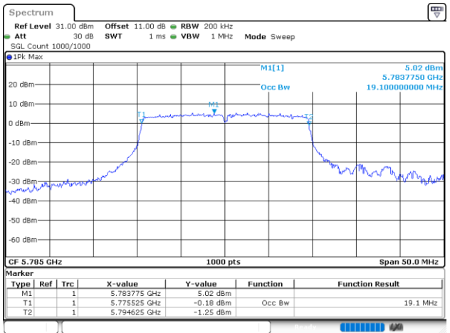
802.11ax20_5785MHz_RU_Full_Chain 0
