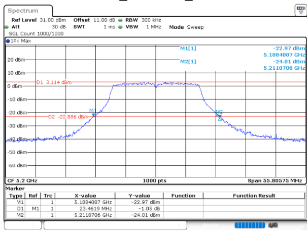
802.11a_5200MHz_Chain 1
