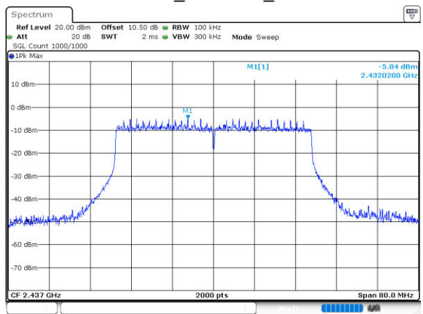
802.11n40_2437MHz_Chain 1
