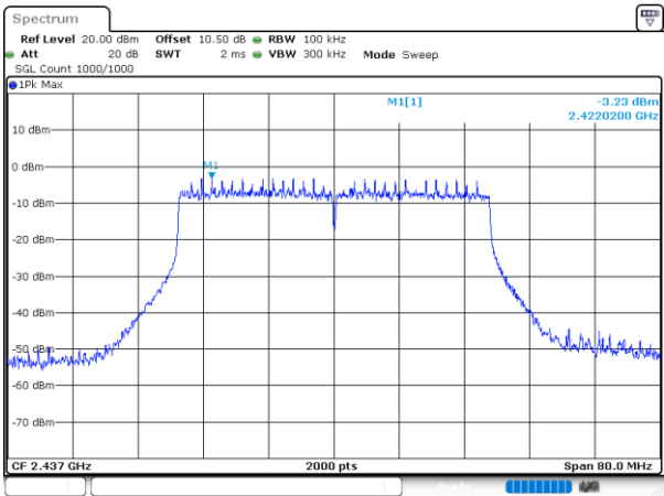
802.11ax40_2437MHz_RU_Full_Chain 0
