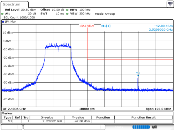
802.11ax20_2462MHz_RU_Full_Chain 1
