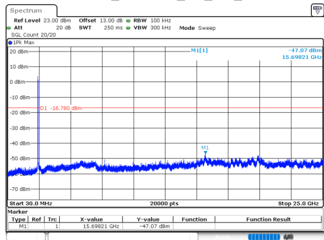
802.11ax20_2412MHz_RU_Full_Chain 0
