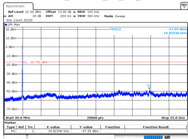
802.11ax20_2437MHz_RU_Full_Chain 0
