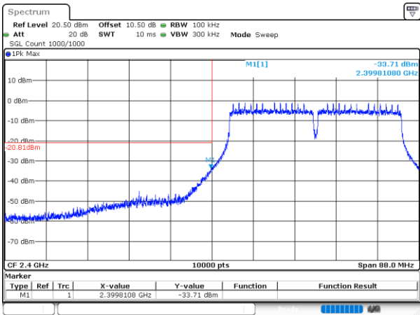
802.11n40_2422MHz_Chain 0
