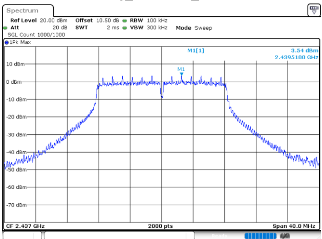
802.11g_2437MHz_Chain 0
