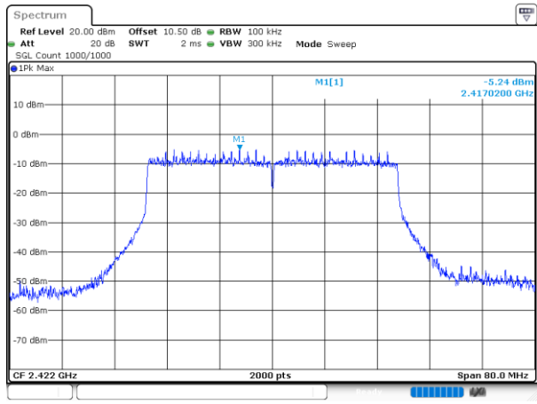
802.11ax40_2422MHz_RU_Full_Chain 1
