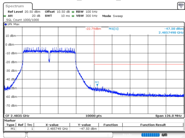
802.11n40_2452MHz_Chain 0
