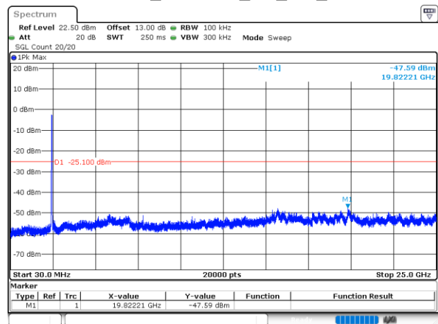
802.11ax40_2437MHz_RU_Full_Chain 1
