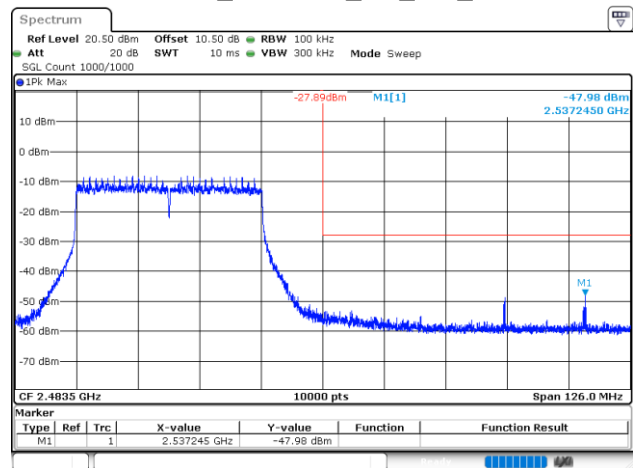
802.11ax40_2452MHz_RU_Full_Chain 1
