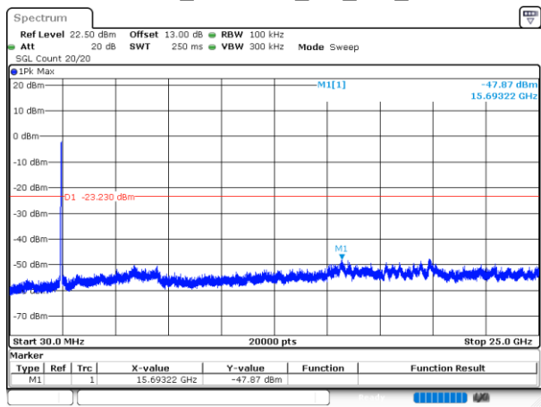
802.11ax40_2437MHz_RU_Full_Chain 0
