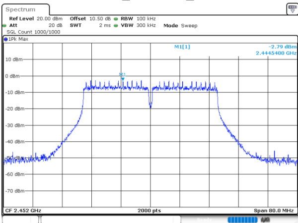
802.11n40_2452MHz_Chain 0
