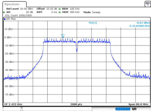
802.11n40_2422MHz_Chain 0
