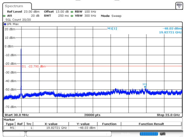
802.11n40_2452MHz_Chain 0
