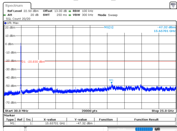
802.11n40_2437MHz_Chain 0
