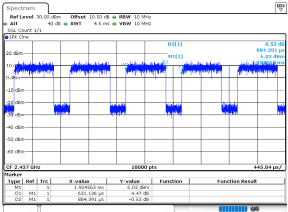
802.11n40_2437MHz_Chain 1
