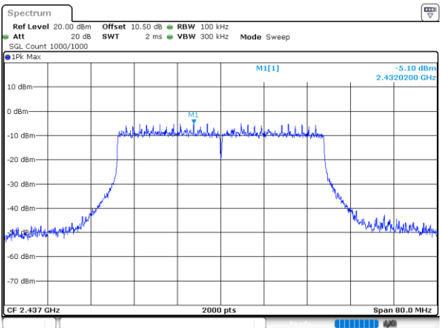
802.11ax40_2437MHz_RU_Full_Chain 1
