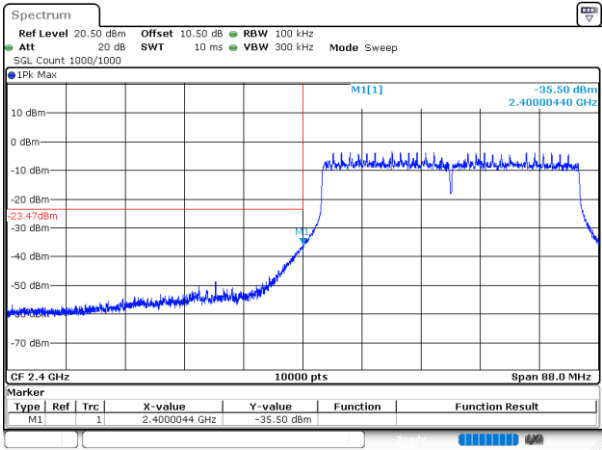
802.11ax40_2422MHz_RU_Full_Chain 0
