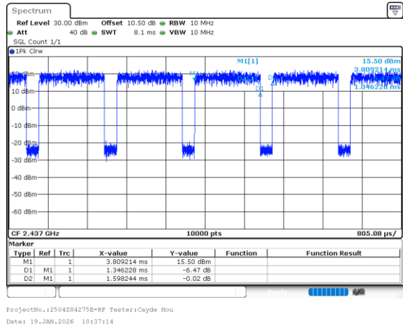
802.11g_2437MHz_Chain 0
