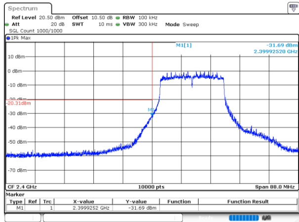
802.11ax20_2412MHz_RU_Full_Chain 1
