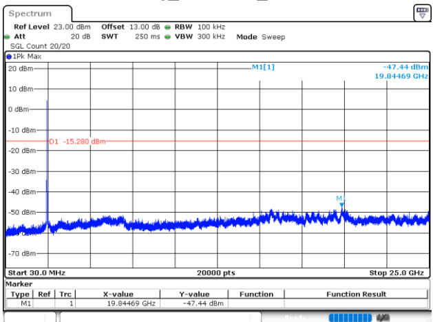
802.11g_2462MHz_Chain 0
