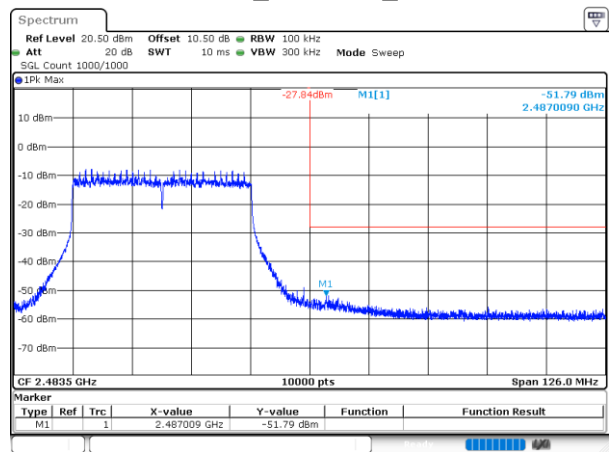
802.11n40_2452MHz_Chain 1
