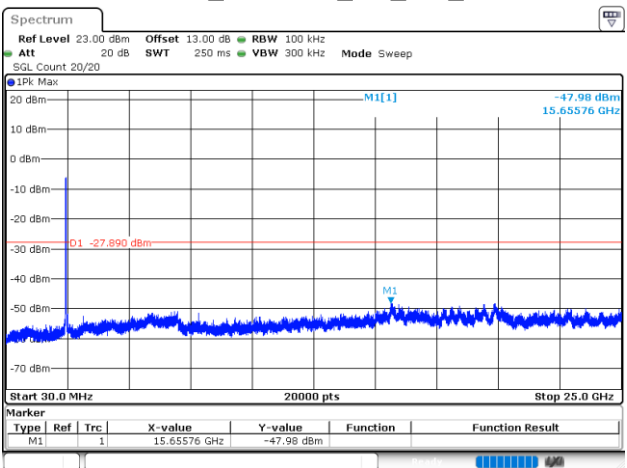
802.11ax40_2452MHz_RU_Full_Chain 1
