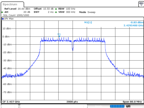
802.11n40_2437MHz_Chain 0
