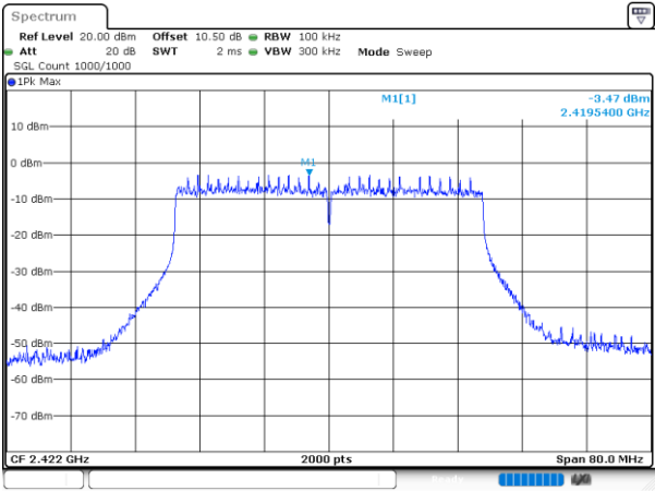
802.11ax40_2422MHz_RU_Full_Chain 0
