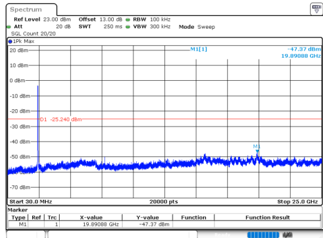
802.11ax40_2422MHz_RU_Full_Chain 1
