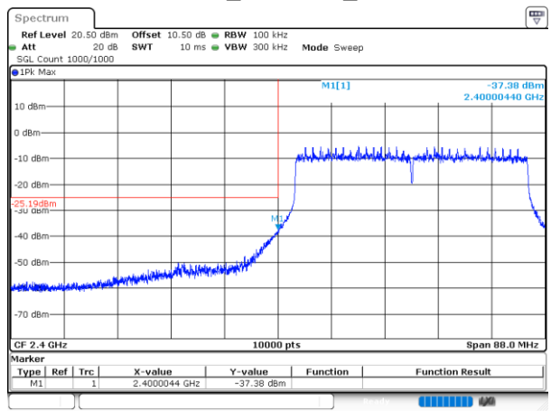
802.11n40_2422MHz_Chain 1
