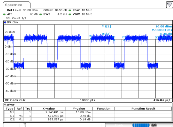
802.11n40_2437MHz_Chain 0
