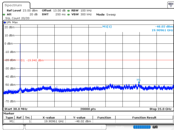
802.11g_2462MHz_Chain 1
