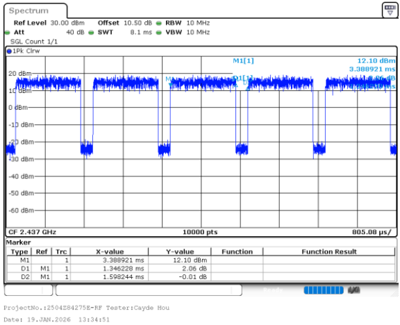
802.11g_2437MHz_Chain 1
