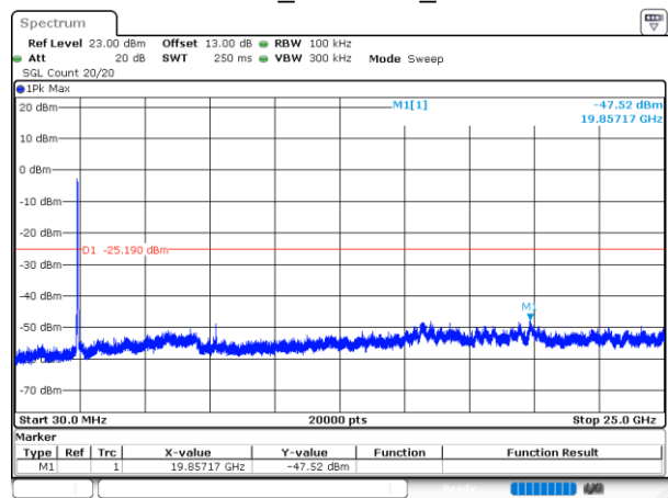
802.11n40_2422MHz_Chain 1
