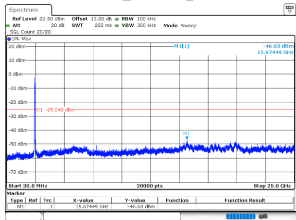
802.11n40_2437MHz_Chain 1
