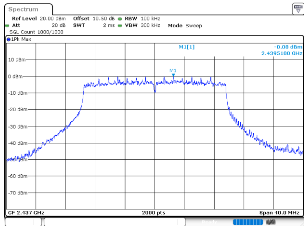
802.11ax20_2437MHz_RU_Full_Chain 1
