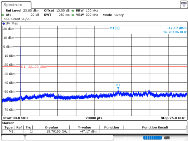
802.11ax20_2462MHz_RU_Full_Chain 1
