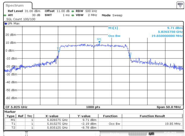
802.11ax20_5825MHz_RU_Full_Chain 0
