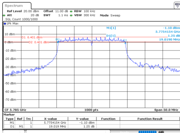
802.11ax20_5785MHz_RU_Full_Chain 1
