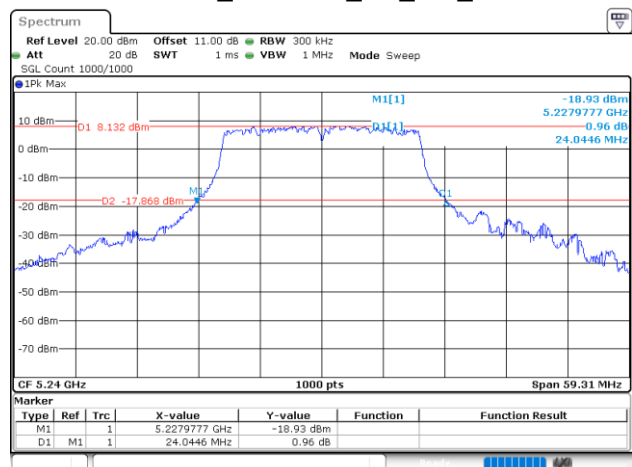
802.11ax20_5240MHz_RU_Full_Chain 1
