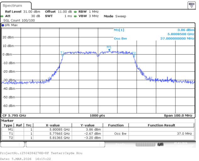
802.11ac40_5795MHz_Chain 1
