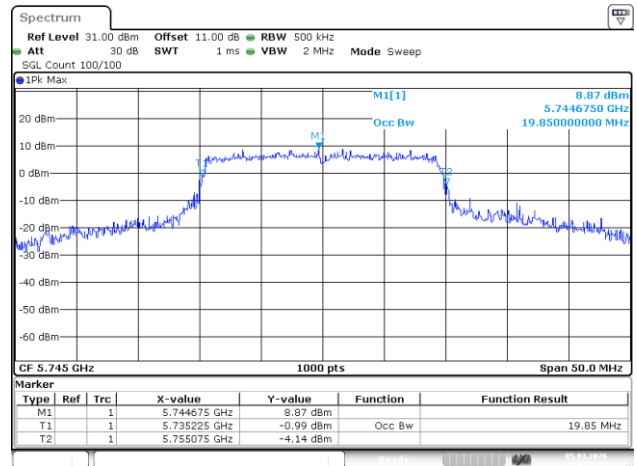
802.11ax20_5745MHz_RU_Full_Chain 0
