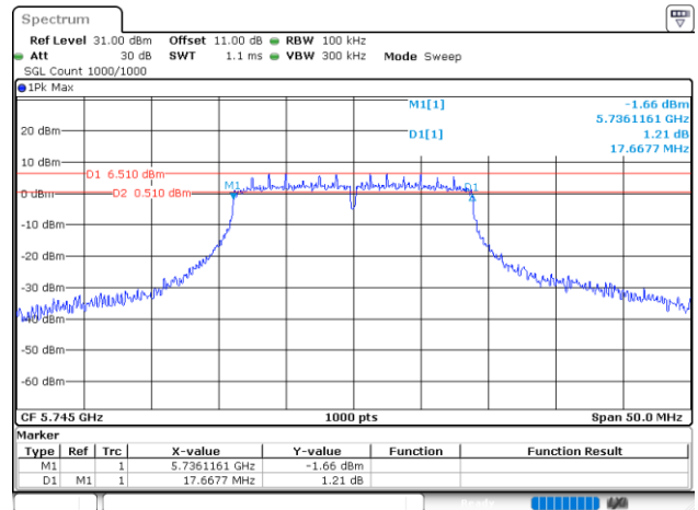
802.11ac20_5745MHz_Chain 0
