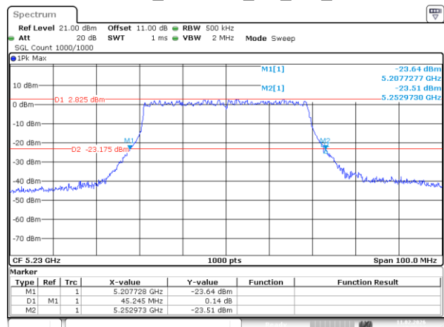
802.11ax40_5230MHz_RU_Full_Chain 1
