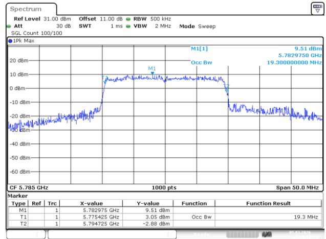
802.11ax20_5785MHz_RU_Full_Chain 1
