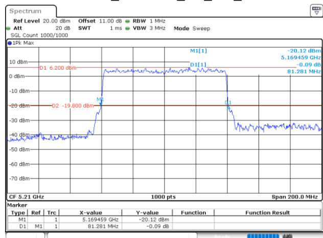
802.11ax80_5210MHz_RU_Full_Chain 1
