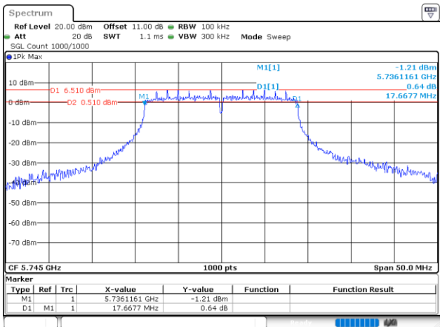
802.11ac20_5745MHz_Chain 1
