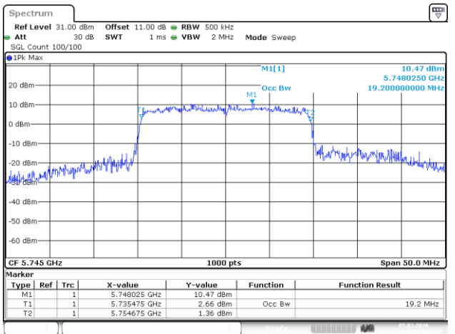
802.11ax20_5745MHz_RU_Full_Chain 1
