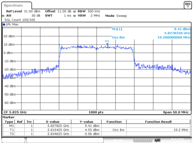
802.11ax20_5825MHz_RU_Full_Chain 1
