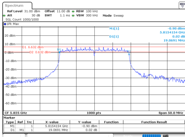
802.11ax20_5825MHz_RU_Full_Chain 0
