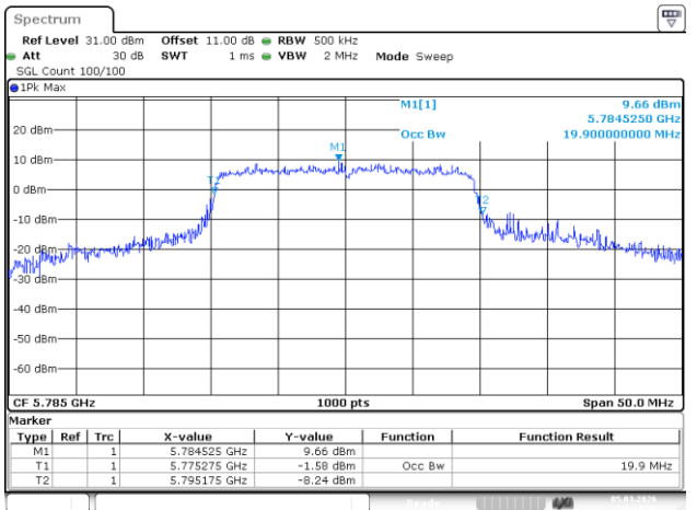
802.11ax20_5785MHz_RU_Full_Chain 0
