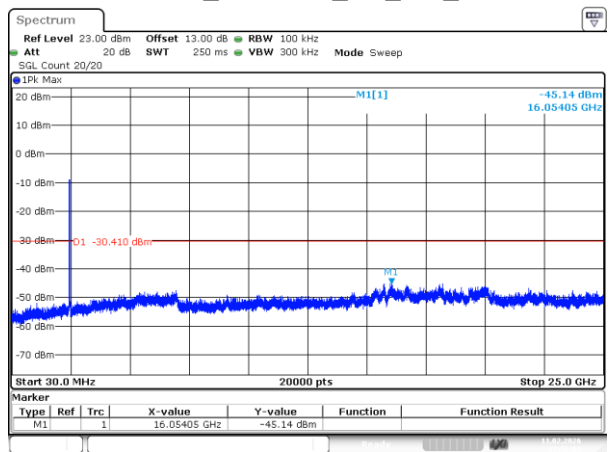
802.11ax40_2452MHz_RU_Full_Chain 0
