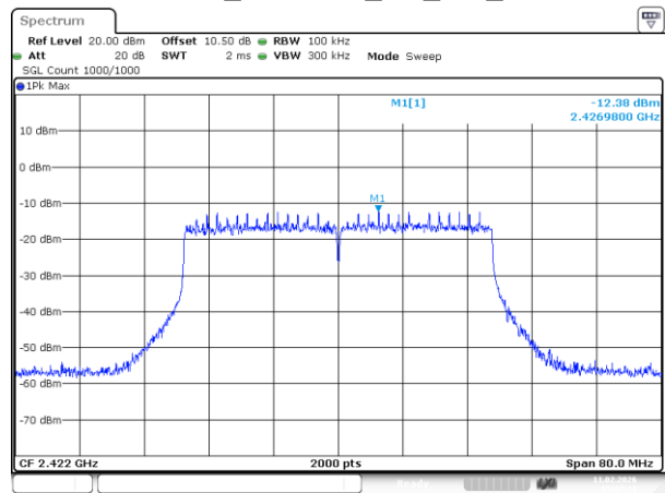
802.11ax40_2422MHz_RU_Full_Chain 1
