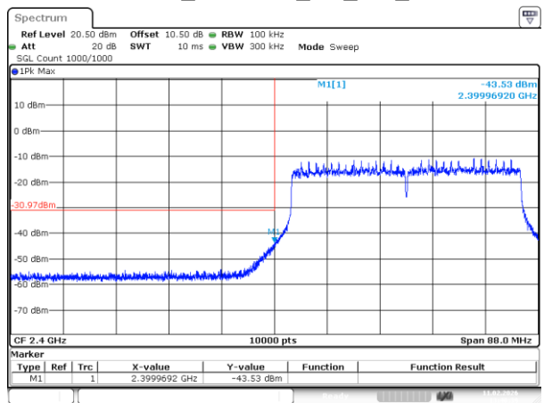
802.11ax40_2422MHz_RU_Full_Chain 0
