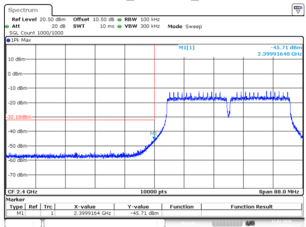
802.11n40_2422MHz_Chain 1
