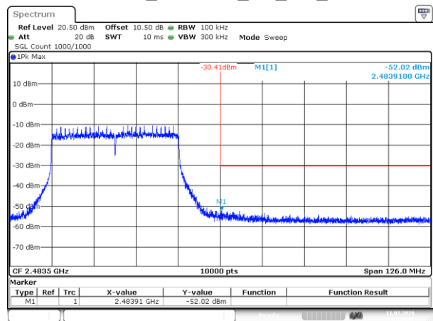
802.11ax40_2452MHz_RU_Full_Chain 0
