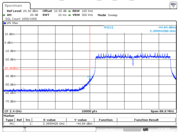
802.11ax40_2422MHz_RU_Full_Chain 1
