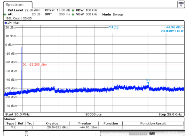
802.11g_2437MHz_Chain 1
