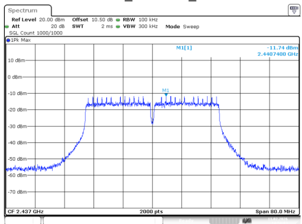
802.11n40_2437MHz_Chain 1
