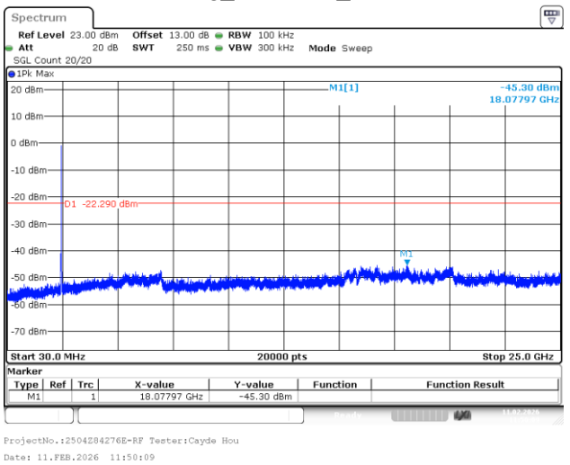
802.11g_2462MHz_Chain 0
