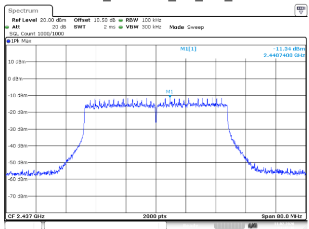
802.11ax40_2437MHz_RU_Full_Chain 0
