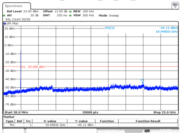
802.11ax20_2462MHz_RU_Full_Chain 1
