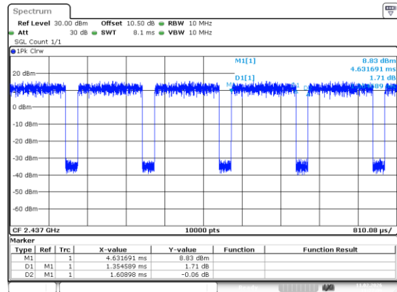
802.11g_2437MHz_Chain 0
