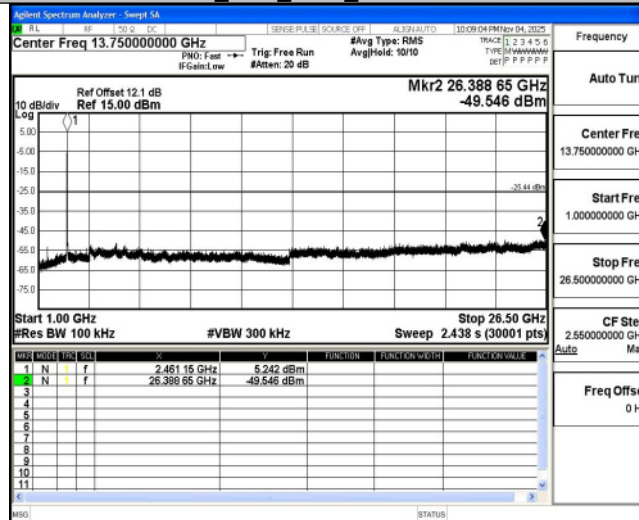
11G_Ant2_2462_0~Reference
