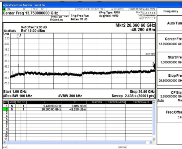
11G_Ant2_2437_0~Reference
