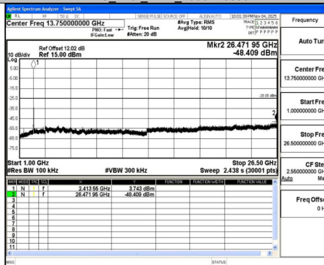
11G_Ant2_2412_0~Reference
