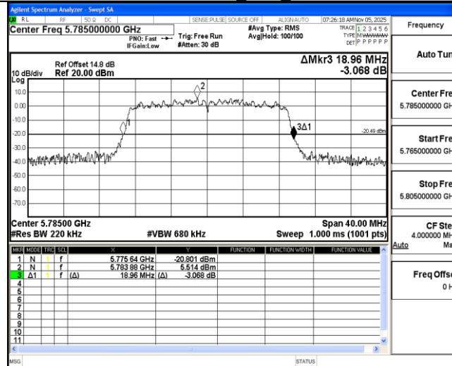
11N20MIMO Ant2 5785
