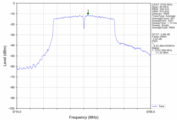
802.11ac(VHT40)_LCH_5755MHz_Ant3_NTNV
