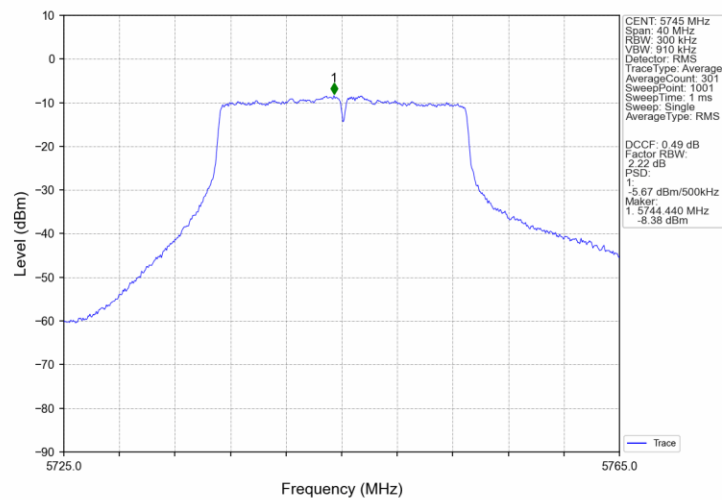
802.11ax(HEW20)_LCH_5745MHz_SU_ / Ant3_NTNV
