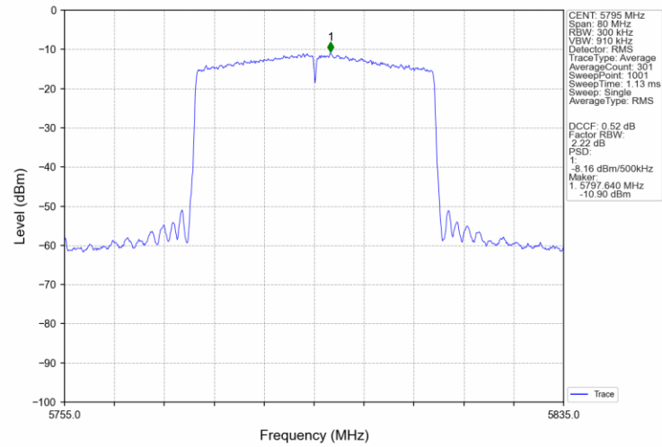
802.11ax(HEW40)_HCH_5795MHz_SU_/_MIMO_NTNV
