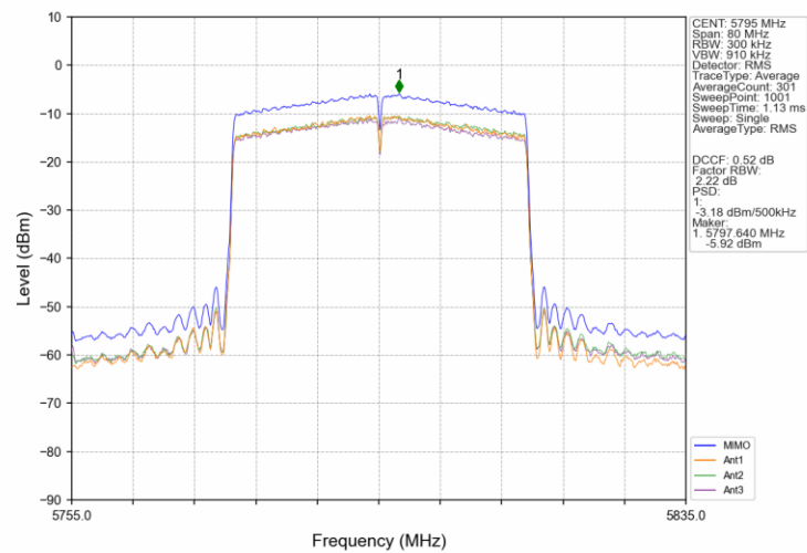
802.11ax(HEW40)_HCH_5795MHz_SU_/_MIMO_NTNV
