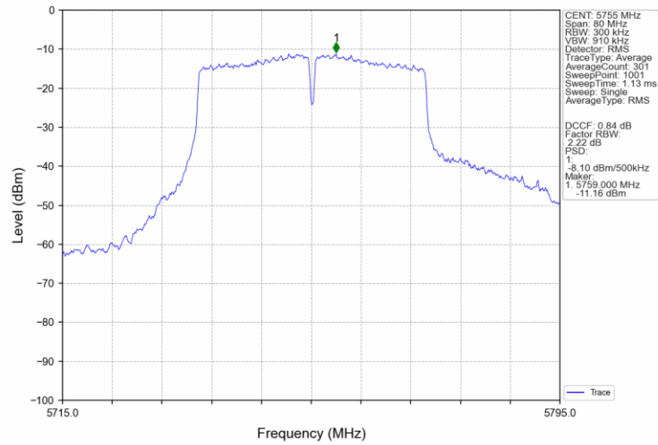
802.11ax(HEW40)_LCH_5755MHz_SU_/_Ant3_NTNV
