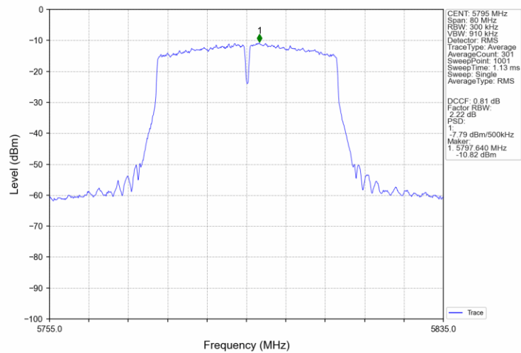
802.11ac(VHT40)_HCH_5795MHz_Ant3_NTNV
