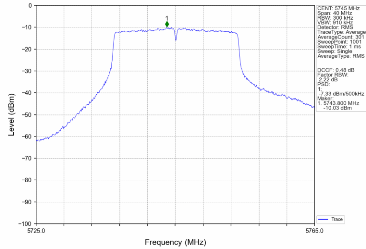
802.11ac(VHT20)_LCH_5745MHz_MIMO_NTNV
