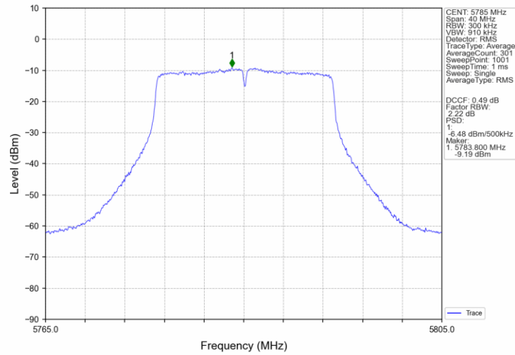
802.11ac(VHT20)_MCH_5785MHz_Ant3_NTNV
