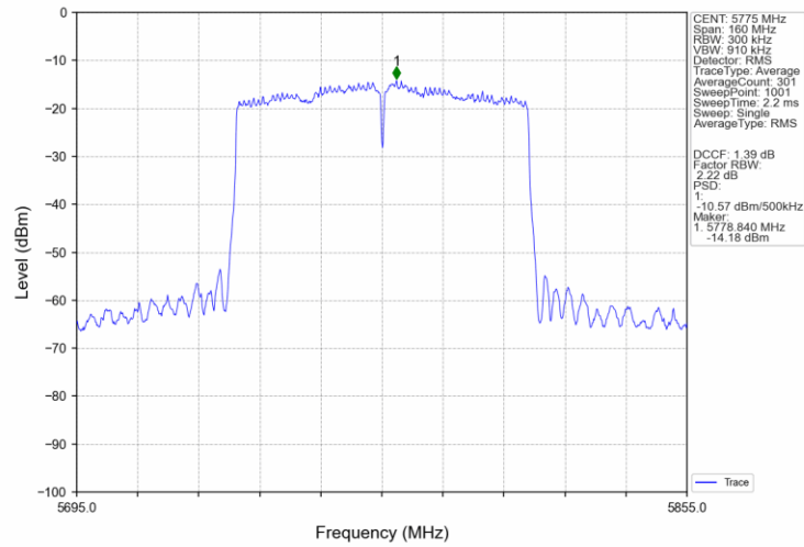
802.11ac(VHT80)_MCH_5775MHz_Ant3_NTNV
