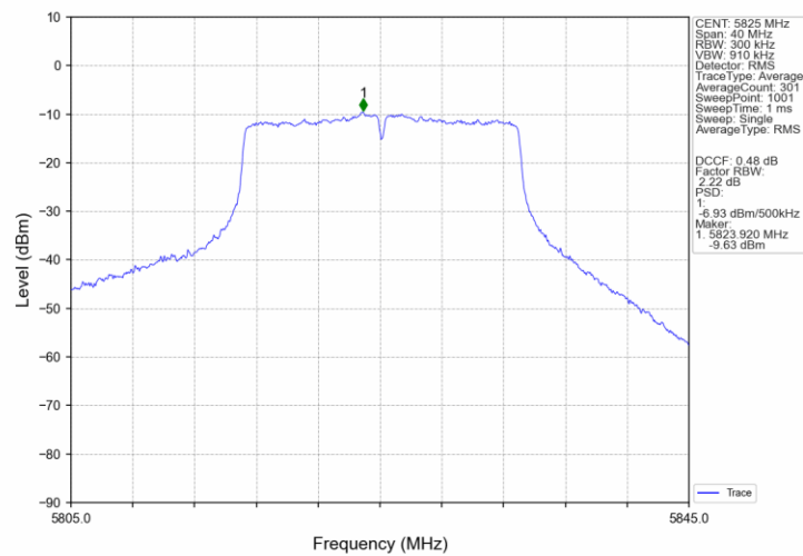
802.11ac(VHT20)_HCH_5825MHz_Ant3_NTNV
