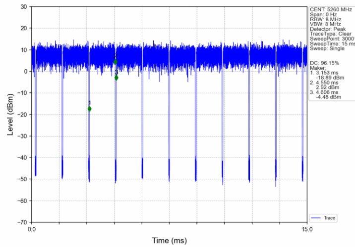
802.11a_LCH_5260MHz_NTNV
