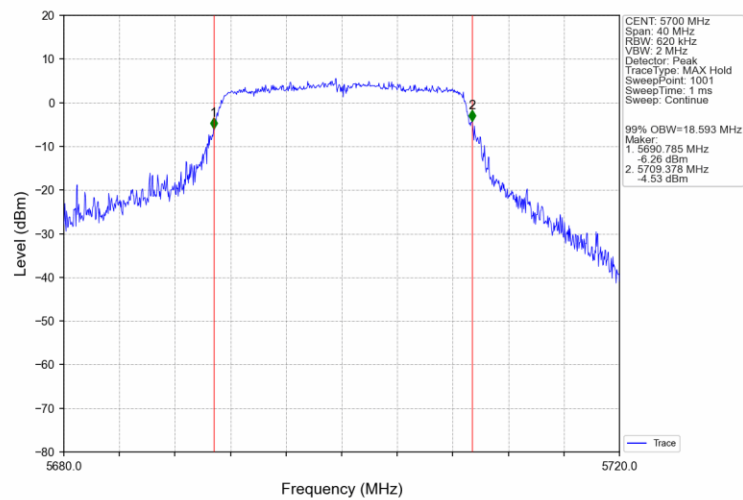
802.11ac(VHT20)_HCH_5700MHz_Ant2_NTNV
