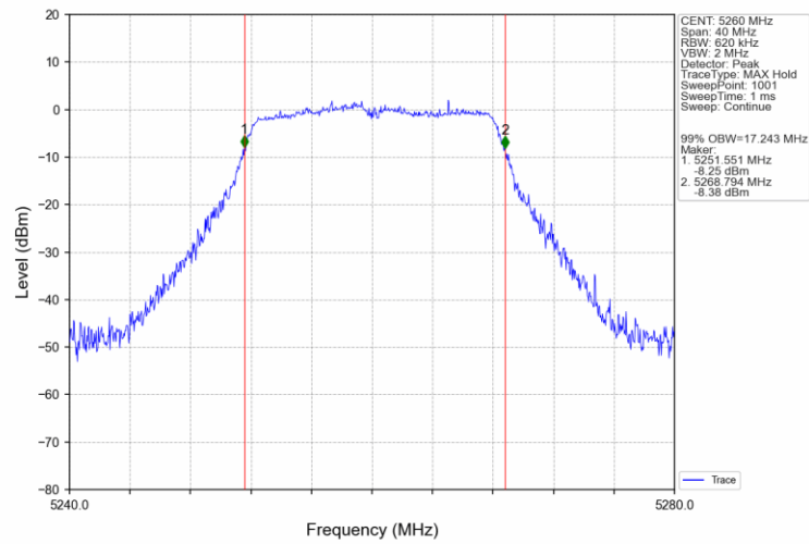
802.11a_LCH_5260MHz_Ant2_NTNV
