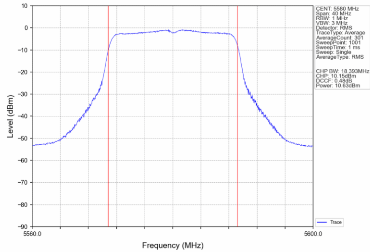
802.11ac(VHT20)_MCH_5580MHz_Ant3_NTNV
