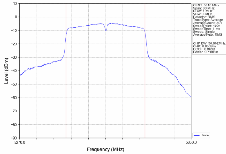
802.11ac(VHT40)_HCH_5310MHz_Ant4_NTNV
