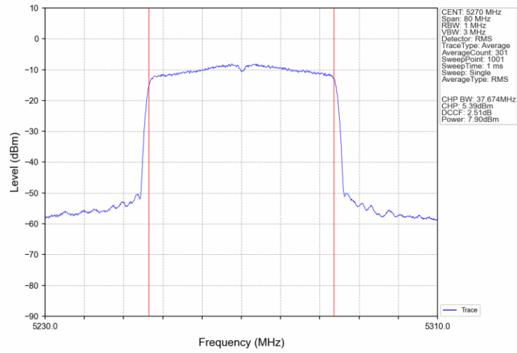
802.11ax(HEW40)_LCH_5270MHz_SU_ / _Ant4_NTNV
