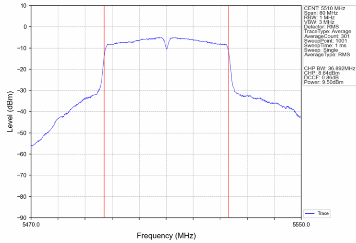
802.11ac(VHT40)_LCH_5510MHz_Ant3_NTNV
