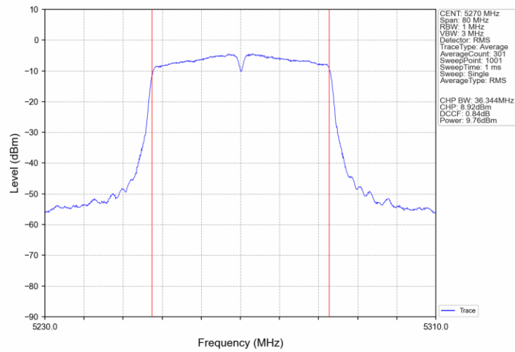
802.11ac(VHT40)_LCH_5270MHz_Ant3_NTNV
