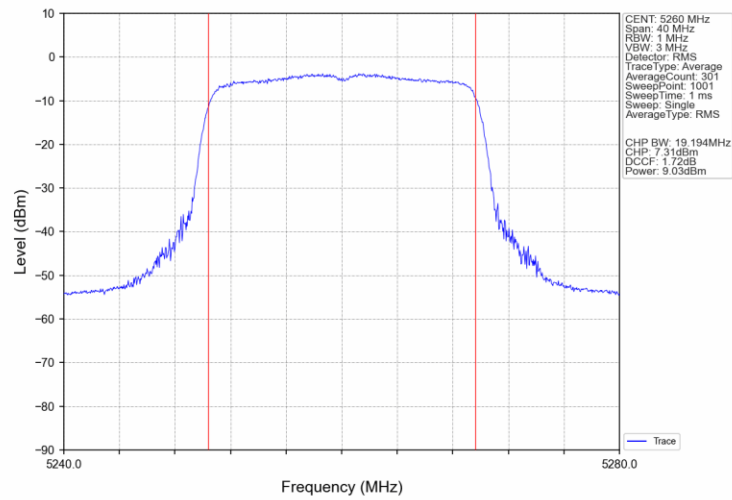
802.11ax(HEW20)_LCH_5260MHz_SU_/_Ant4_NTNV
