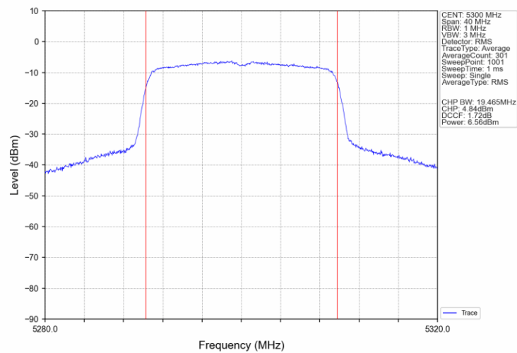
802.11ax(HEW20)_MCH_5300MHz_SU_/_Ant3_NTNV
