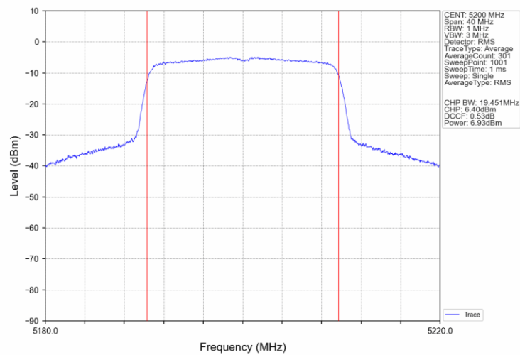
802.11ax(HEW20)_MCH_5200MHz_SU_/_Ant4_NTNV
