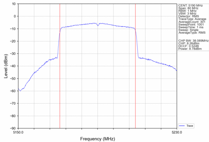
802.11ax(HEW40)_LCH_5190MHz_SU_ / _Ant4_NTNV
