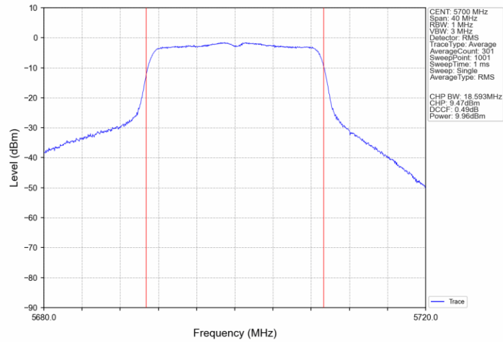
802.11ac(VHT20)_HCH_5700MHz_Ant4_NTNV
