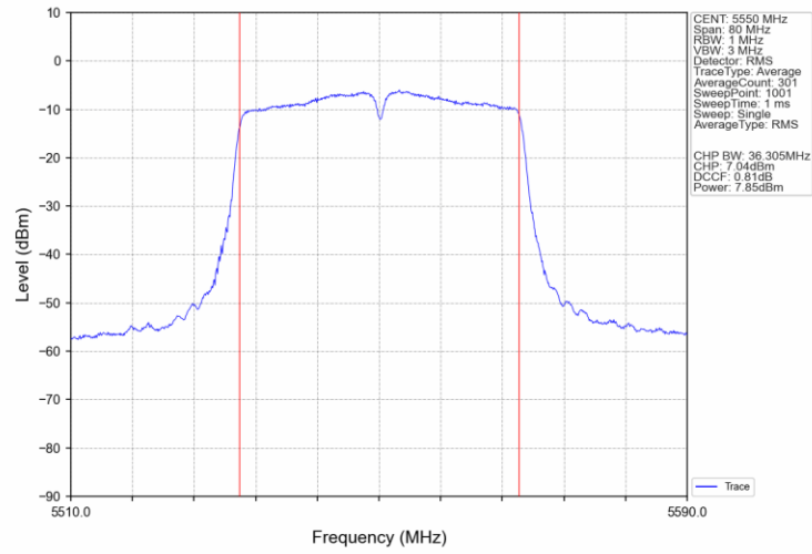
802.11ac(VHT40)_MCH_5550MHz_Ant4_NTNV
