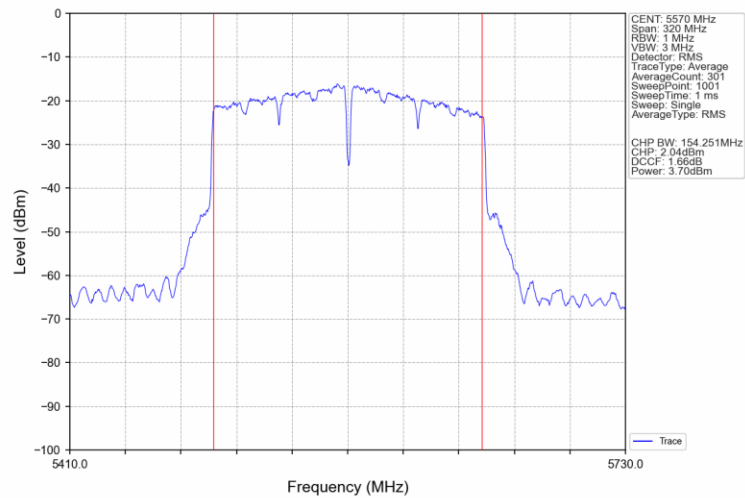
802.11ac(VHT160)_MCH_5570MHz_Ant4_NTNV
