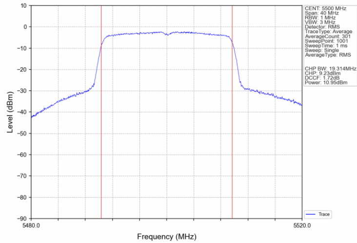
802.11ax(HEW20)_LCH_5500MHz_SU_ / _Ant3_NTNV
