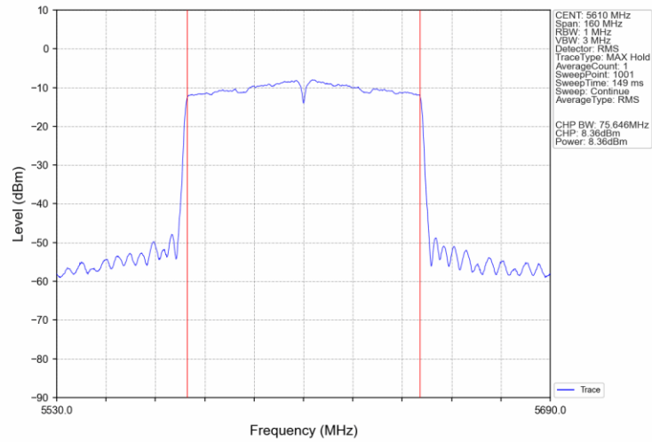
802.11ac(VHT80)_HCH_5610MHz_Ant3_NTNV
