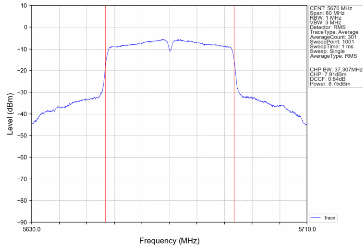
802.11ac(VHT40)_HCH_5670MHz_Ant3_NTNV
