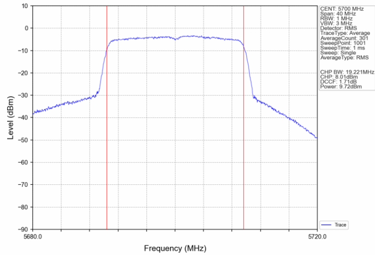
802.11ax(HEW20)_HCH_5700MHz_SU_/_Ant3_NTNV
