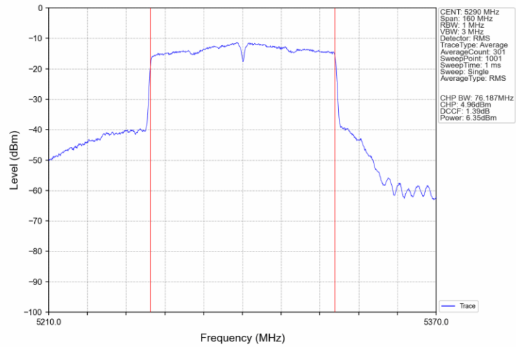
802.11ac(VHT80)_MCH_5290MHz_Ant3_NTNV
