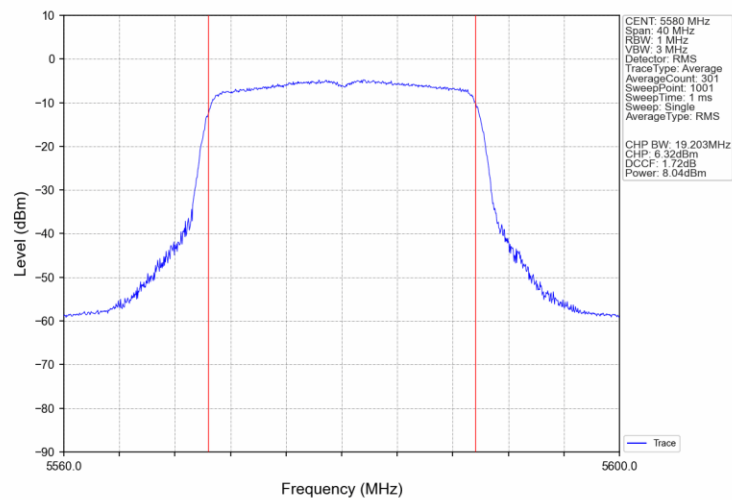
802.11ax(HEW20)_MCH_5580MHz_SU_/_Ant4_NTNV
