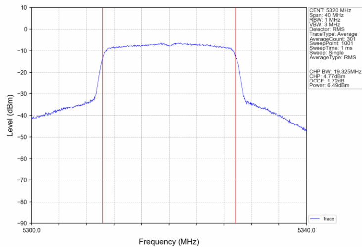
802.11ax(HEW20)_HCH_5320MHz_SU_/_Ant4_NTNV
