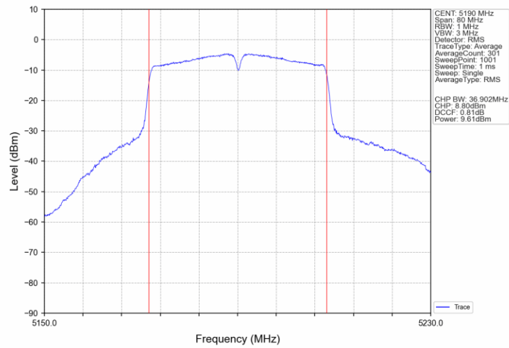
802.11ac(VHT40)_LCH_5190MHz_Ant3_NTNV
