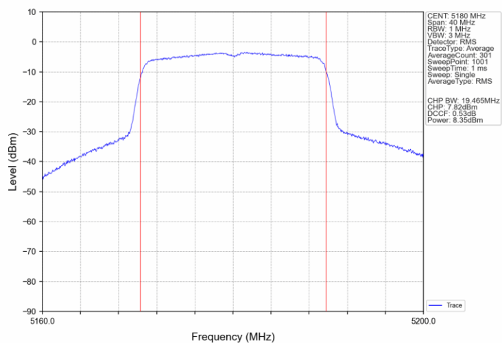
802.11ax(HEW20)_LCH_5180MHz_SU_ / Ant3 NTN
