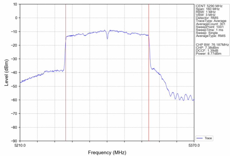
802.11ac(VHT80)_MCH_5290MHz_Ant3_NTNV
