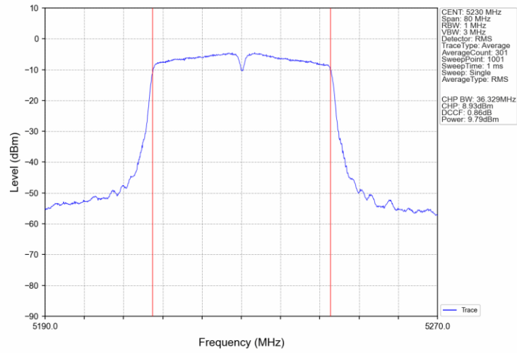
802.11ac(VHT40)_HCH_5230MHz_Ant4_NTNV
