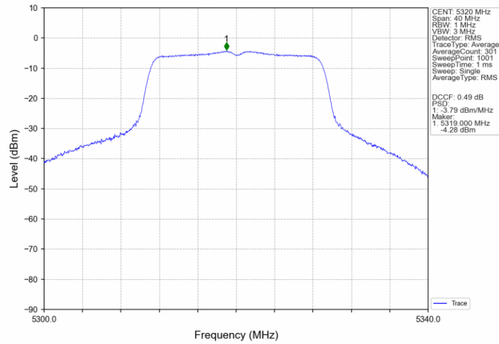
802.11ac(VHT20)_HCH_5320MHz_Ant3_NTNV
