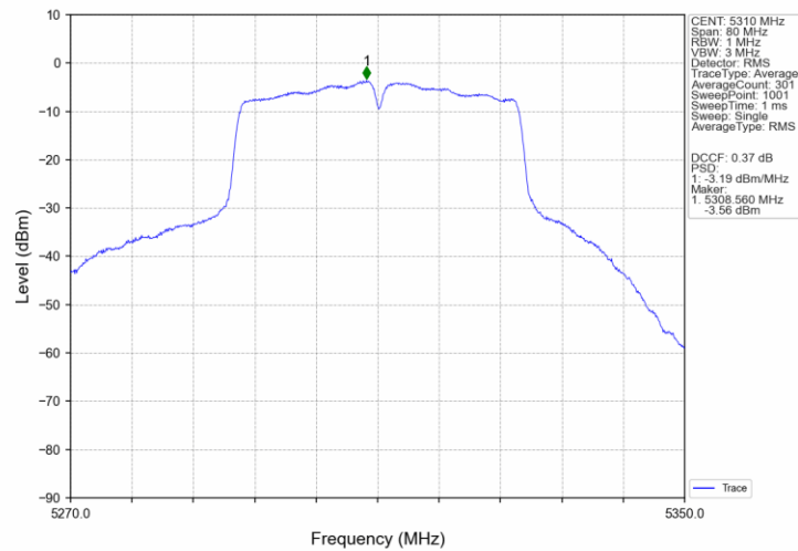
802.11n(HT40)_HCH_5310MHz_Ant3_NTNV
