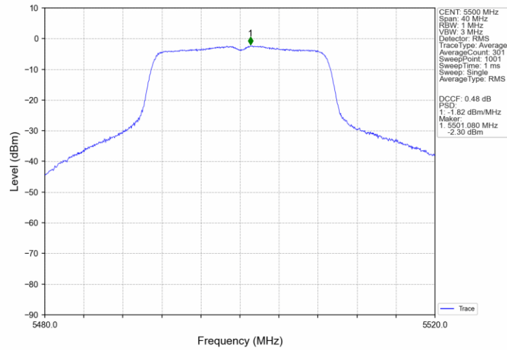
802.11ac(VHT20)_LCH_5500MHz_Ant3_NTNV
