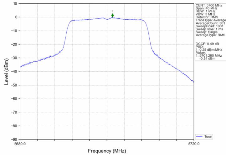
802.11ac(VHT20)_HCH_5700MHz_Ant3_NTNV
