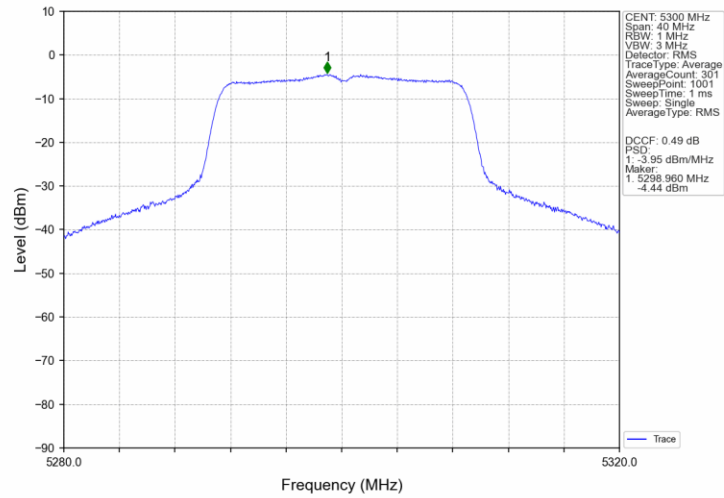
802.11ac(VHT20)_MCH_5300MHz_Ant3_NTNV
