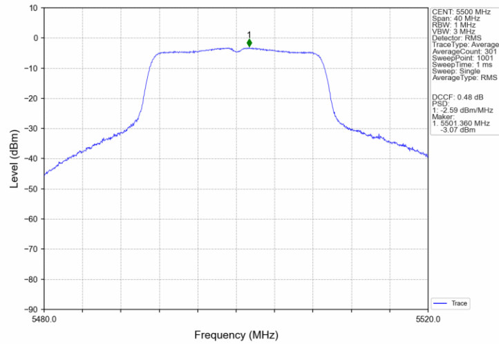
802.11ac(VHT20)_LCH_5500MHz_MIMO_NTNV
