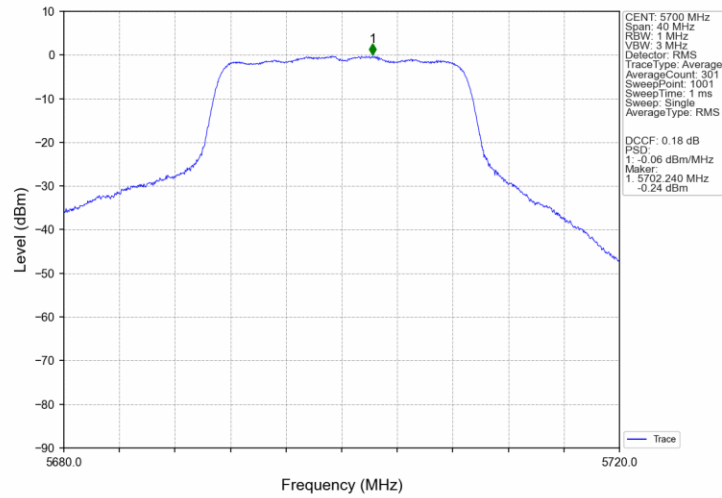
802.11n(HT20)_HCH_5700MHz_Ant3_NTNV
