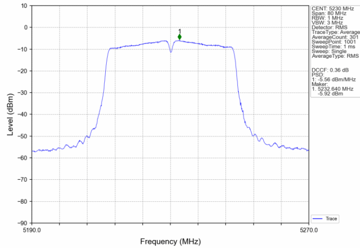
802.11n(HT40)_HCH_5230MHz_MIMO_NTNV
