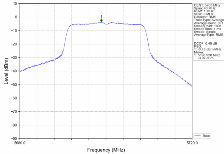
802.11ac(VHT20)_HCH_5700MHz_MIMO_NTNV
