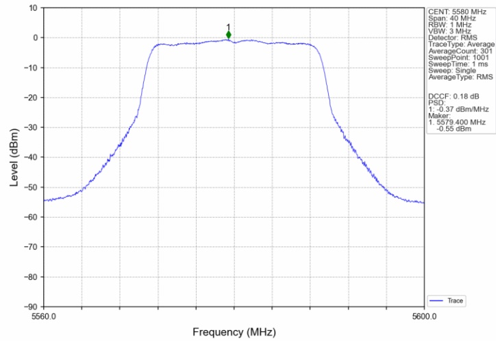
802.11n(HT20)_MCH_5580MHz_Ant3_NTNV
