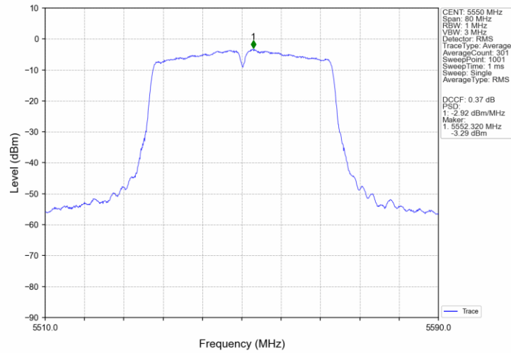
802.11n(HT40)_MCH_5550MHz_Ant3_NTNV
