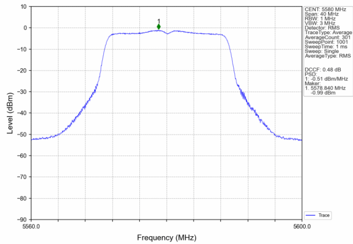
802.11ac(VHT20)_MCH_5580MHz_Ant3_NTNV
