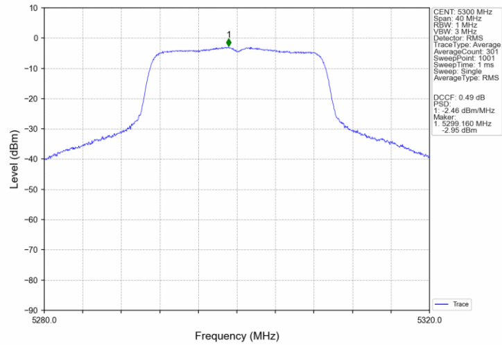
802.11ac(VHT20)_MCH_5300MHz_MIMO_NTNV
