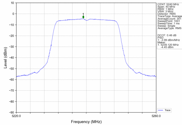
802.11ac(VHT20)_HCH_5240MHz_Ant3_NTNV
