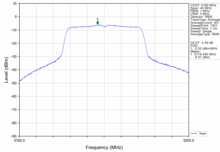
802.11ac(VHT20)_LCH_5180MHz_Ant3_NTNV
