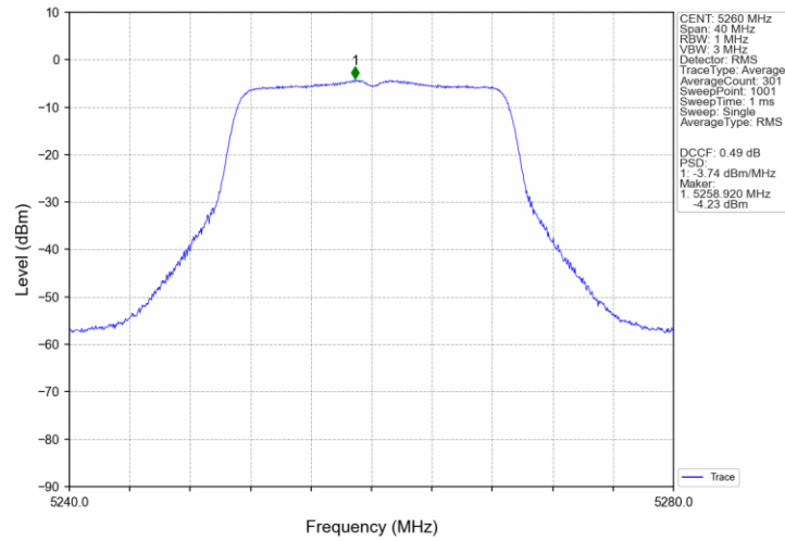
802.11ac(VHT20)_LCH_5260MHz_Ant3_NTNV
