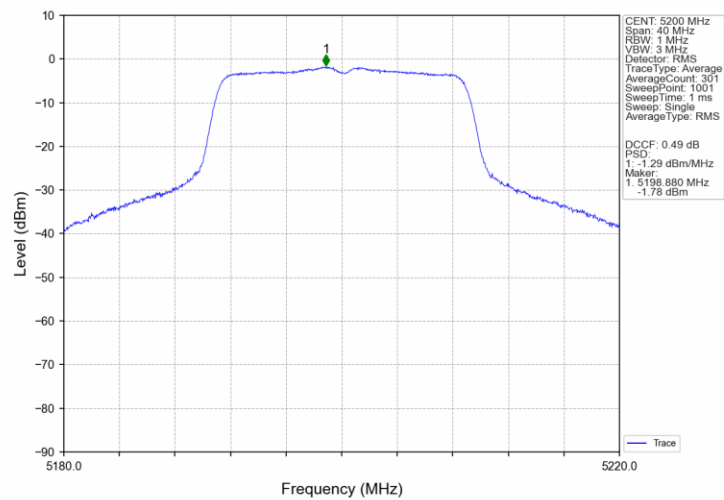
802.11ac(VHT20)_MCH_5200MHz_Ant3_NTNV
