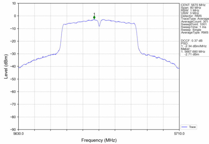
802.11n(HT40)_HCH_5670MHz_Ant3_NTNV
