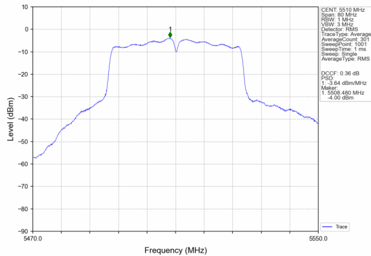
802.11n(HT40)_LCH_5510MHz_Ant3_NTNV
