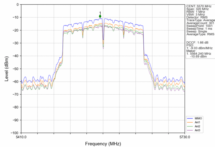
802.11ac(VHT160)_MCH_5570MHz_MIMO_NTNV
