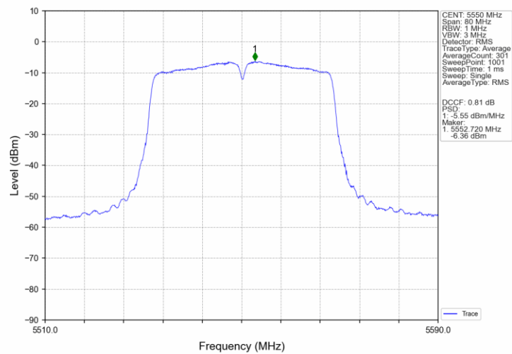
802.11ac(VHT40)_MCH_5550MHz_Ant3_NTNV
