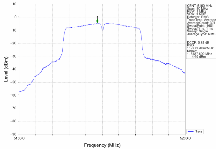
802.11ac(VHT40)_LCH_5190MHz_Ant3_NTNV
