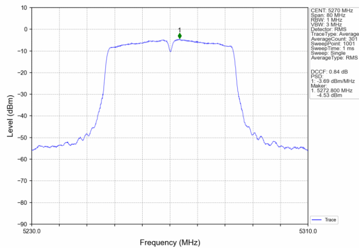
802.11ac(VHT40)_LCH_5270MHz_Ant3_NTNV
