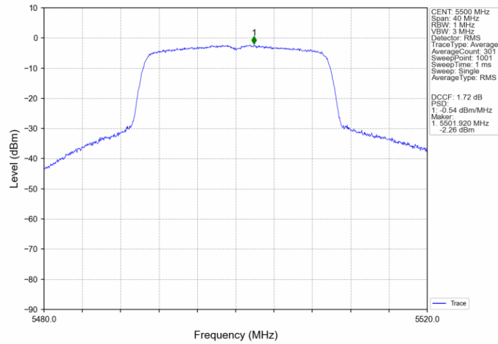
802.11ax(HEW20)_LCH_5500MHz_SU_/_MIMO_NTNV
