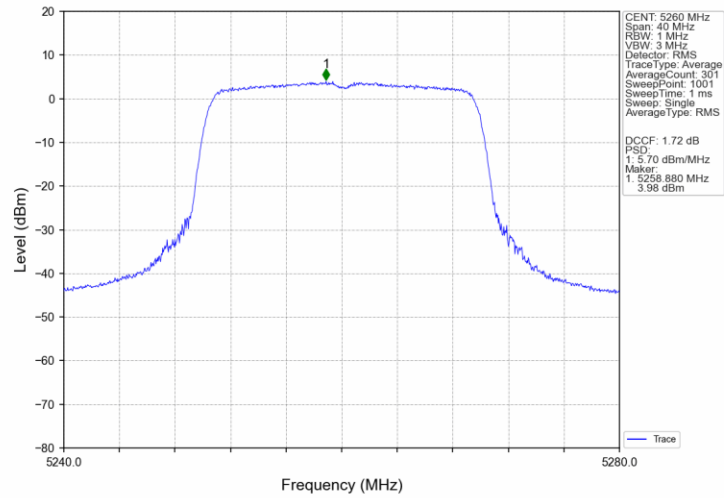
802.11ax(HEW20)_LCH_5260MHz_SU_/_Ant3_NTNV
