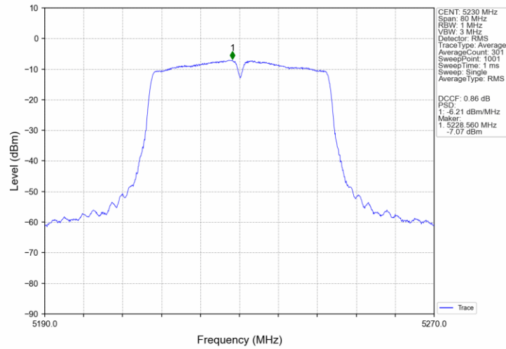
802.11ac(VHT40)_HCH_5230MHz_Ant3_NTNV
