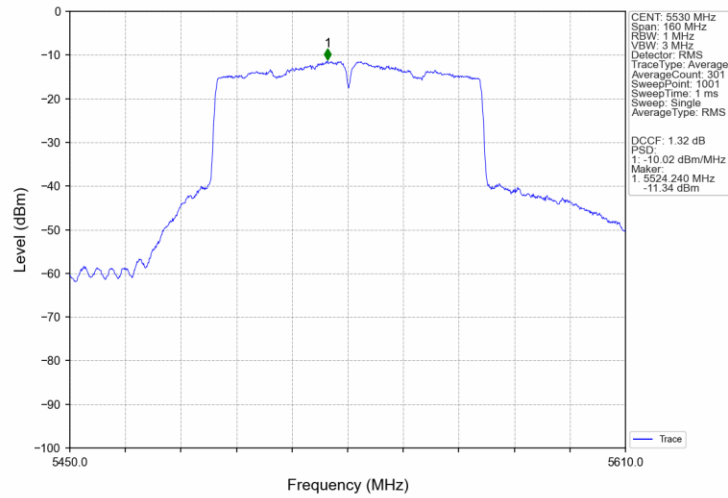
802.11ac(VHT80)_LCH_5530MHz_MIMO_NTNV
