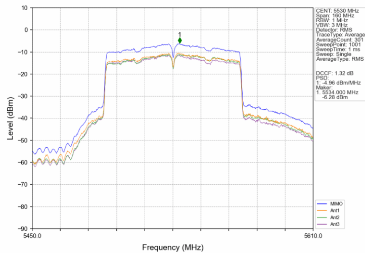
802.11ac(VHT80)_LCH_5530MHz_MIMO_NTNV
