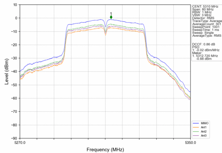
802.11ac(VHT40)_HCH_5310MHz_MIMO_NTNV
