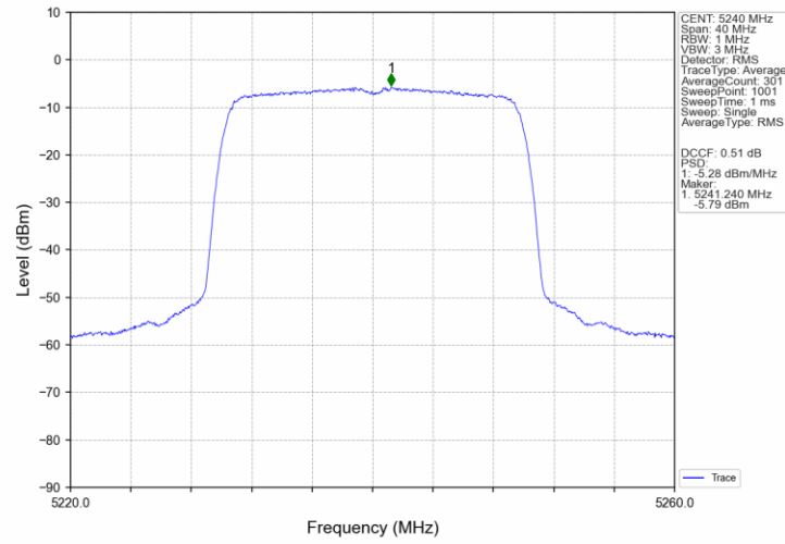
802.11ax(HEW20)_HCH_5240MHz_SU_/_Ant3_NTNV
