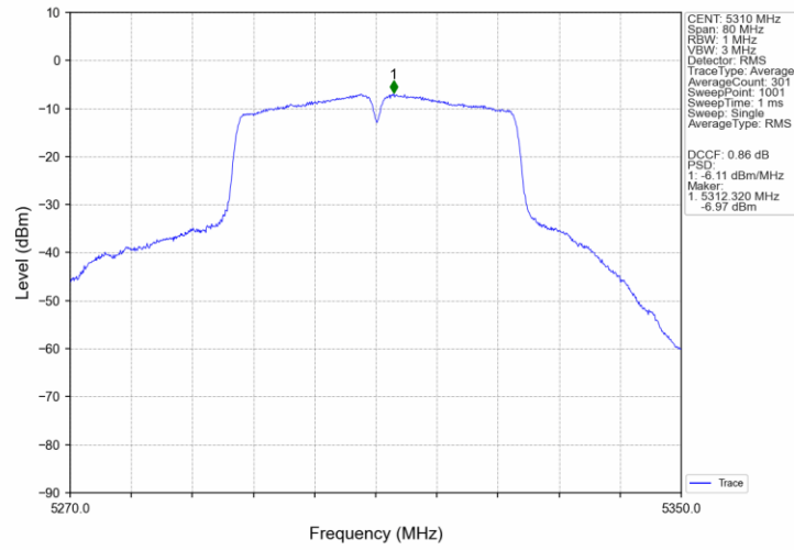
802.11ac(VHT40)_HCH_5310MHz_Ant3_NTNV
