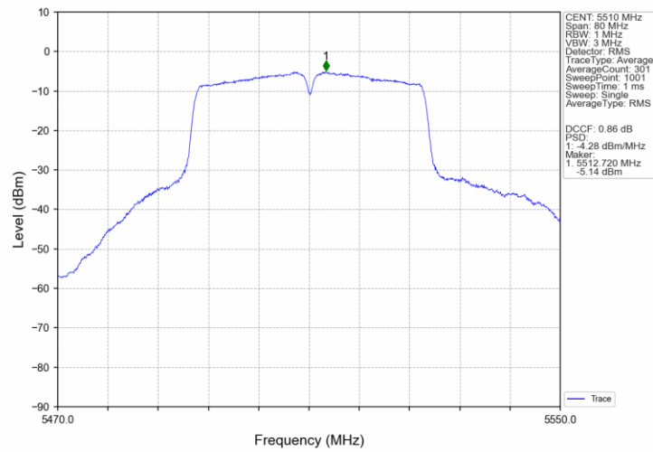
802.11ac(VHT40)_LCH_5510MHz_Ant3_NTNV
