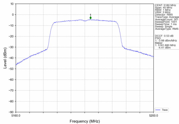
802.11ax(HEW20)_LCH_5180MHz_SU_/_Ant3_NTNV
