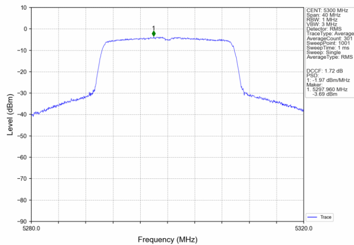
802.11ax(HEW20)_MCH_5300MHz_SU_/_Ant3_NTNV
