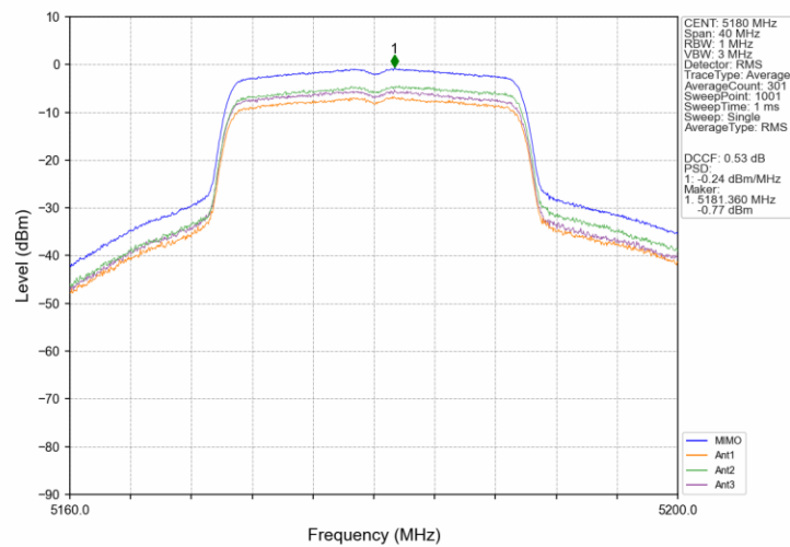
802.11ax(HEW20)_LCH_5180MHz_SU_/_MIMO NTN
