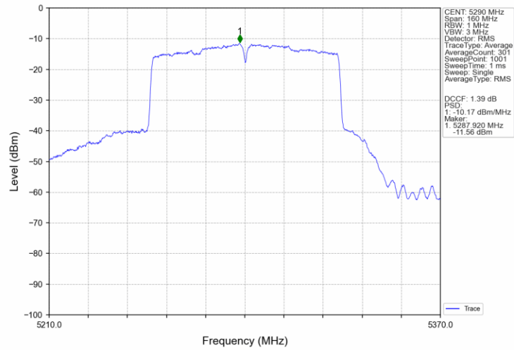
802.11ac(VHT80)_MCH_5290MHz_Ant3_NTNV
