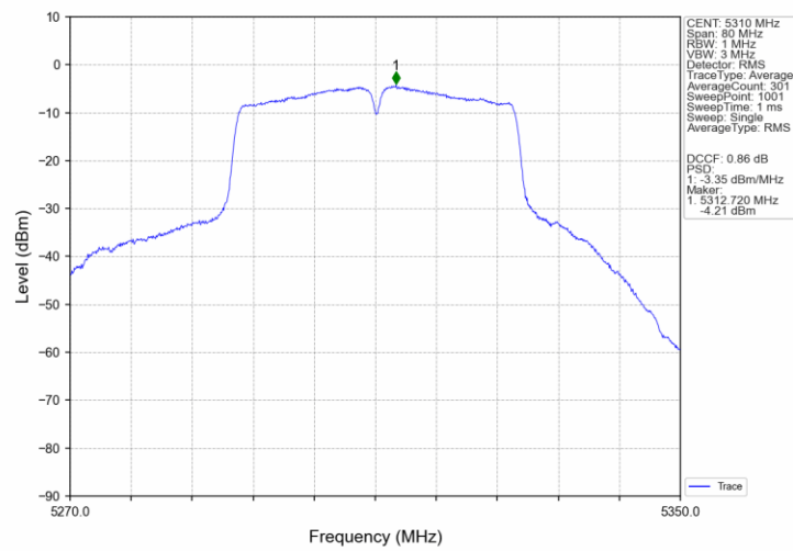
802.11ac(VHT40)_HCH_5310MHz_Ant3_NTNV
