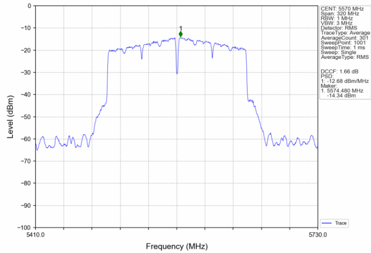
802.11ac(VHT160)_MCH_5570MHz_Ant3_NTNV
