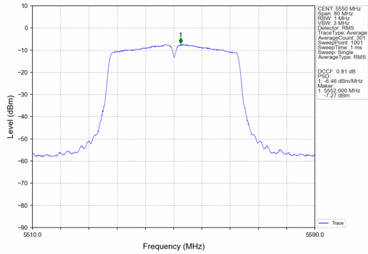
802.11ac(VHT40)_MCH_5550MHz_MIMO_NTNV
