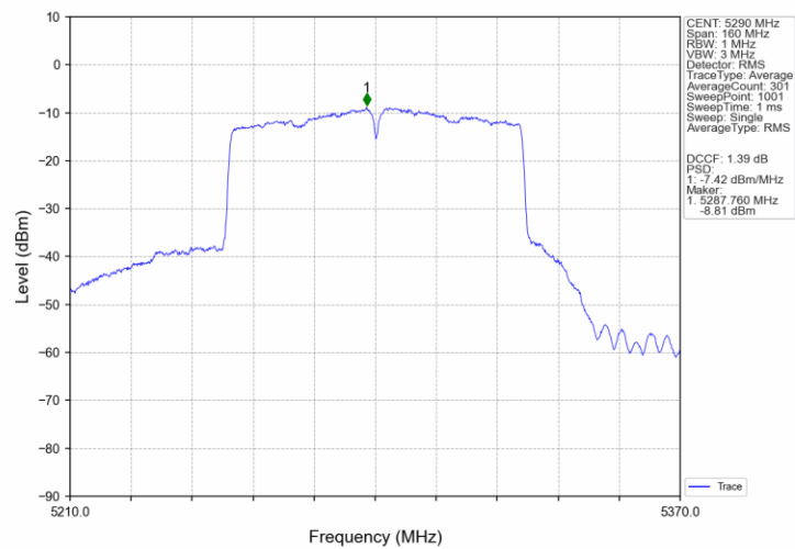
802.11ac(VHT80)_MCH_5290MHz_Ant3_NTNV
