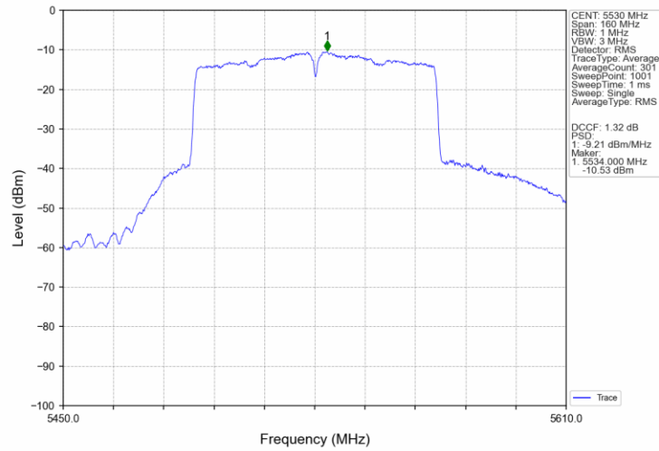
802.11ac(VHT80)_LCH_5530MHz_Ant3_NTNV
