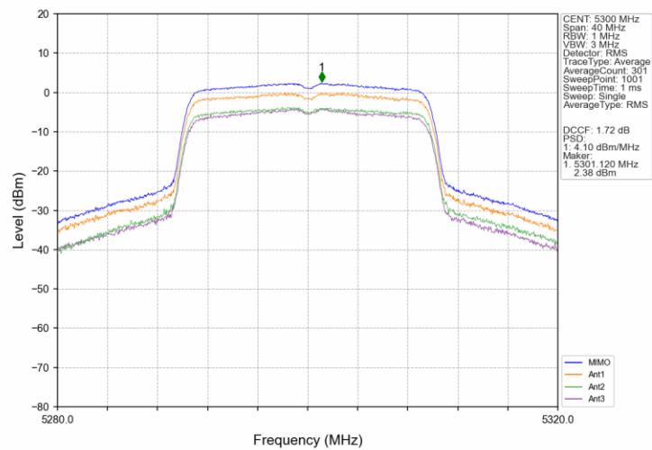
802.11ax(HEW20)_MCH_5300MHz_SU_/_MIMO_NTNV
