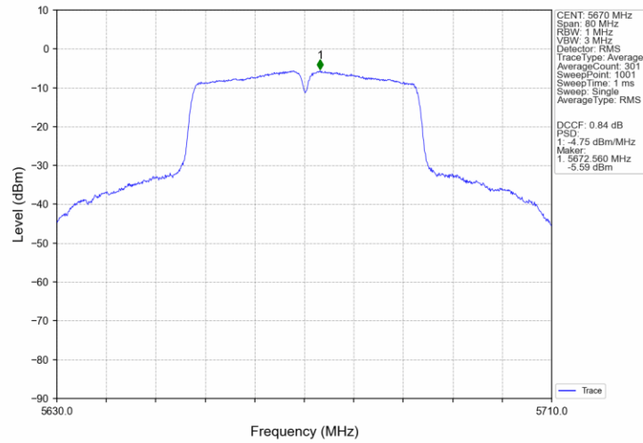
802.11ac(VHT40)_HCH_5670MHz_Ant3_NTNV
