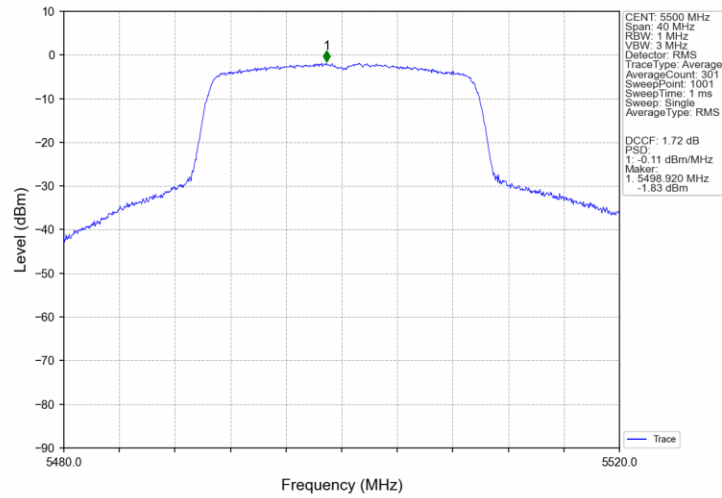
802.11ax(HEW20)_LCH_5500MHz_SU_ / _Ant3_NTNV
