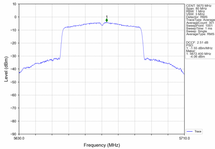
802.11ax(HEW40)_HCH_5670MHz_SU_/_Ant3_NTNV
