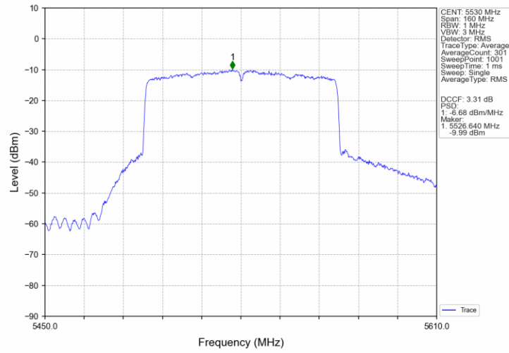
802.11ax(HEW80)_LCH_5530MHz_SU_/_MIMO NTN
