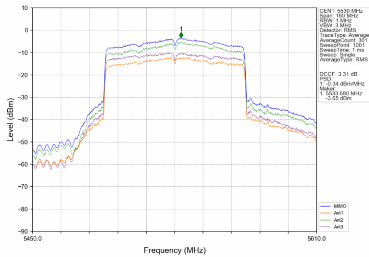
802.11ax(HEW80)_LCH_5530MHz_SU_/_MIMO NTN
