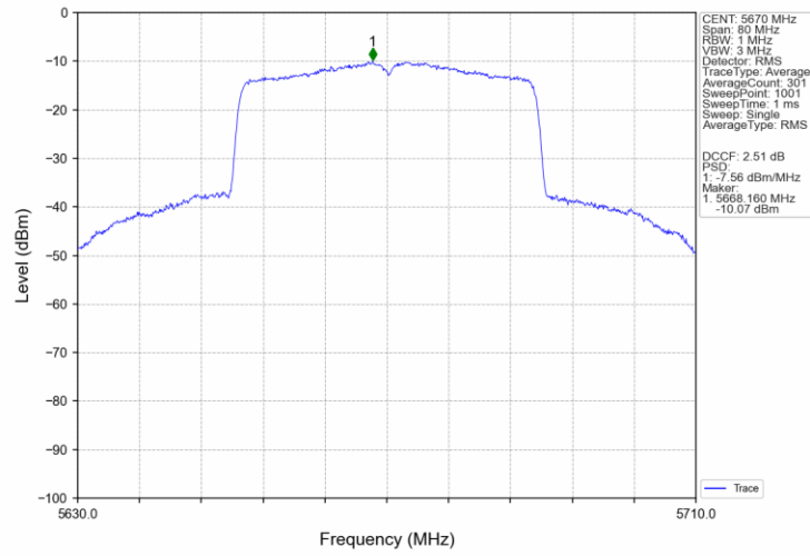
802.11ax(HEW40)_HCH_5670MHz_SU_/_Ant3_NTNV
