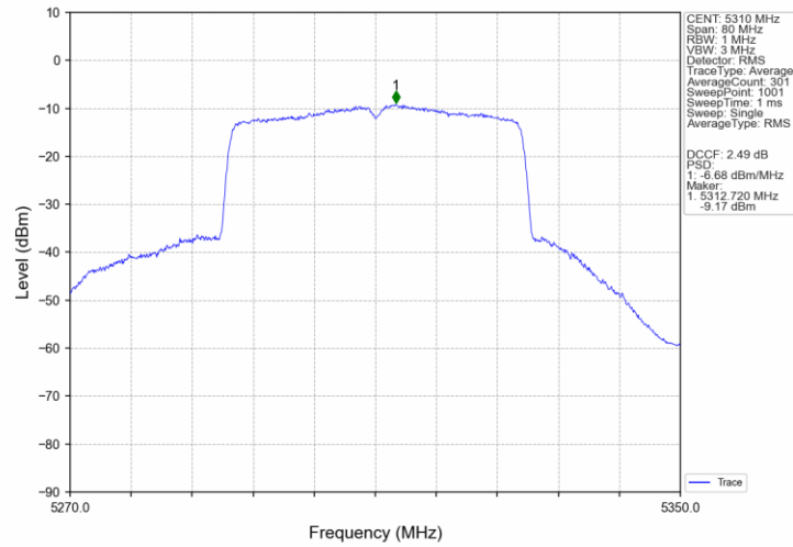
802.11ax(HEW40)_HCH_5310MHz_SU_/_MIMO_NTNV
