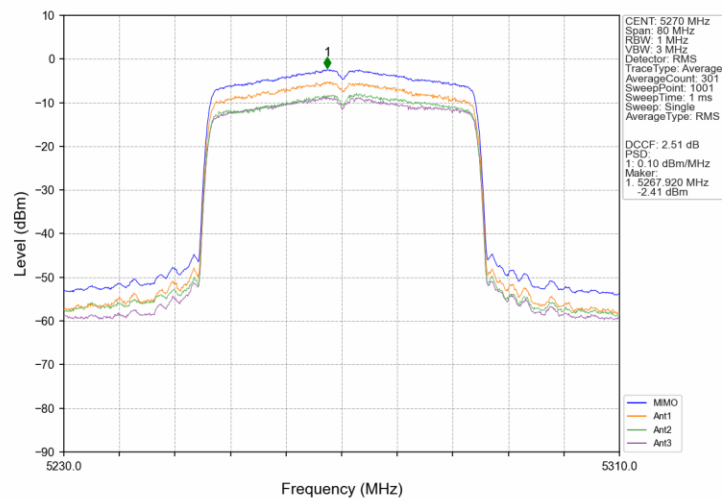
802.11ax(HEW40)_LCH_5270MHz_SU_/_MIMO NTN
