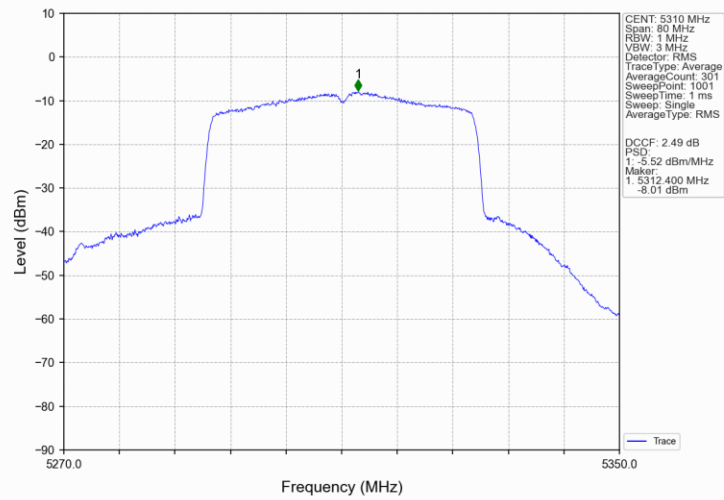
802.11ax(HEW40)_HCH_5310MHz_SU_/_Ant3_NTNV
