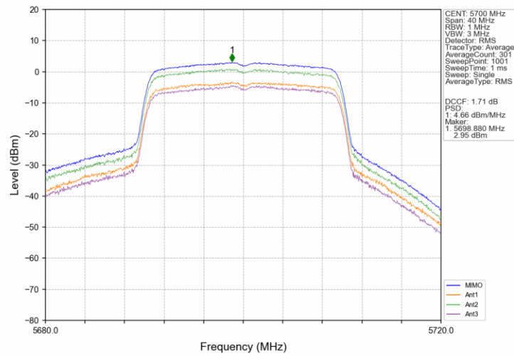
802.11ax(HEW20)_HCH_5700MHz_SU_/_MIMO_NTNV
