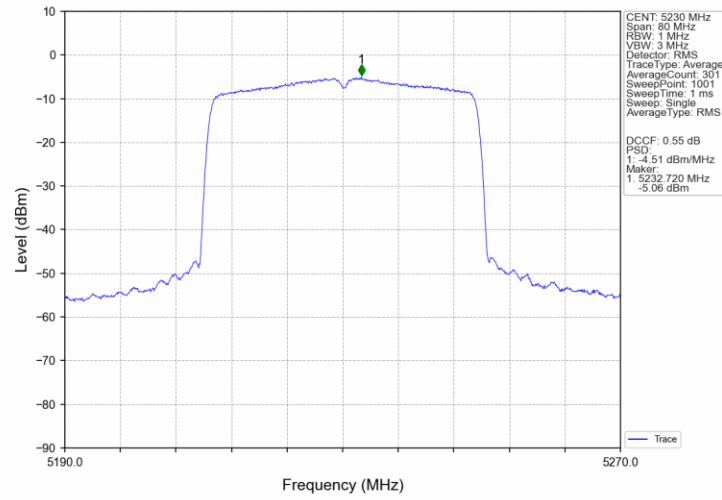
802.11ax(HEW40)_HCH_5230MHz_SU_/_MIMO_NTNV
