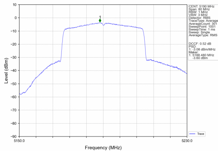
802.11ax(HEW40)_LCH_5190MHz_SU_ / _Ant3_NTNV
