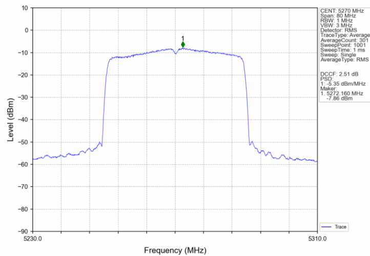
802.11ax(HEW40)_LCH_5270MHz_SU_ / _Ant3_NTNV
