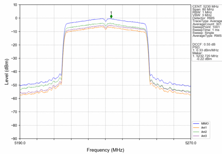
802.11ax(HEW40)_HCH_5230MHz_SU_/_MIMO_NTNV
