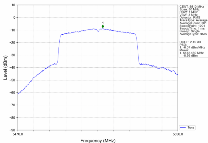
802.11ax(HEW40)_LCH_5510MHz_SU_ / _Ant3_NTNV
