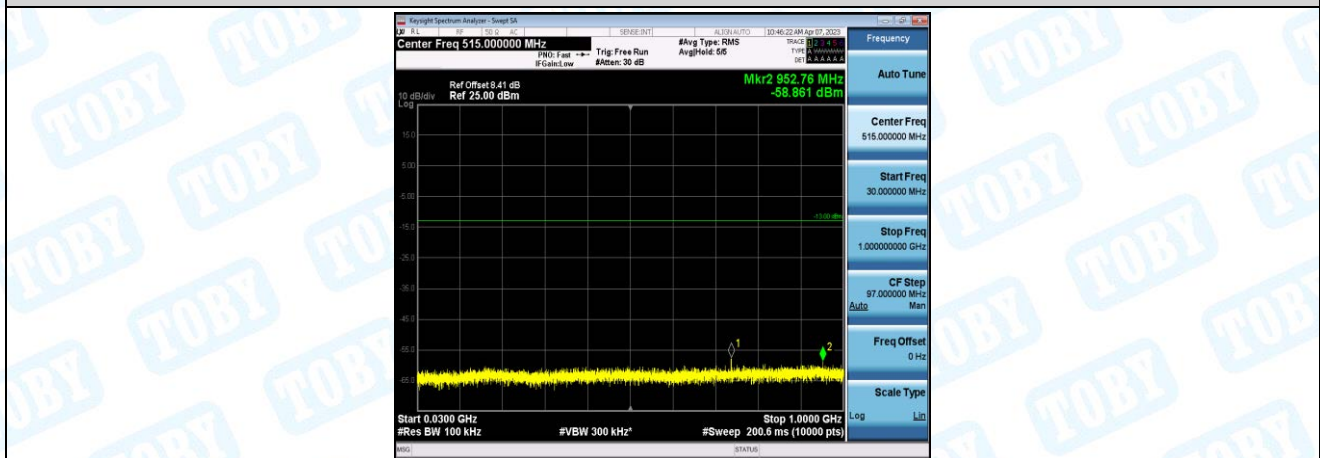
Band17-Stand-Alone-NaN-QPSK-23831-12@0-15kHz-30-1000-30~1000MHz@-58.86dBm--13-PASS
