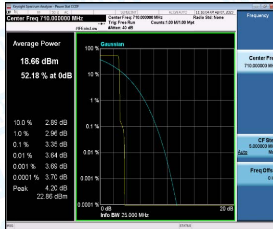
Band17-Stand-Alone-NaN-QPSK-23790-1@47-3.75kHz-3.35-<=13-PASS
