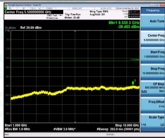
Band26-Stand-Alone-NaN-QPSK-26740-12@0-15kHz-1000-10000-1000-10000MHz@-39.4dBm--13-PASS
