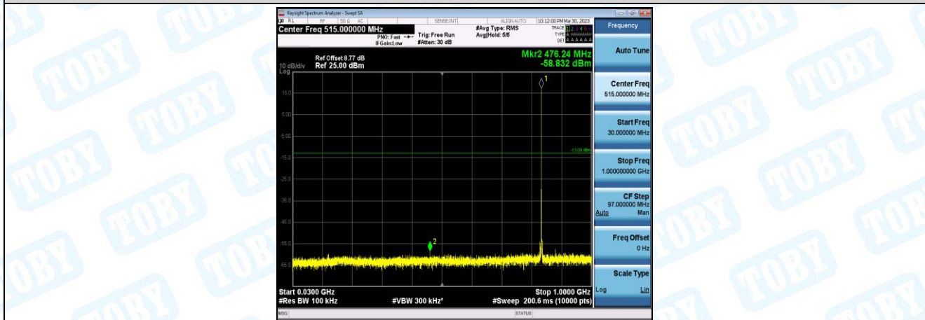
Band26-Stand-Alone-NaN-BPSK-26915-1@11-15kHz-30-1000-30~1000MHz@-58.83dBm--13-PASS
