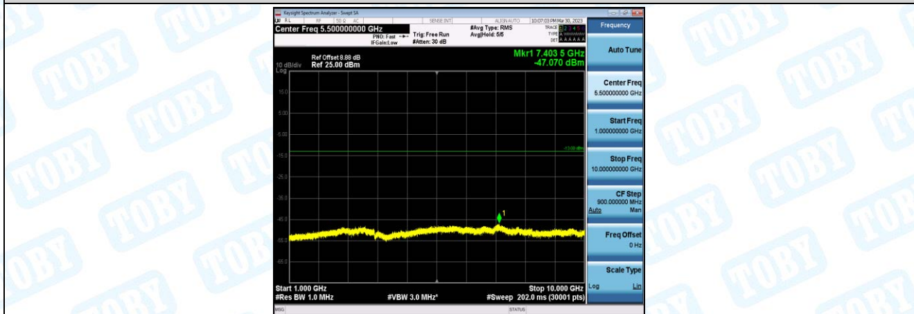
Band26-Stand-Alone-NaN-QPSK-27039-12@0-15kHz-1000-10000-1000~10000MHz@-47.07dBm--13-PAS
