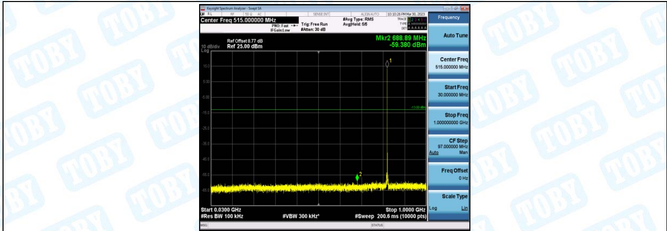
Band26-Stand-Alone-NaN-BPSK-26791-1@11-15kHz-30-1000-30~1000MHz@-59.38dBm--13-PASS
