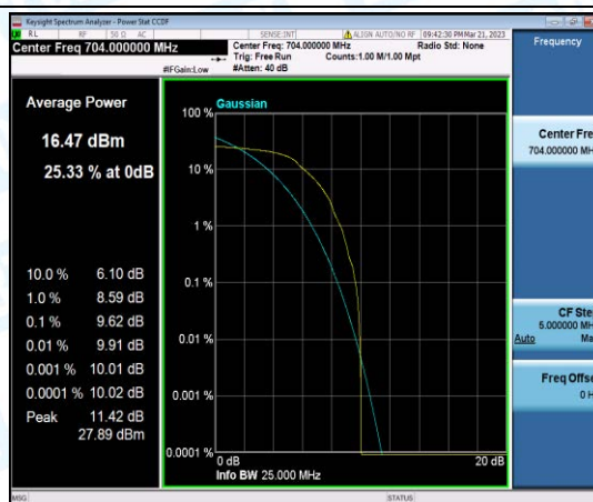
Band12-10MHz-QPSK-23060-1-0-Low-9.62-<=13-PASS
