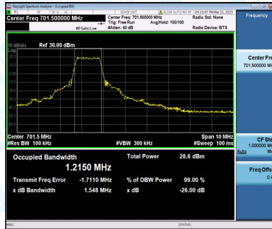
Band12-5MHz-16QAM-23035-6-0-Low-1.2150-1.548-PASS
