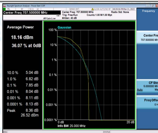
Band12-1.4MHz-QPSK-23095-1-0-Low-7.85-<=13-PASS
