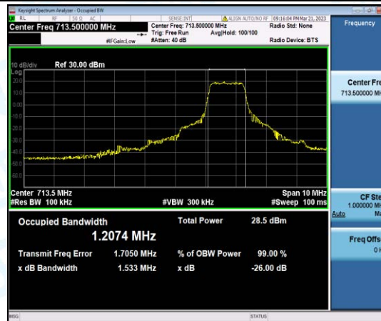
Band12-5MHz-QPSK-23155-6-0-High-1.2074-1.533-PASS
