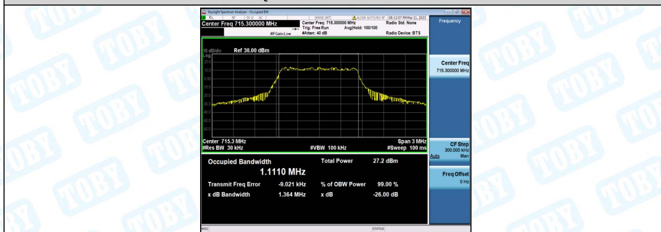
Band12-1.4MHz-QPSK-23173-6-0-High-1.1110-1.364-PASS
