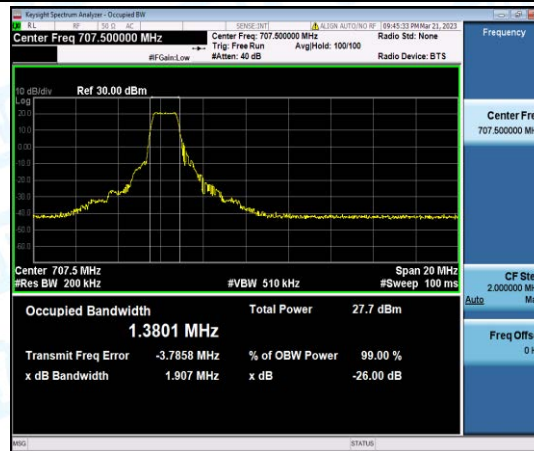
Band12-10MHz-16QAM-23095-6-0-Low-1.3801-1.907-PASS
