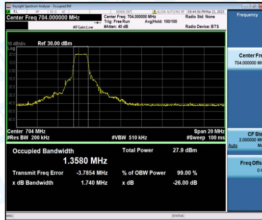
Band12-10MHz-16QAM-23060-6-0-Low-1.3580-1.740-PASS
