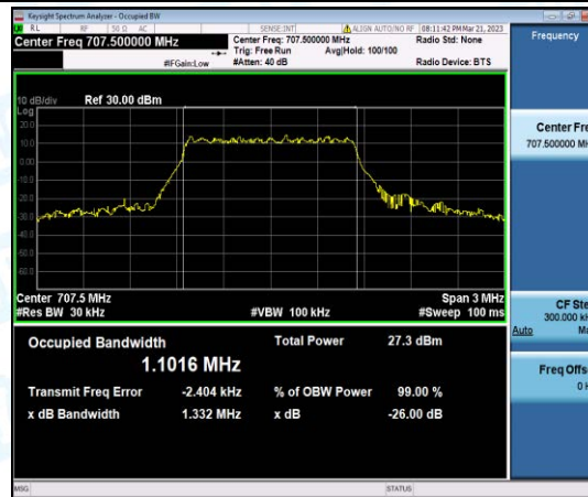
Band12-1.4MHz-16QAM-23095-6-0-Low-1.1016-1.332-PASS
