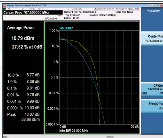
Band12-10MHz-16QAM-23095-6-0-Low-9.31-<=13-PASS
