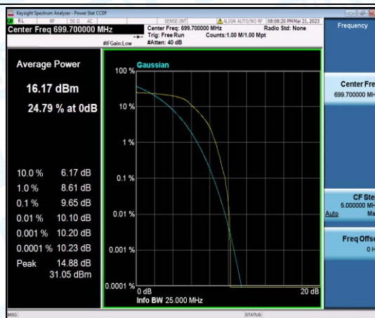
Band12-1.4MHz-QPSK-23017-1-0-Low-9.65-<=13-PASS
