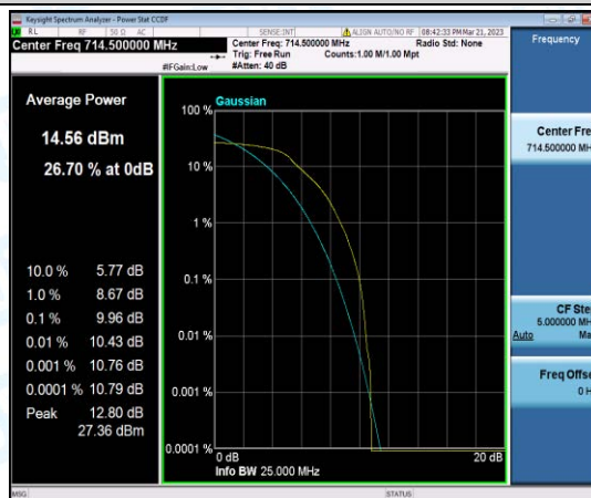
Band12-3MHz-QPSK-23165-6-0-High-9.96-<=13-PASS
