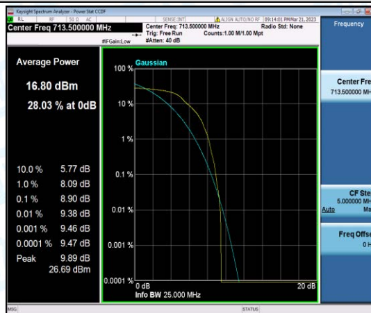
Band12-5MHz-QPSK-23155-1-0-High-8.90-<=13-PASS
