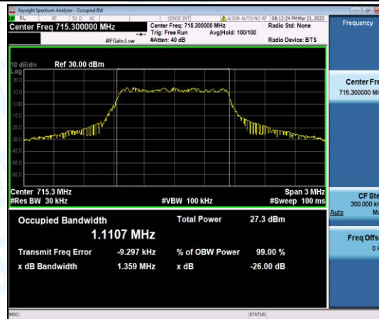
Band12-1.4MHz-16QAM-23173-6-0-High-1.1107-1.359-PASS
