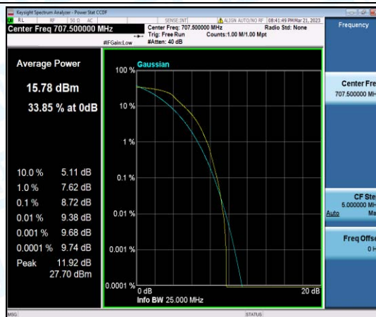
Band12-3MHz-QPSK-23095-6-0-Low-8.72-<=13-PASS
