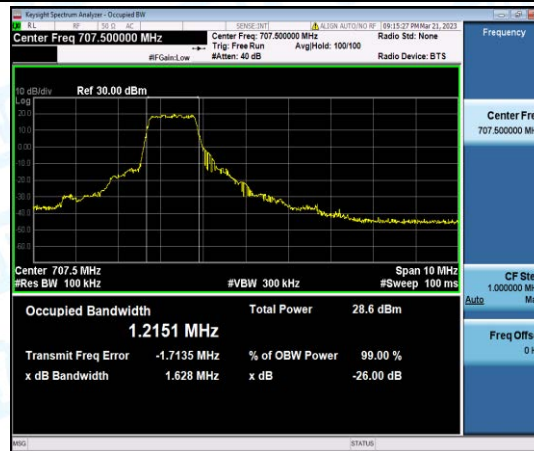
Band12-5MHz-QPSK-23095-6-0-Low-1.2151-1.628-PASS
