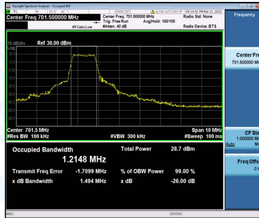
Band12-5MHz-QPSK-23035-6-0-Low-1.2148-1.494-PASS
