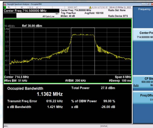
Band12-3MHz-QPSK-23165-6-0-High-1.1362-1.421-PASS
