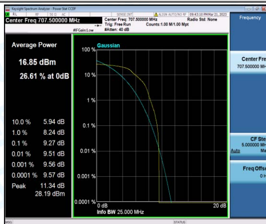
Band12-10MHz-QPSK-23095-1-0-Low-9.27-<=13-PASS
