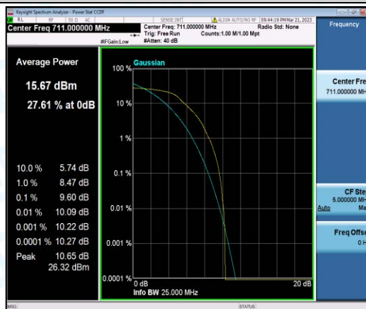
Band12-10MHz-16QAM-23130-6-0-High-9.60-<=13-PASS
