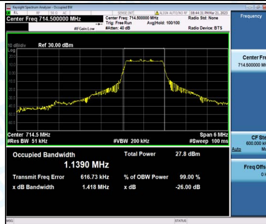
Band12-3MHz-16QAM-23165-6-0-High-1.1390-1.418-PASS
