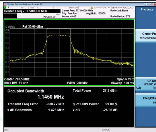
Band12-3MHz-QPSK-23095-6-0-Low-1.1450-1.428-PASS
