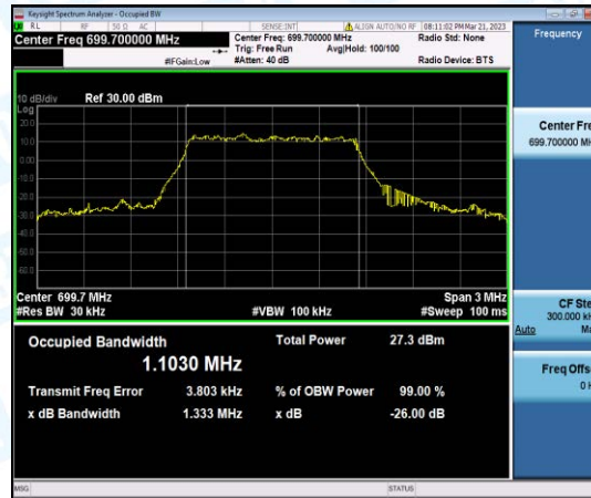
Band12-1.4MHz-16QAM-23017-6-0-Low-1.1030-1.333-PASS
