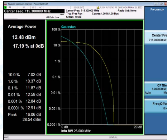
Band12-1.4MHz-16QAM-23173-6-0-High-11.87-<=13-PASS
