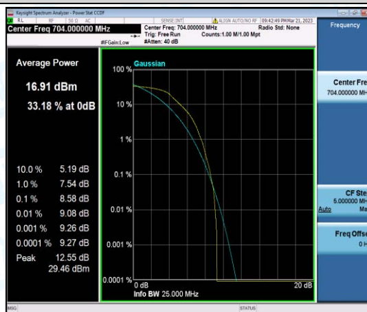
Band12-10MHz-QPSK-23060-6-0-Low-8.58-<=13-PASS
