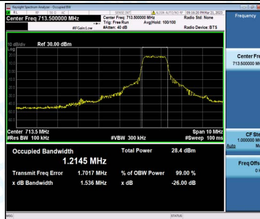
Band12-5MHz-16QAM-23155-6-0-High-1.2145-1.536-PASS
