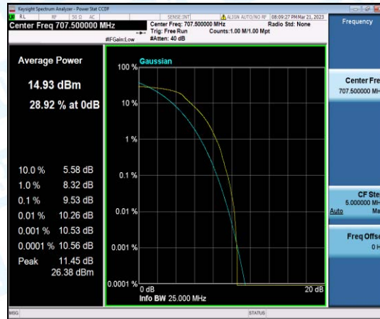
Band12-1.4MHz-QPSK-23095-6-0-Low-9.53-<=13-PASS
