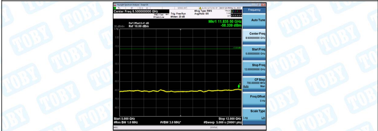
Band12-3MHz-16QAM-23165-1-0-High-5000-12000--58.34-PASS
