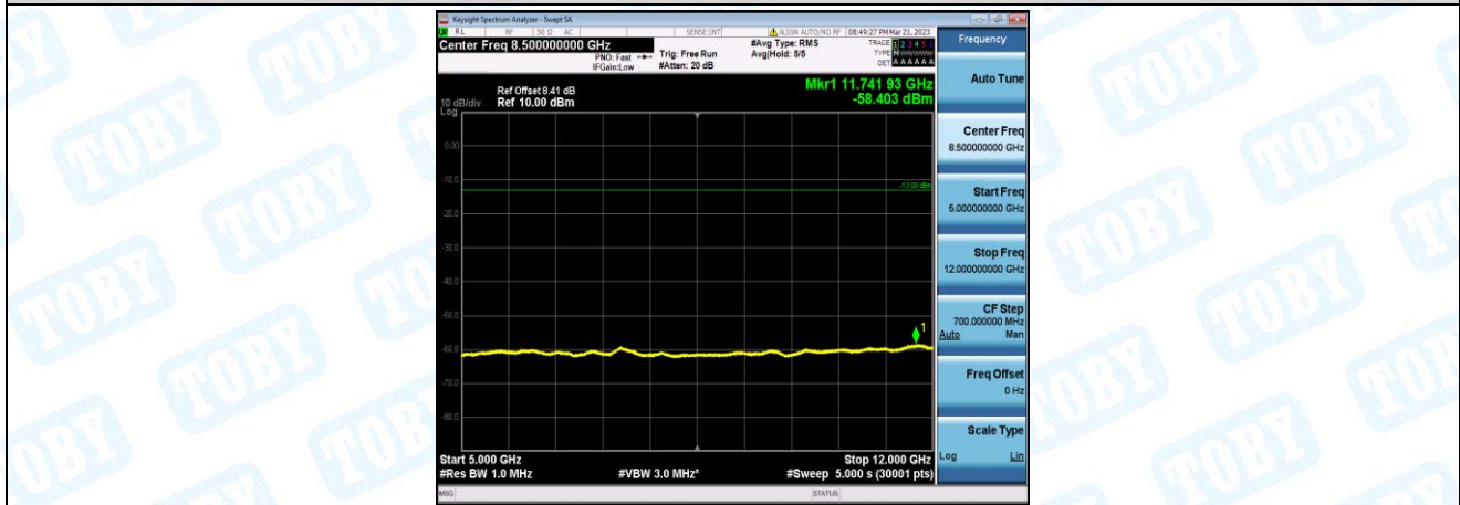
Band12-3MHz-16QAM-23025-1-0-Low-5000-12000--58.4-PASS
