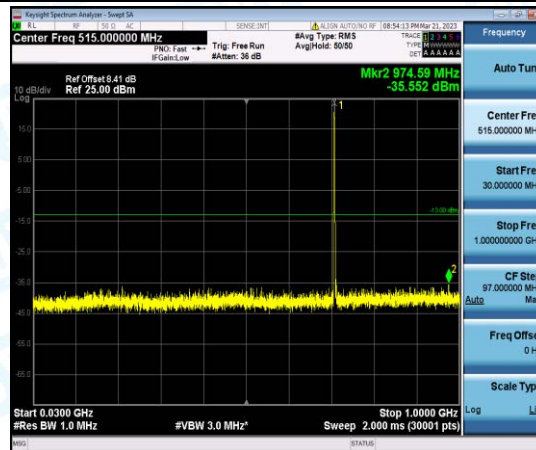
Band12-3MHz-QPSK-23165-1-0-High-30-1000--35.55-PASS
