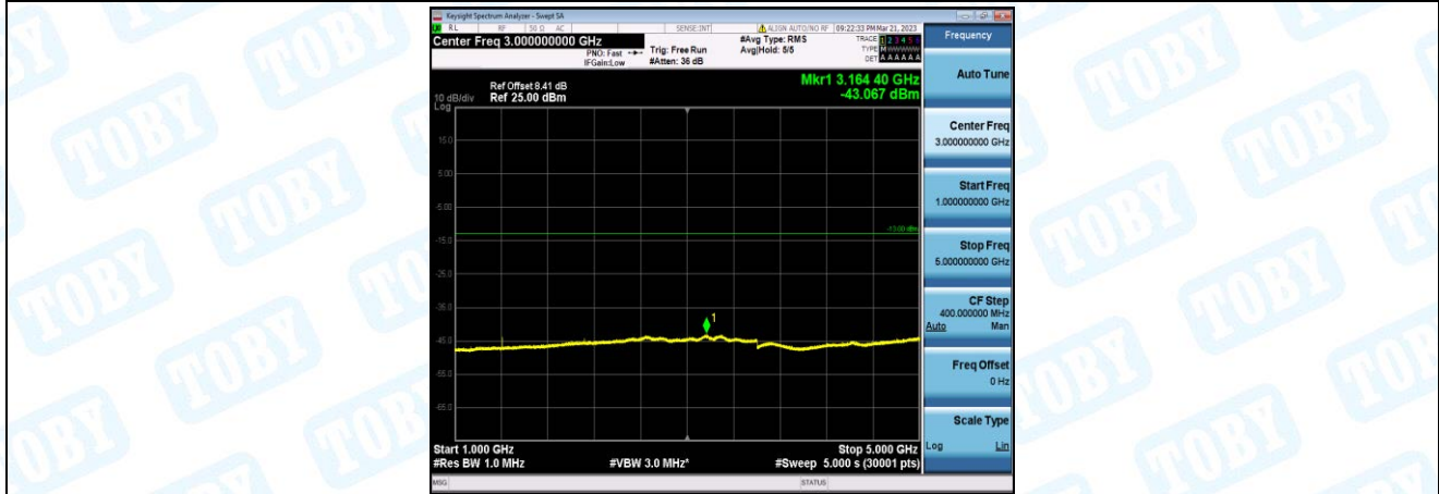
Band12-5MHz-QPSK-23095-1-0-Low-1000-5000--43.07-PASS
