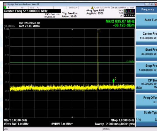
Band12-3MHz-16QAM-23165-1-0-High-30-1000--36.12-PASS
