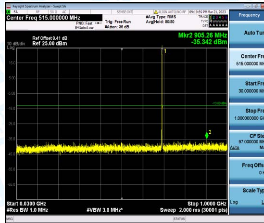
Band12-5MHz-16QAM-23035-1-0-Low-30-1000--35.34-PASS
