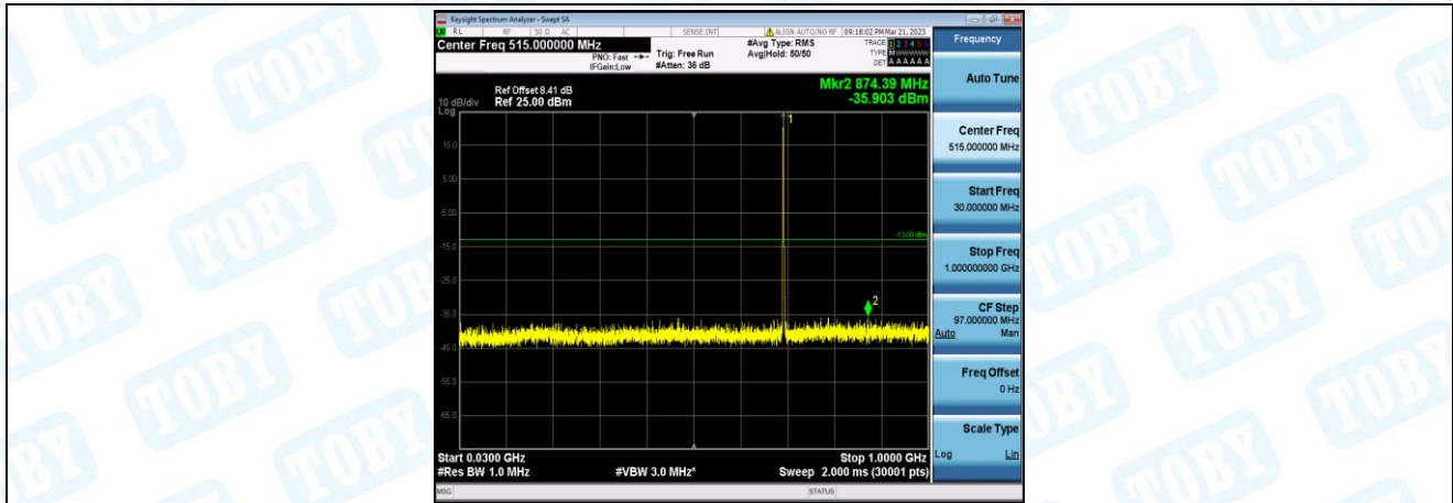
Band12-5MHz-QPSK-23035-1-0-Low-30-1000--35.9-PASS
