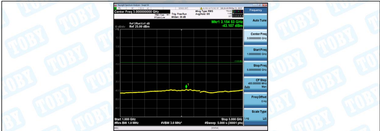
Band12-1.4MHz-16QAM-23173-1-0-High-1000-5000--43.11-PASS
