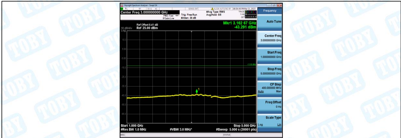
Band12-3MHz-QPSK-23165-1-0-High-1000-5000--43.29-PASS
