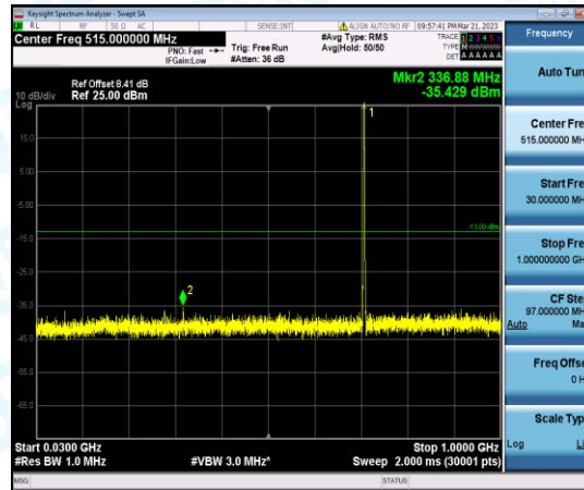
Band12-10MHz-16QAM-23130-1-0-High-30-1000--35.43-PASS
