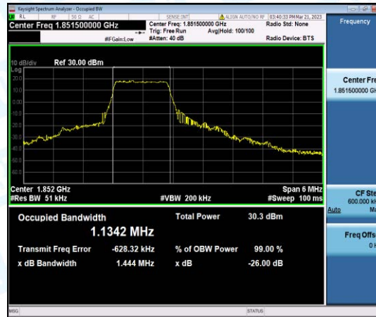
Band2-3MHz-QPSK-18615-6-0-Low-1.1342-1.444-PASS
