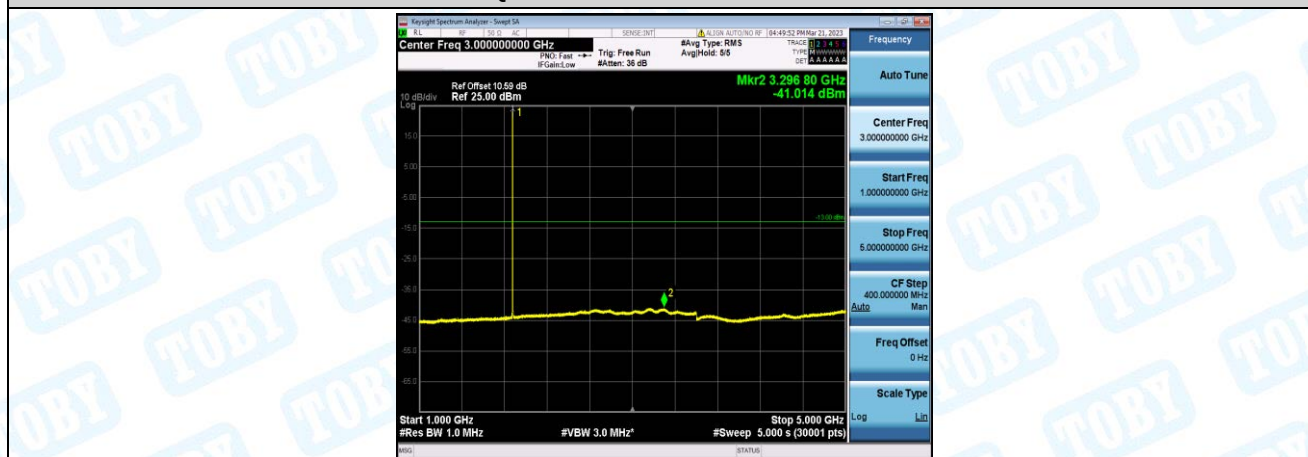
Band2-10MHz-QPSK-18900-1-0-Low-1000-5000--41.01-PASS
