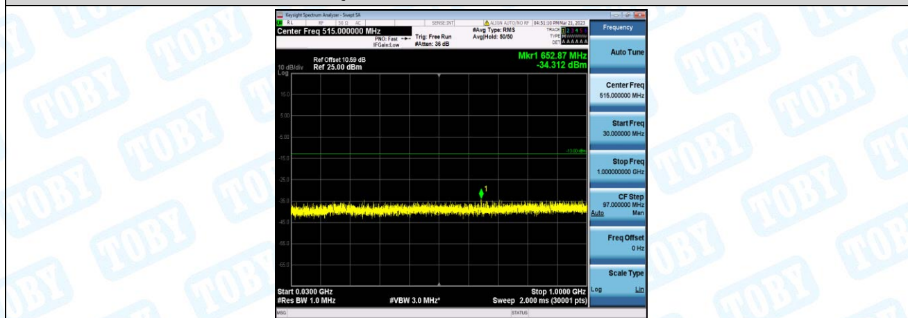
Band2-10MHz-16QAM-18900-1-0-Low-30-1000--34.31-PASS
