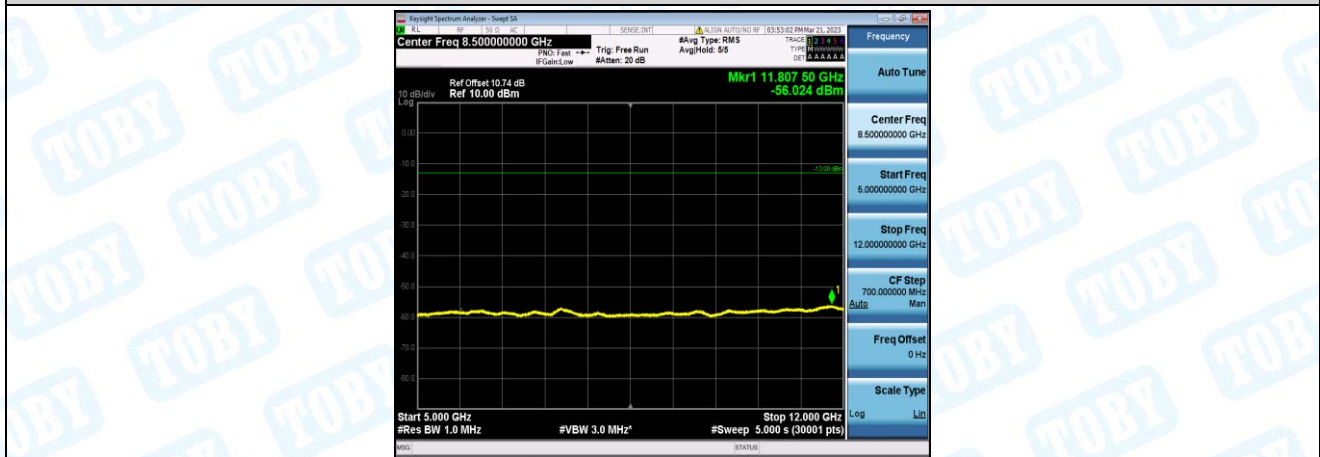
Band2-3MHz-QPSK-19185-1-0-High-5000-12000--56.02-PASS
