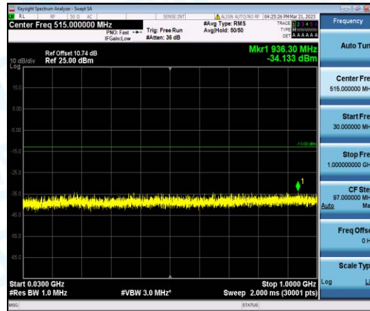
Band2-5MHz-16QAM-19175-1-0-High-30-1000--34.13-PASS
