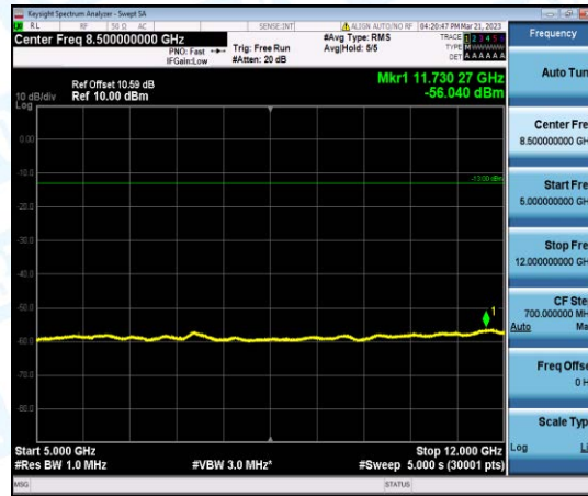
Band2-5MHz-QPSK-18900-1-0-Low-5000-12000--56.04-PASS
