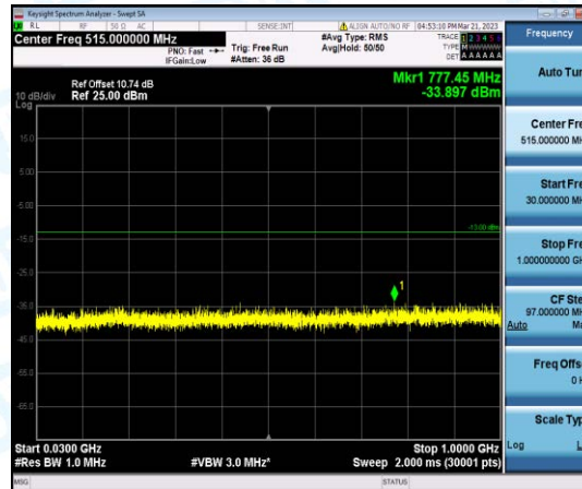
Band2-10MHz-QPSK-19150-1-0-High-30-1000--33.9-PASS
