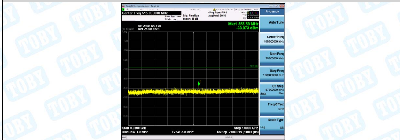
Band2-10MHz-16QAM-19150-1-0-High-30-1000--33.07-PASS
