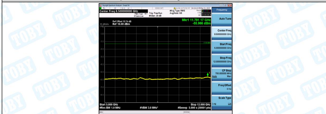
Band2-5MHz-QPSK-19175-1-0-High-5000-12000--55.97-PASS
