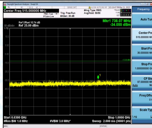
Band2-1.4MHz-QPSK-19193-1-0-High-30-1000--34.06-PASS
