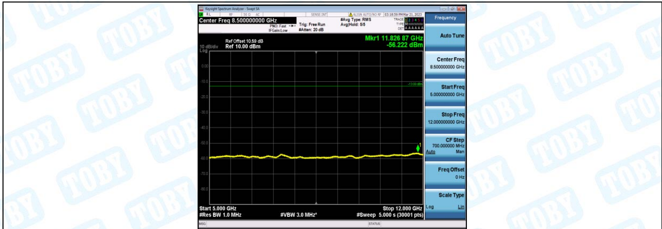
Band2-1.4MHz-16QAM-18900-1-0-Low-5000-12000--56.22-PASS
