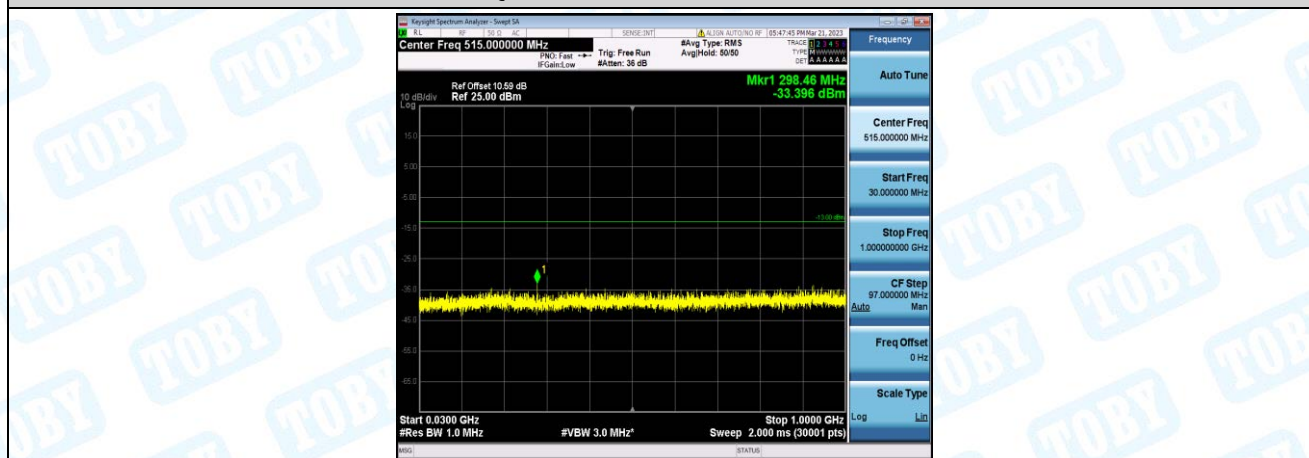
Band2-20MHz-16QAM-18900-1-0-Low-30-1000--33.4-PASS
