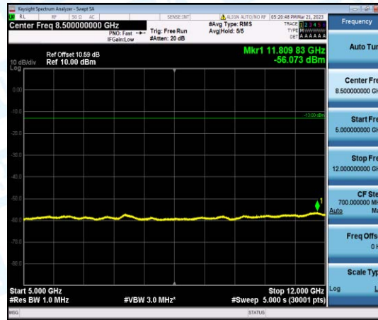
Band2-15MHz-16QAM-18900-1-0-Low-5000-12000--56.07-PASS
