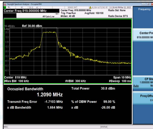
Band26-5MHz-QPSK-26740-6-0-Low-1.2090-1.664-PASS
