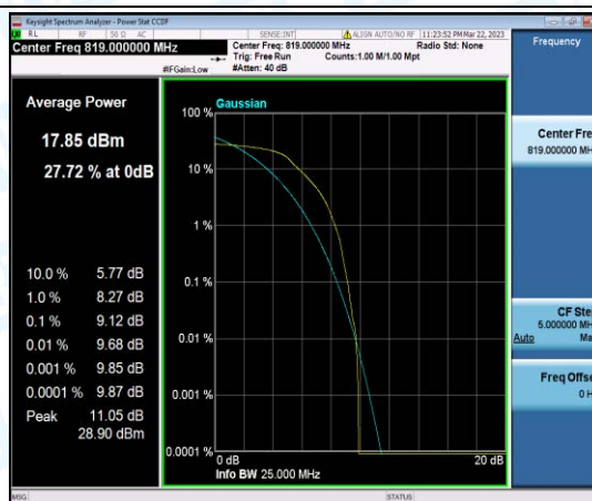
Band26-5MHz-QPSK-26740-6-0-Low-9.12-13-PASS
