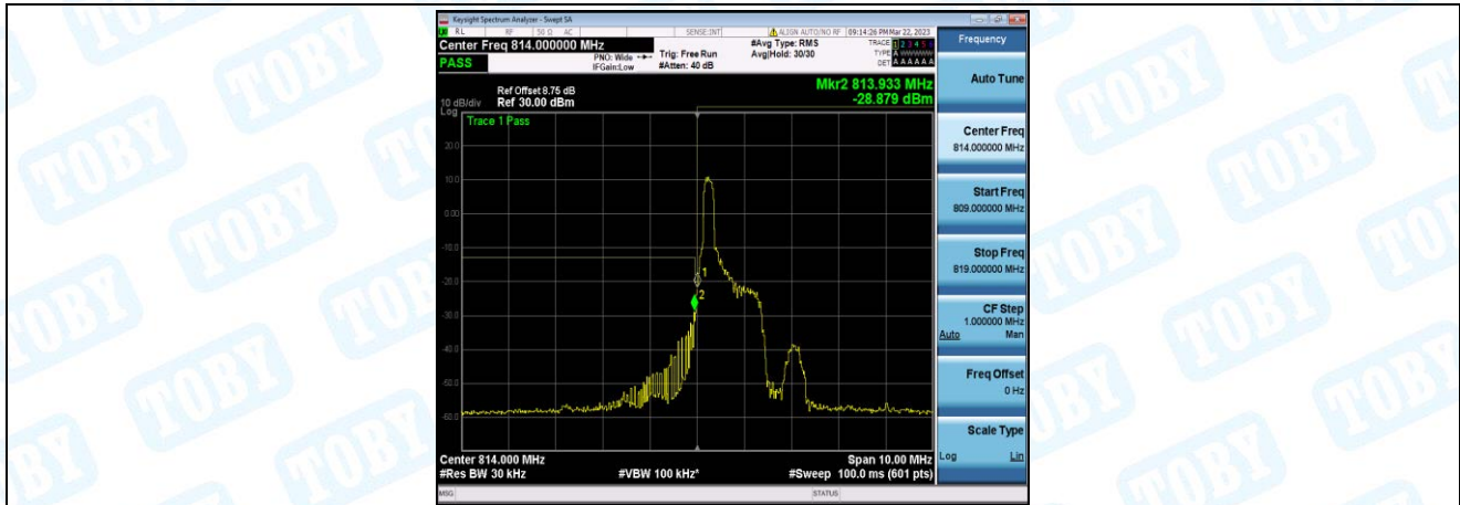
Band26-1.4MHz-16QAM-26697-1-0-Low--22.25,-28.88-PASS
