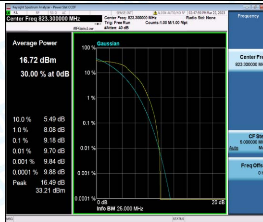
Band26-1.4MHz-16QAM-26783-6-0-High-9.18-<=13-PASS
