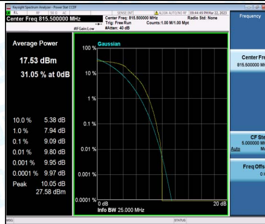
Band26-3MHz-16QAM-26705-6-0-Low-9.09-<=13-PASS
