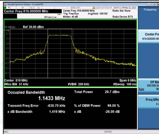
Band26-3MHz-QPSK-26740-6-0-Low-1.1433-1.419-PASS
