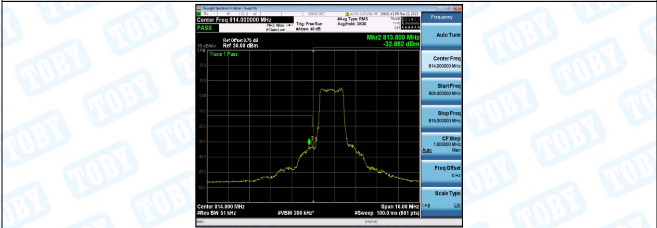
Band26-3MHz-QPSK-26705-6-0-Low--33.52,-32.86-PASS
