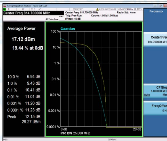
Band26-1.4MHz-QPSK-26697-1-0-Low-10.41-<=13-PASS
