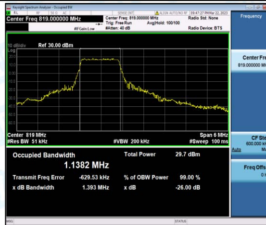
Band26-3MHz-16QAM-26740-6-0-Low-1.1382-1.393-PASS
