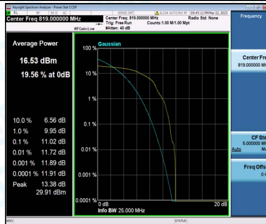
Band26-3MHz-16QAM-26740-1-0-Low-11.02-<=13-PASS
