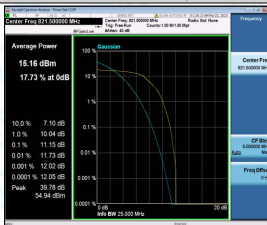
Band26-5MHz-QPSK-26765-6-0-High-11.15-13-PASS
