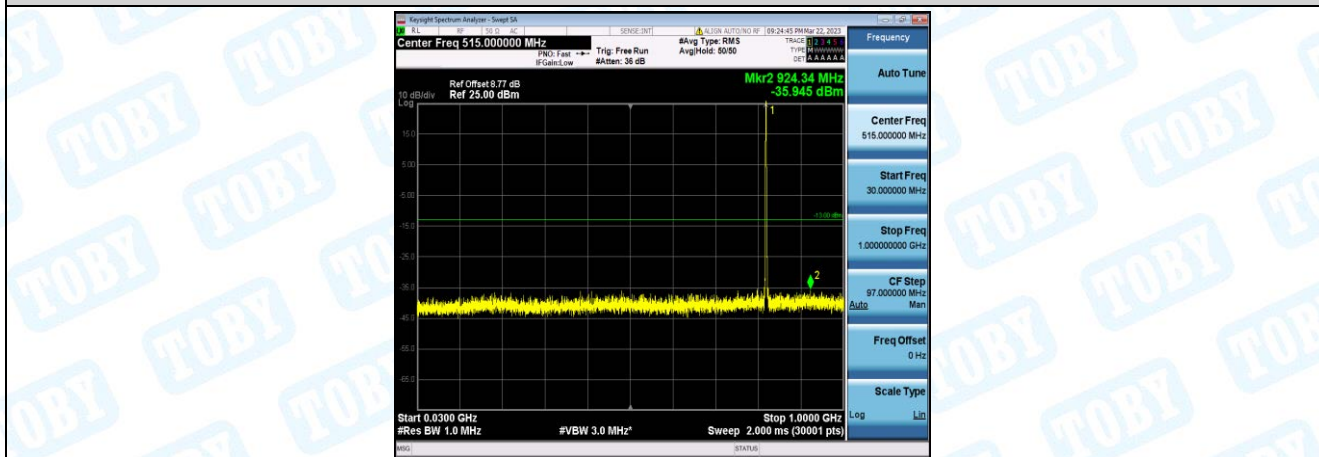
Band26-1.4MHz-QPSK-26783-1-0-High-30-1000--35.95-PASS
