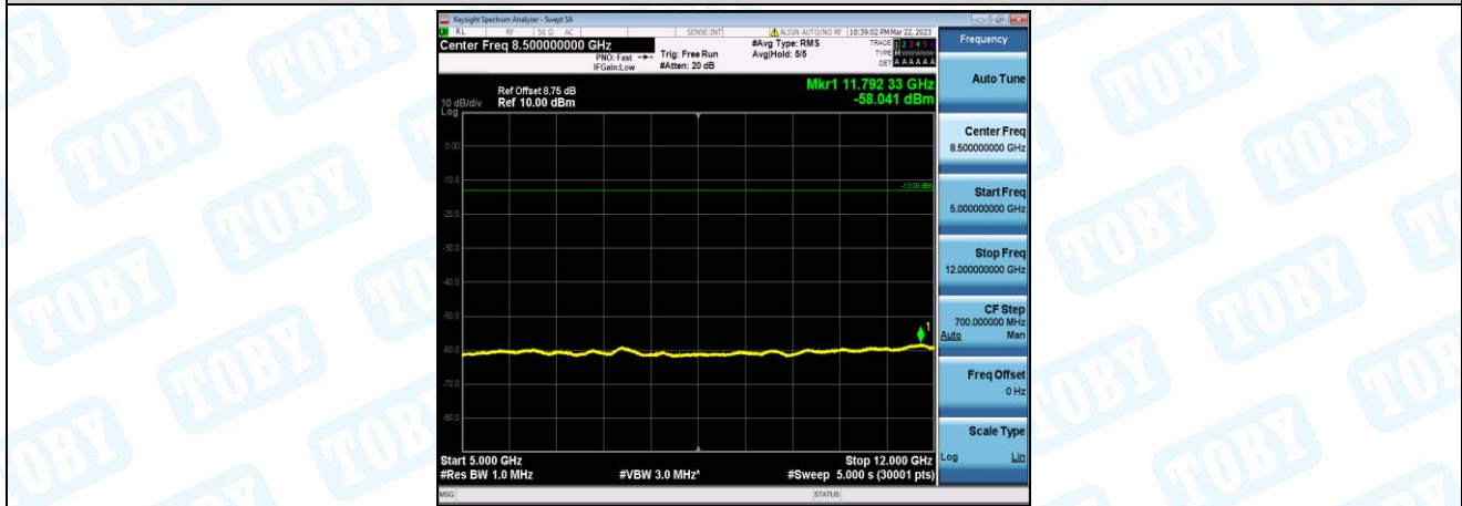
Band26-3MHz-16QAM-26705-1-0-Low-5000-12000--58.04-PASS
