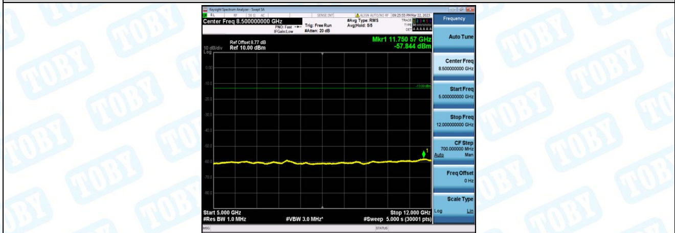
Band26-1.4MHz-QPSK-26783-1-0-High-5000-12000--57.84-PASS
