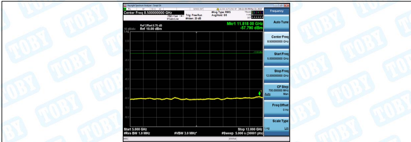
Band26-1.4MHz-QPSK-26740-1-0-Low-5000-12000--57.79-PASS
