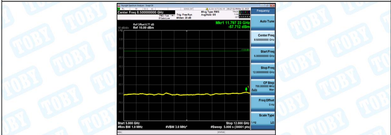
Band26-1.4MHz-16QAM-26783-1-0-High-5000-12000--57.71-PASS
