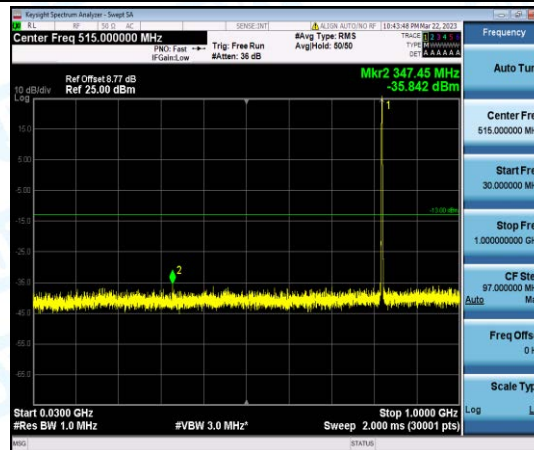
Band26-3MHz-QPSK-26775-1-0-High-30-1000--35.84-PASS
