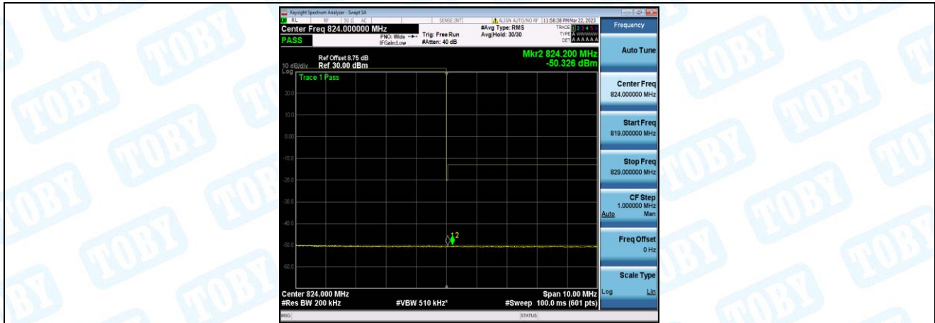
Band26-10MHz-QPSK-26740-1-0-Low--50.51,-50.33-PASS
