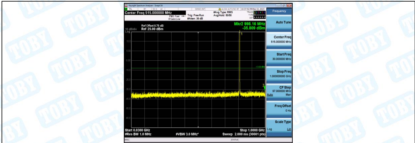
Band26-3MHz-16QAM-26705-1-0-Low-30-1000--35.81-PASS
