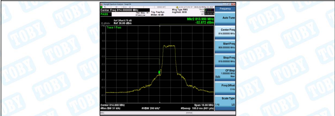
Band26-3MHz-16QAM-26705-6-0-Low--33.92,-32.87-PASS
