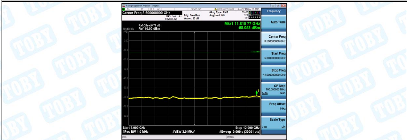
Band26-3MHz-QPSK-26775-1-0-High-5000-12000--58.05-PASS
