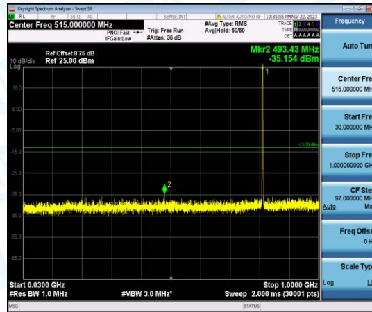
Band26-3MHz-QPSK-26705-1-0-Low-30-1000--35.15-PASS
