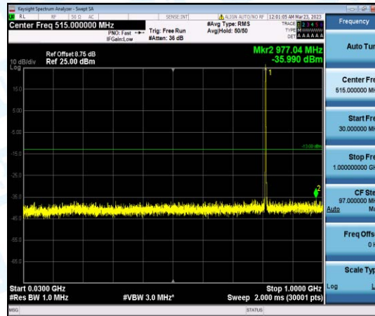
Band26-5MHz-QPSK-26715-1-0-Low-30-1000--35.99-PASS
