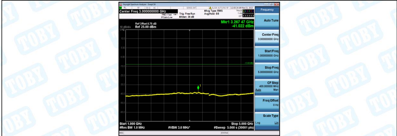
Band26-5MHz-QPSK-26740-1-0-Low-1000-5000--41.02-PASS
