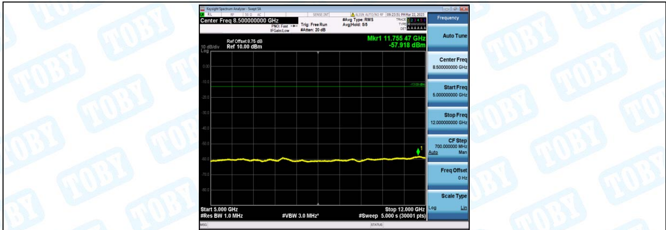
Band26-1.4MHz-16QAM-26740-1-0-Low-5000-12000--57.92-PASS
