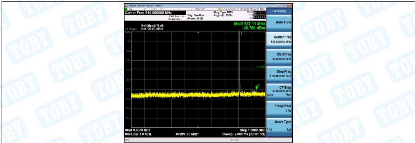
Band26-1.4MHz-16QAM-26697-1-0-Low-30-1000--35.78-PASS
