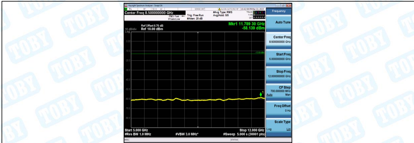
Band26-3MHz-16QAM-26740-1-0-Low-5000-12000--58.14-PASS
