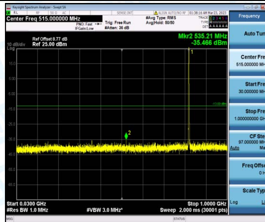
Band26-5MHz-QPSK-26765-1-0-High-30-1000--35.47-PASS
