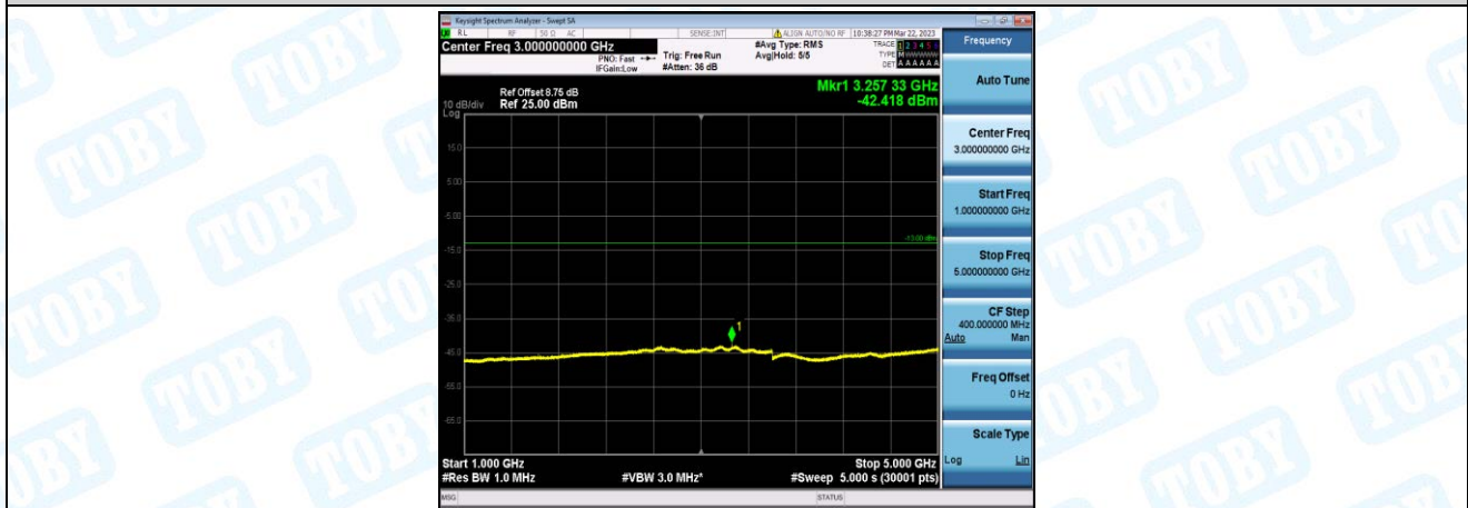
Band26-3MHz-16QAM-26705-1-0-Low-1000-5000--42.42-PASS
