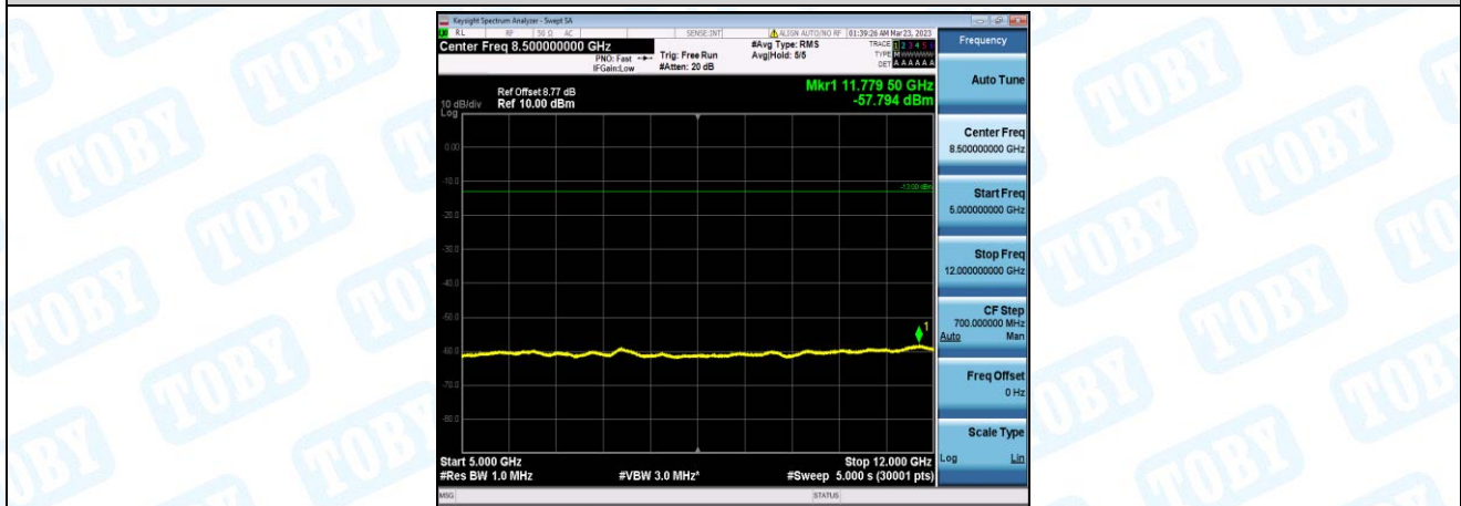
Band26-5MHz-QPSK-26765-1-0-High-5000-12000--57.79-PASS
