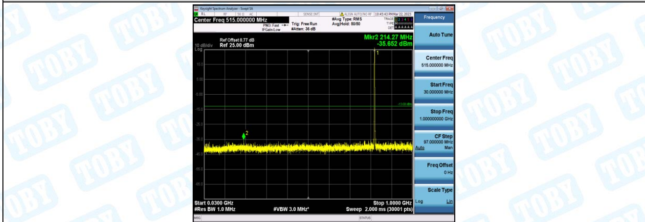
Band26-3MHz-16QAM-26775-1-0-High-30-1000--35.65-PASS
