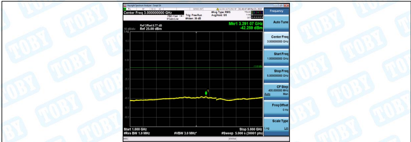
Band26-5MHz-16QAM-26765-1-0-High-1000-5000--42.26-PASS
