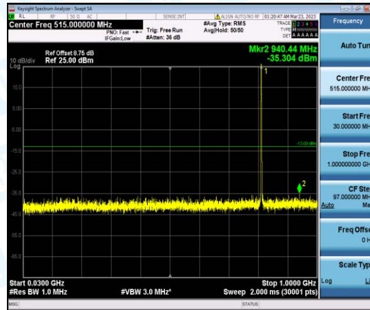
Band26-10MHz-QPSK-26740-1-0-Low-30-1000--35.3-PASS
