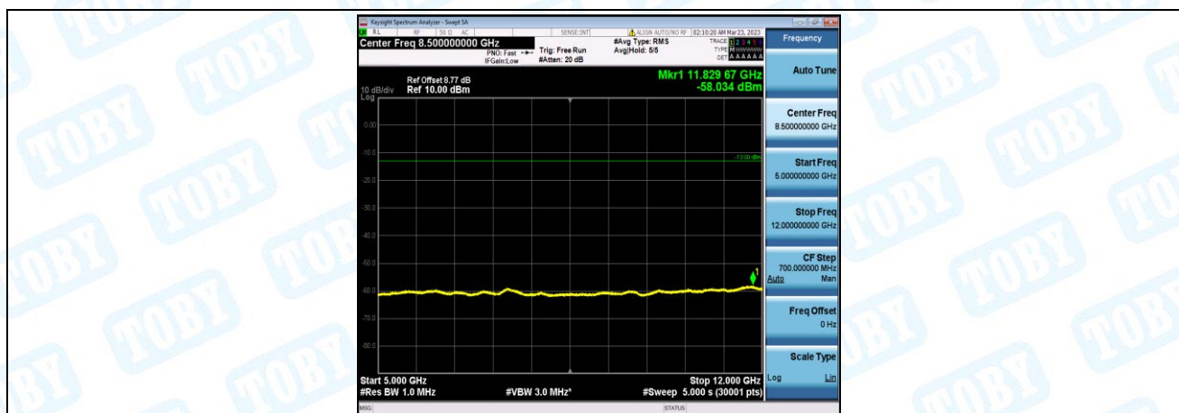
Band26-1.4MHz-QPSK-26915-1-0-Low-5000-12000--58.03-PASS
