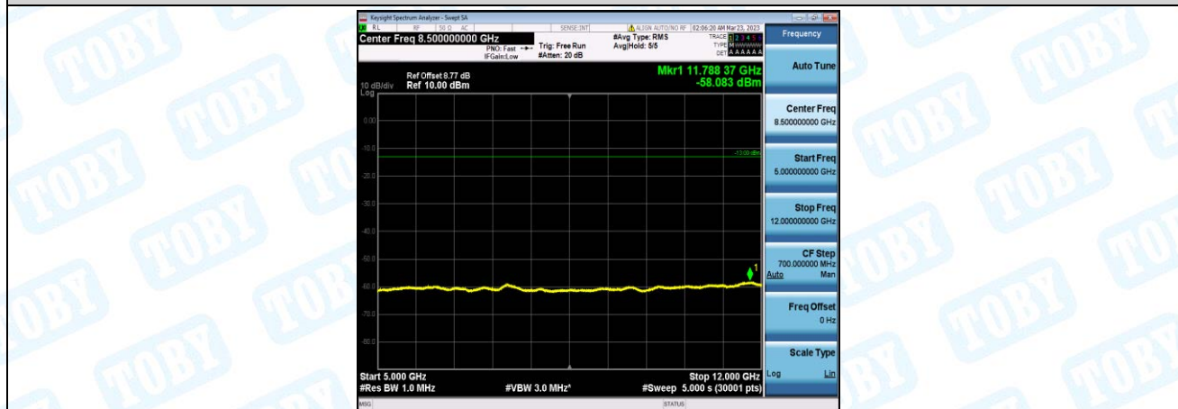
Band26-1.4MHz-QPSK-26797-1-0-Low-5000-12000--58.08-PASS
