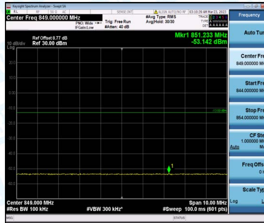
Band26-5MHz-QPSK-26915-6-0-Low--53.14-PASS
