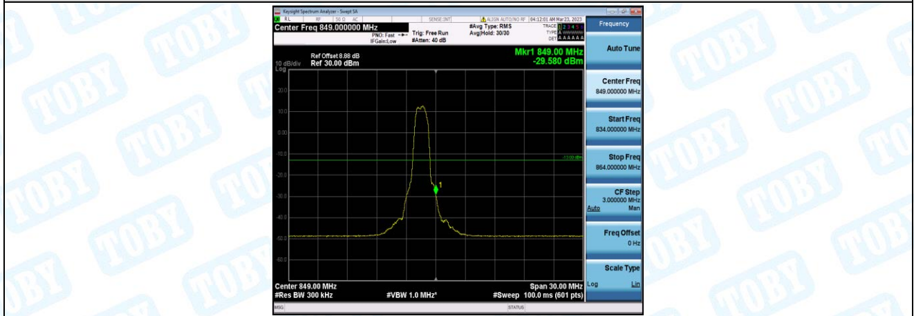
Band26-15MHz-16QAM-26965-6-0-High--29.58-PASS
