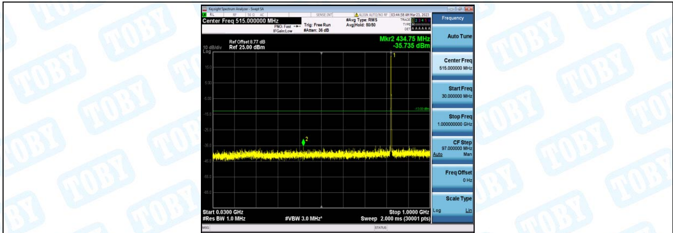
Band26-10MHz-16QAM-26840-1-0-Low-30-1000--35.74-PASS
