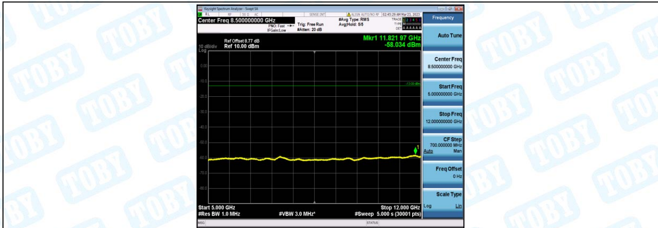
Band26-3MHz-16QAM-26915-1-0-Low-5000-12000--58.03-PASS
