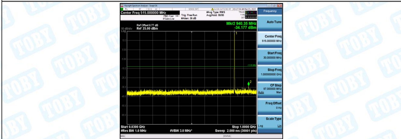
Band26-5MHz-16QAM-26915-1-0-Low-30-1000--34.18-PASS
