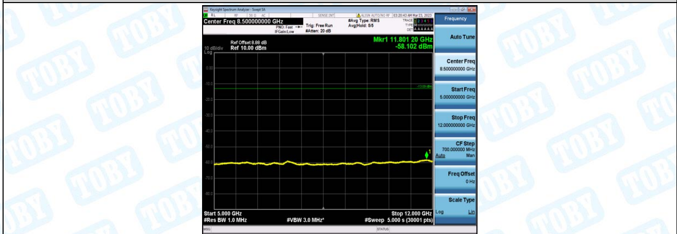
Band26-5MHz-QPSK-27015-1-0-High-5000-12000--58.1-PASS
