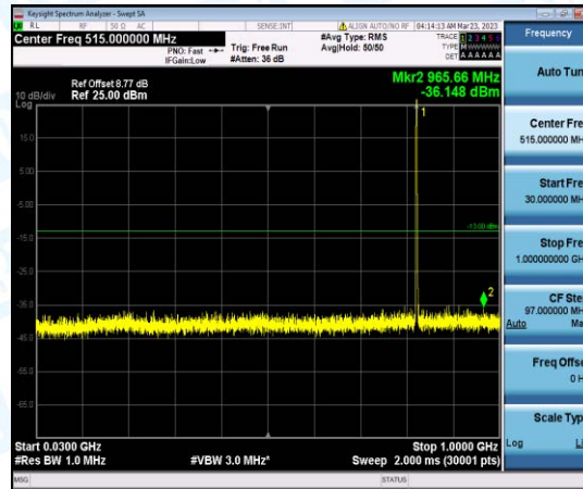
Band26-15MHz-16QAM-26865-1-0-Low-30-1000--36.15-PASS
