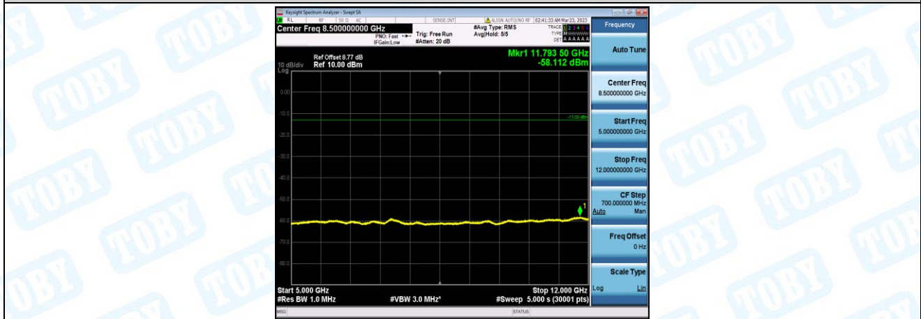
Band26-3MHz-16QAM-26805-1-0-Low-5000-12000--58.11-PASS
