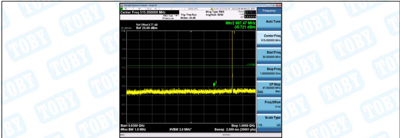
Band26-5MHz-16QAM-26815-1-0-Low-30-1000--35.72-PASS
