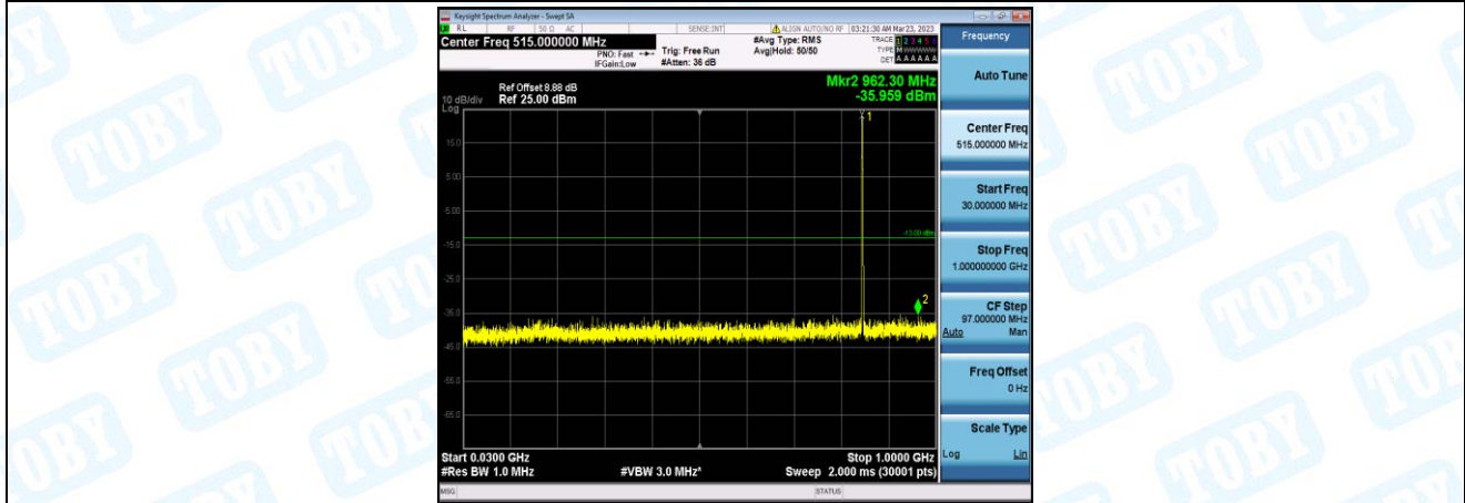
Band26-5MHz-16QAM-27015-1-0-High-30-1000--35.96-PASS
