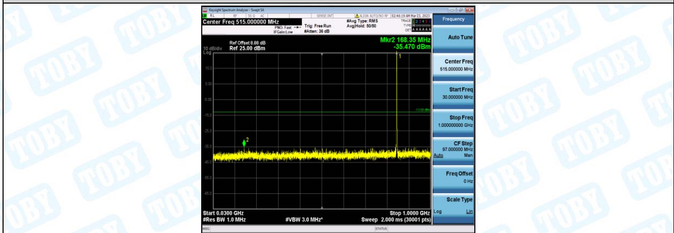
Band26-3MHz-QPSK-27025-1-0-High-30-1000--35.47-PASS
