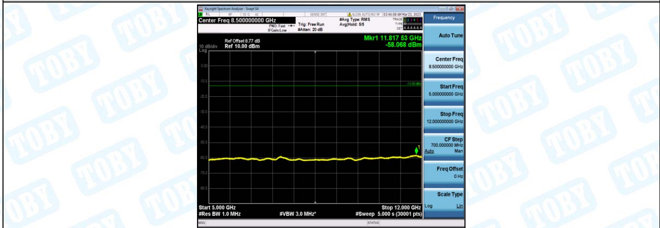
Band26-10MHz-16QAM-26840-1-0-Low-5000-12000--58.07-PASS
