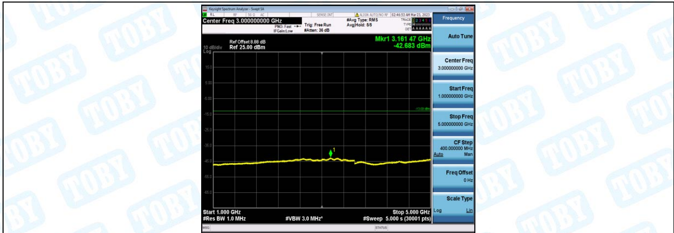
Band26-3MHz-QPSK-27025-1-0-High-1000-5000--42.68-PASS
