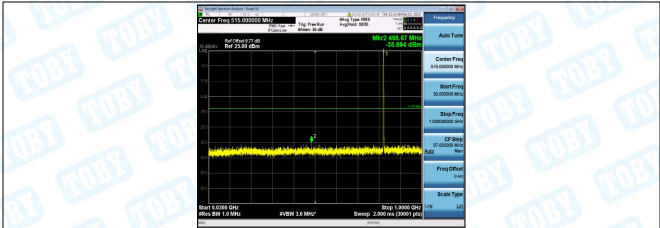
Band26-15MHz-QPSK-26865-1-0-Low-30-1000--35.69-PASS
