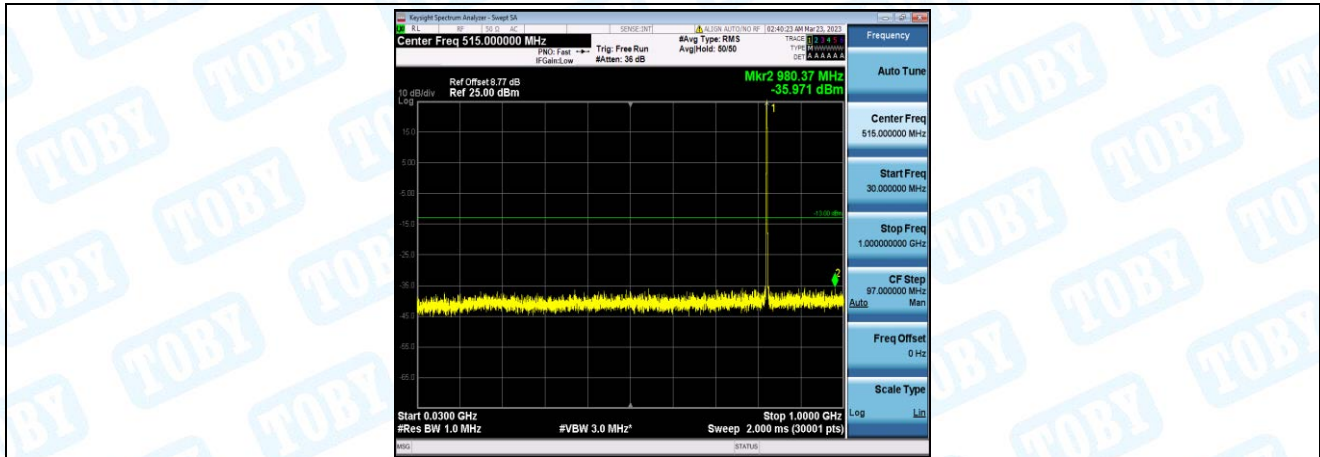
Band26-3MHz-16QAM-26805-1-0-Low-30-1000--35.97-PASS
