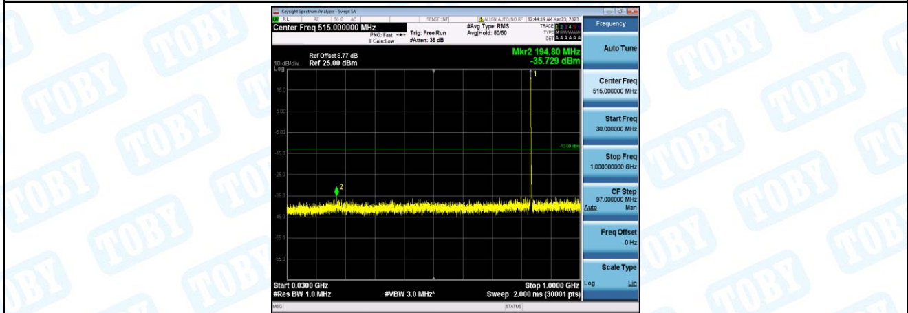
Band26-3MHz-16QAM-26915-1-0-Low-30-1000--35.73-PASS
