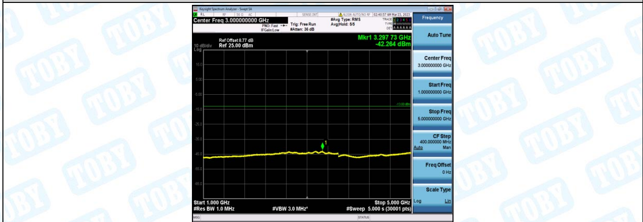
Band26-3MHz-16QAM-26805-1-0-Low-1000-5000--42.26-PASS
