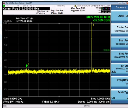
Band26-5MHz-QPSK-26815-1-0-Low-30-1000--35.56-PASS
