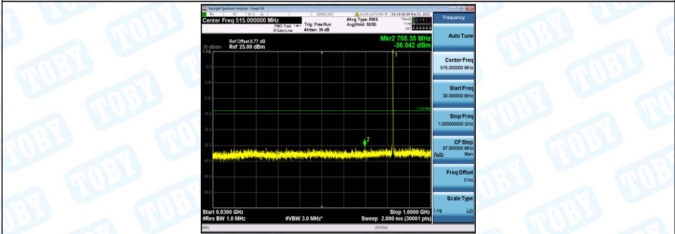
Band26-15MHz-16QAM-26915-1-0-Low-30-1000--36.04-PASS
