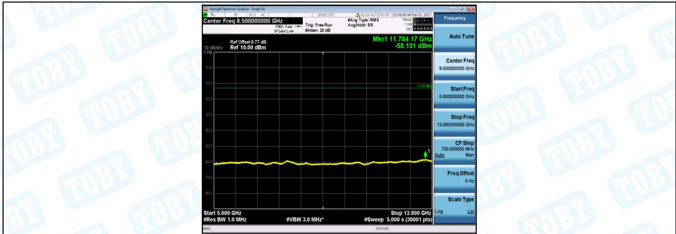
Band26-10MHz-QPSK-26915-1-0-Low-5000-12000--58.13-PASS
