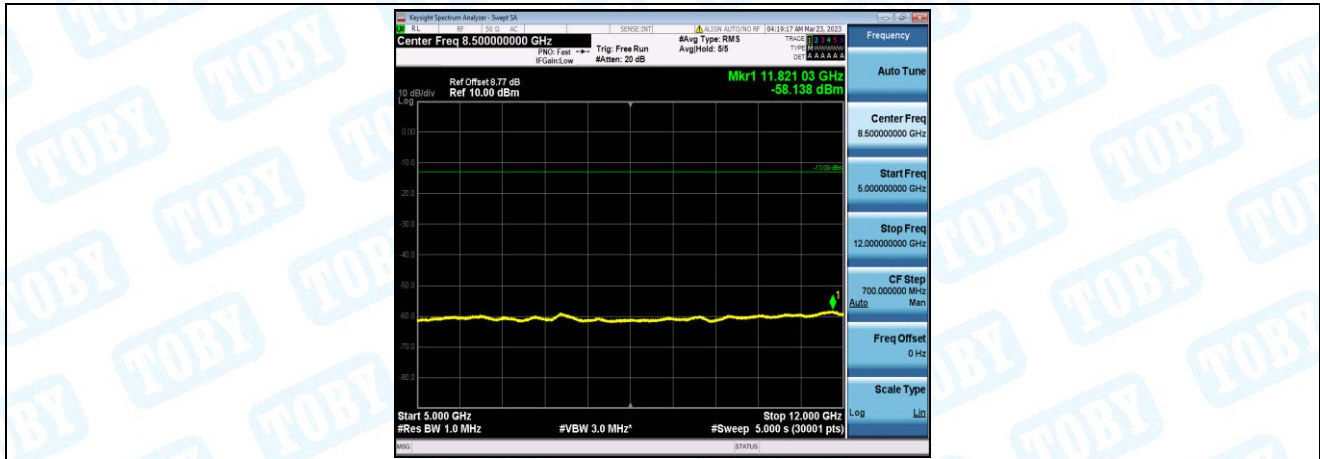
Band26-15MHz-16QAM-26915-1-0-Low-5000-12000--58.14-PASS
