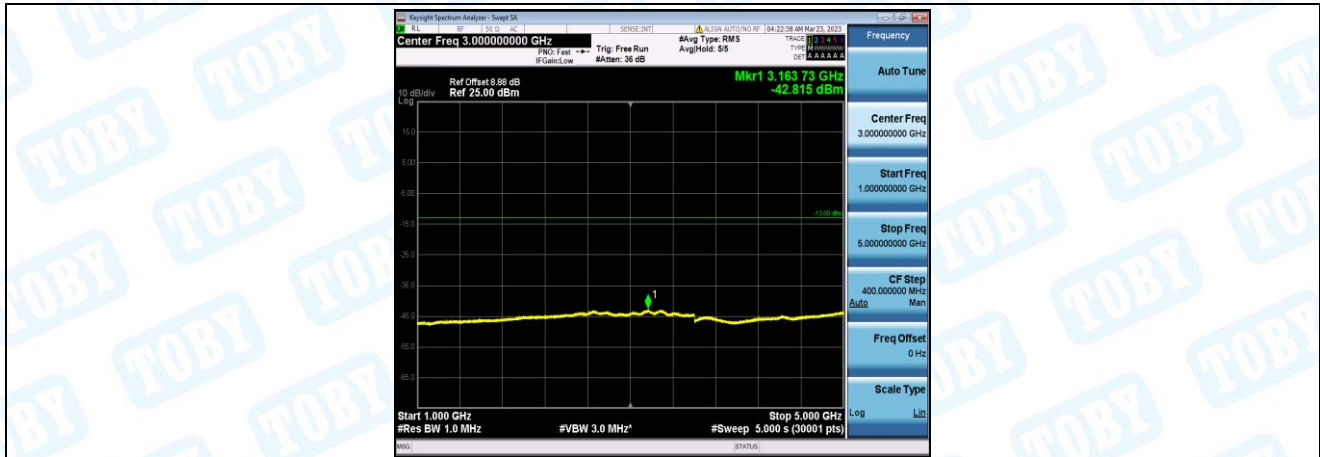
Band26-15MHz-16QAM-26965-1-0-High-1000-5000--42.82-PASS
