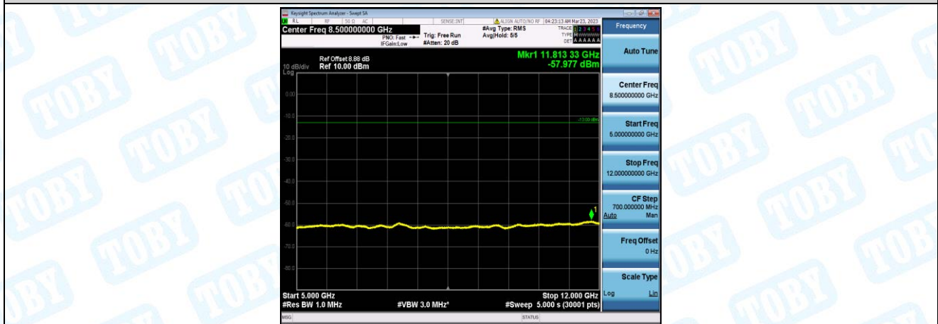
Band26-15MHz-16QAM-26965-1-0-High-5000-12000--57.98-PASS
