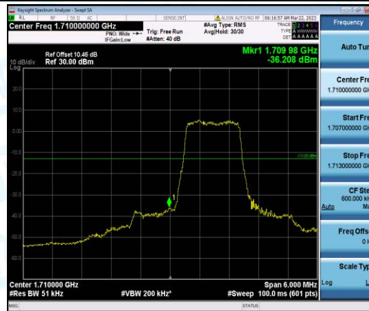
Band4-3MHz-16QAM-19965-6-0-Low--36.21-PASS
