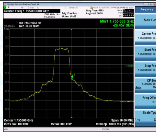
Band4-5MHz-QPSK-20375-6-0-High--26.46-PASS
