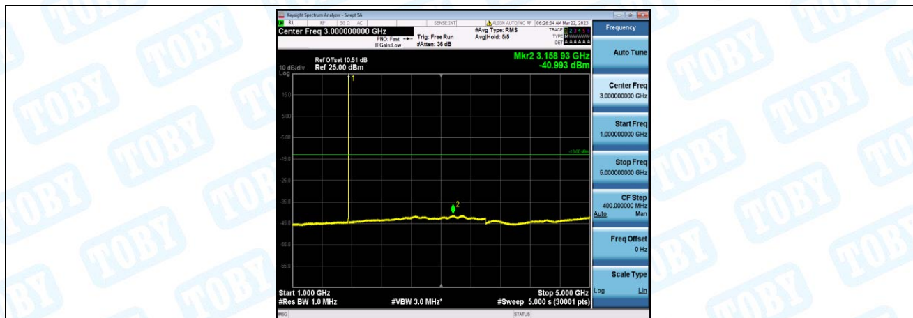
Band4-3MHz-QPSK-20385-1-0-High-1000-5000--40.99-PASS
