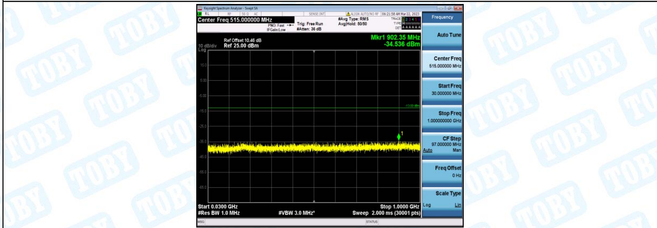
Band4-3MHz-QPSK-20175-1-0-Low-30-1000--34.54-PASS
