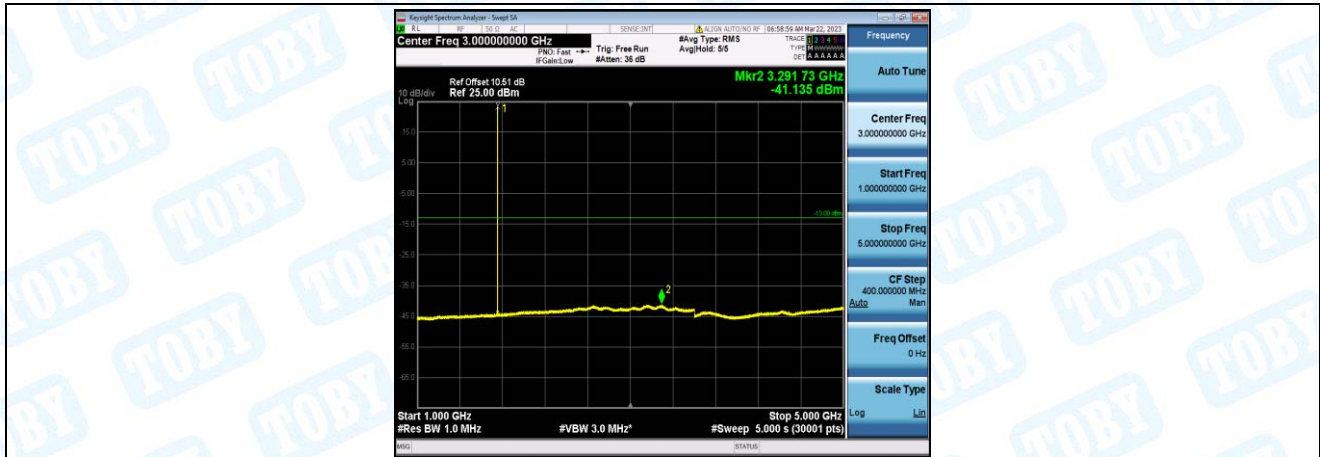
Band4-5MHz-16QAM-20375-1-0-High-1000-5000--41.14-PASS
