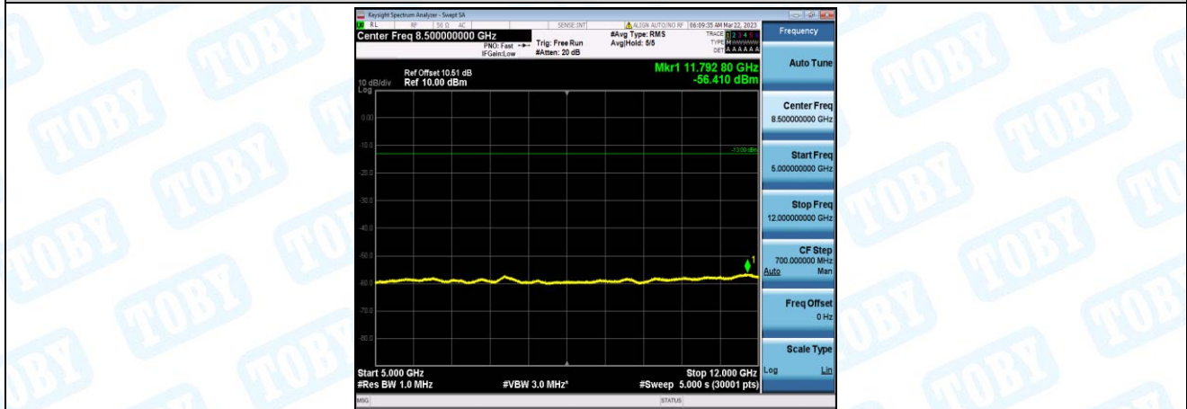
Band4-1.4MHz-16QAM-20393-1-0-High-5000-12000--56.41-PASS
