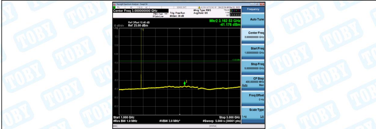
Band4-3MHz-QPSK-20175-1-0-Low-1000-5000--41.18-PASS
