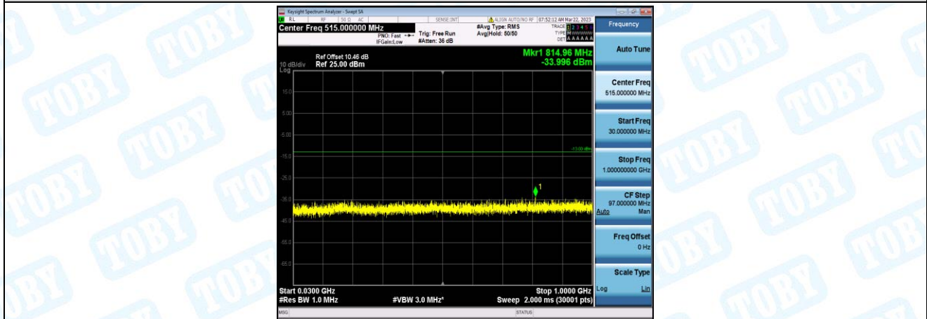
Band4-15MHz-QPSK-20175-1-0-Low-30-1000--34-PASS
