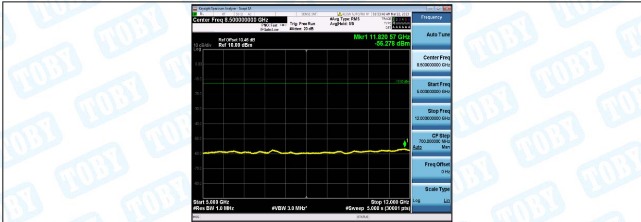
Band4-5MHz-QPSK-20175-1-0-Low-5000-12000--56.28-PASS
