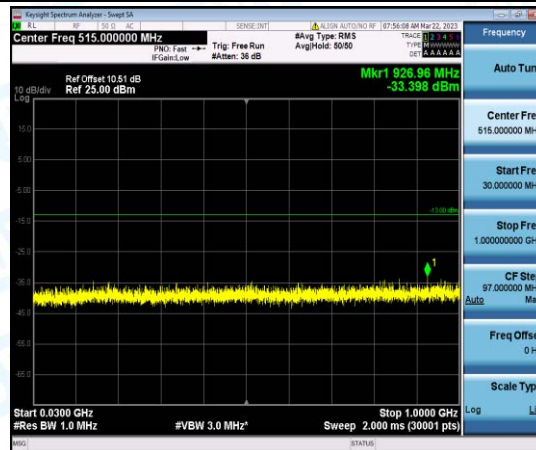
Band4-15MHz-QPSK-20325-1-0-High-30-1000--33.4-PASS
