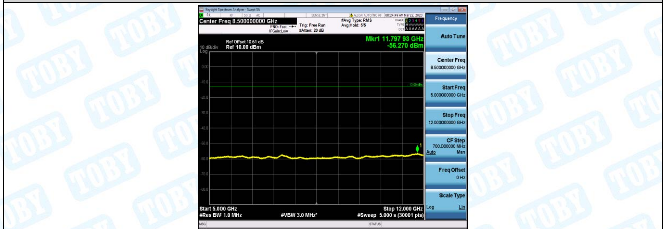
Band4-20MHz-QPSK-20300-1-0-High-5000-12000--56.27-PASS
