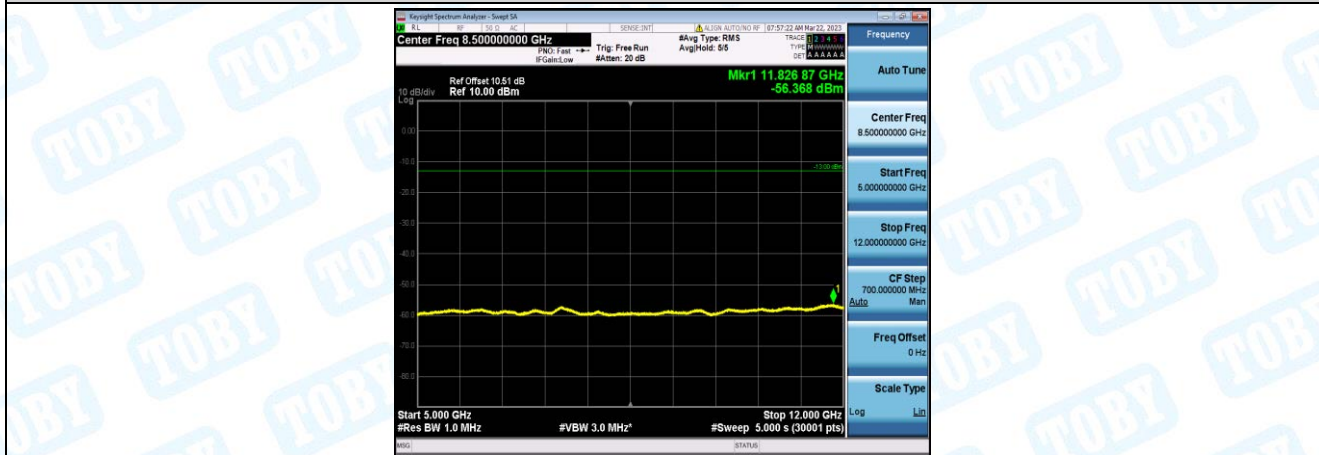
Band4-15MHz-QPSK-20325-1-0-High-5000-12000--56.37-PASS
