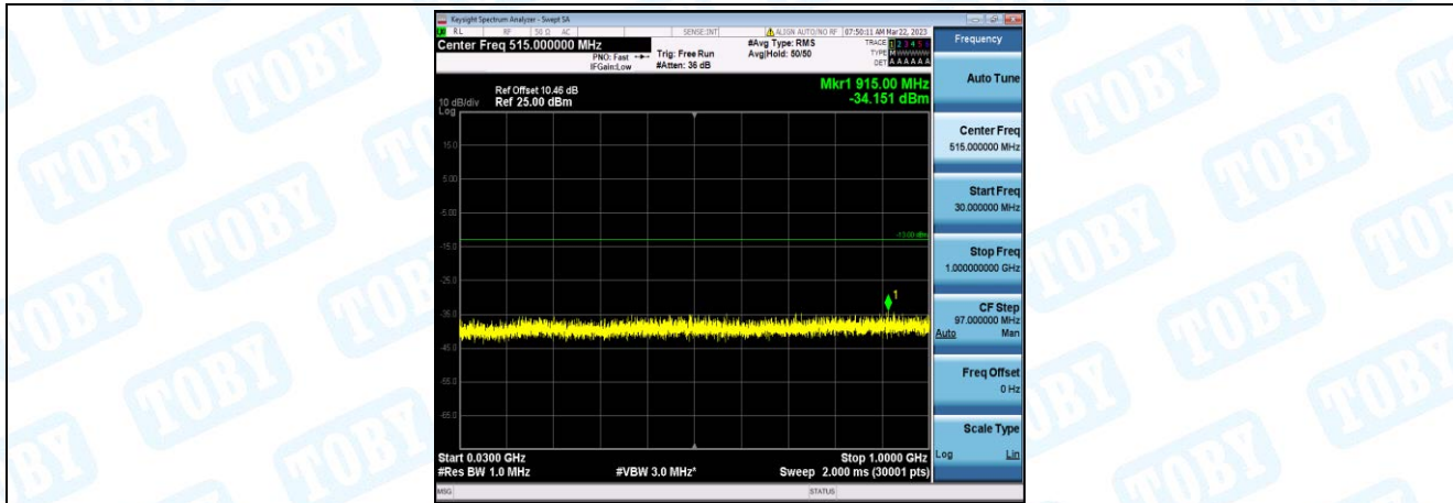
Band4-15MHz-16QAM-20025-1-0-Low-30-1000--34.15-PASS
