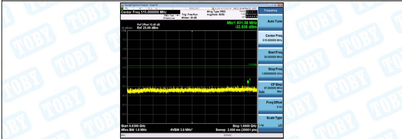
Band4-20MHz-16QAM-20175-1-0-Low-30-1000--32.94-PASS
