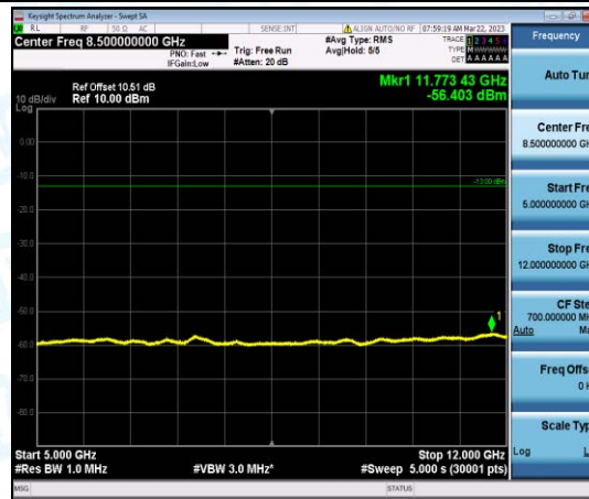
Band4-15MHz-16QAM-20325-1-0-High-5000-12000--56.4-PASS
