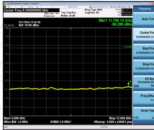
Band4-20MHz-QPSK-20175-1-0-Low-5000-12000--56.29-PASS
