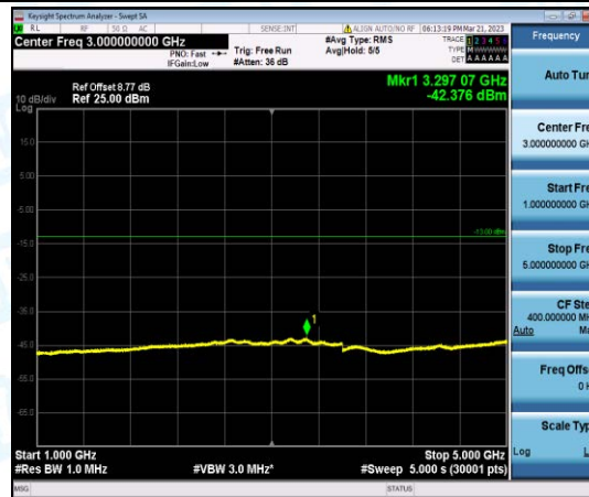
Band5-1.4MHz-16QAM-20407-1-0-Low-1000-5000--42.38-PASS
