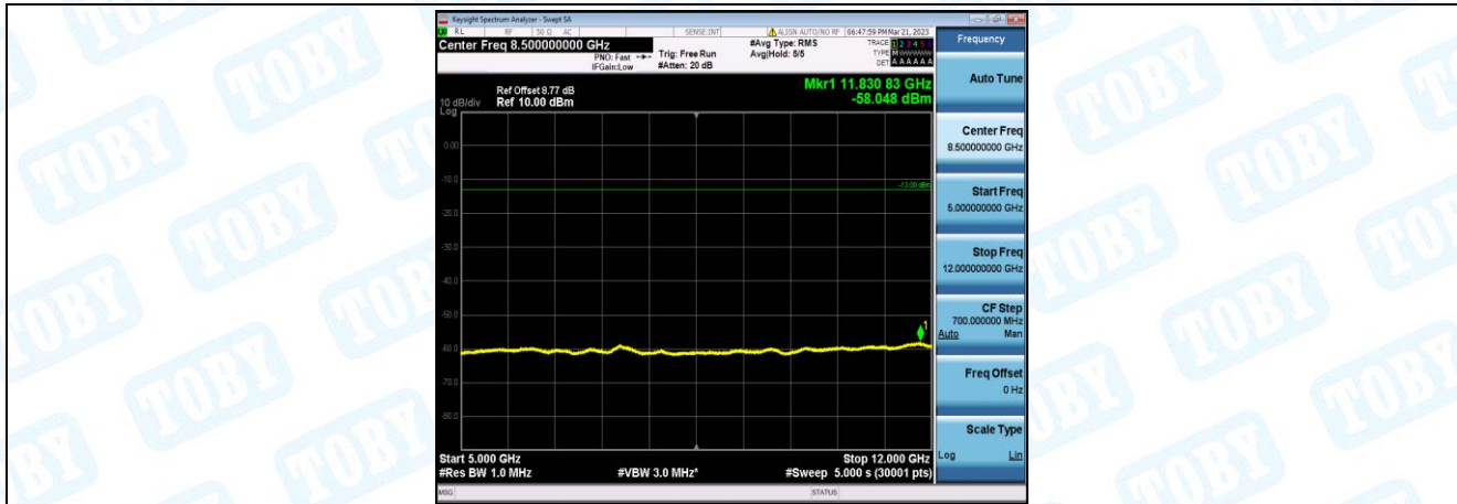
Band5-3MHz-QPSK-20525-1-0-Low-5000-12000--58.05-PASS
