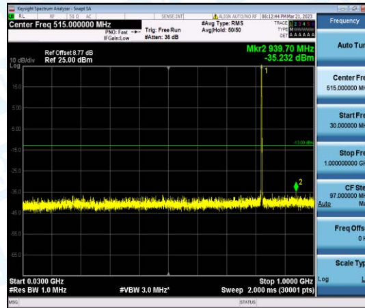
Band5-1.4MHz-16QAM-20407-1-0-Low-30-1000--35.23-PASS
