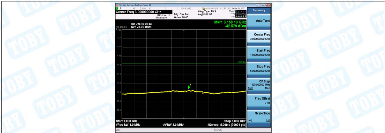
Band5-5MHz-QPSK-20625-1-0-High-1000-5000--42.58-PASS
